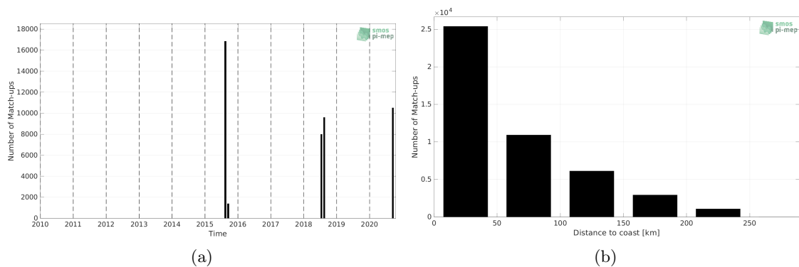
Figure 1: Number of match-ups between TSG (SAMOS) and SMAP SSS L3 v5.0 - 8-Day running (JPL) SSS as a function of time (a) and as function of the distance to coast (b) over the Arctic Ocean Pi-MEP region and for the full satellite product period.
