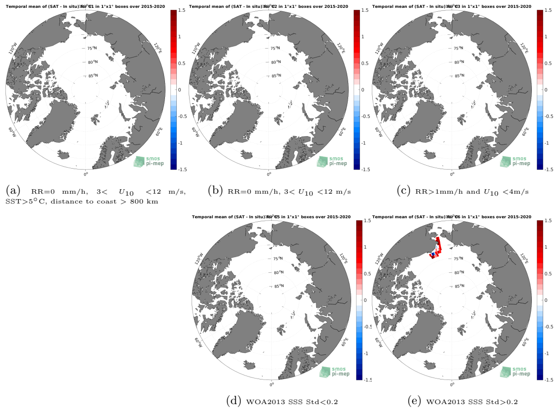
Figure 12: Temporal mean gridded over spatial boxes of size 1^{\circ}\times 1^{\circ} of \Delta\text{SSS} (SMAP SSS L3 v5.0 - 8-Day running (JPL) - TSG (SAMOS)) for 5 different subdatasets corresponding to:RR=0 mm/h, 3 < U_{10} < 12 m/s, SST > 5^{\circ}\text{C} , distance to coast > 800 km (a), RR=0 mm/h, 3 < U_{10} < 12 m/s (b), RR > 1 mm/h and U_{10} < 4 m/s (c), WOA2013 SSS Std < 0.2 (d), WOA2013 SSS Std > 0.2 (e).
