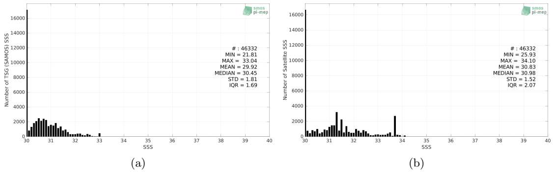
Figure 2: Histograms of SSS from TSG (SAMOS) (a) and SMAP SSS L3 v5.0 - 8-Day running (JPL) (b) considering all match-up pairs per bins of 0.1 over the Arctic Ocean Pi-MEP region and for the full satellite product period.
