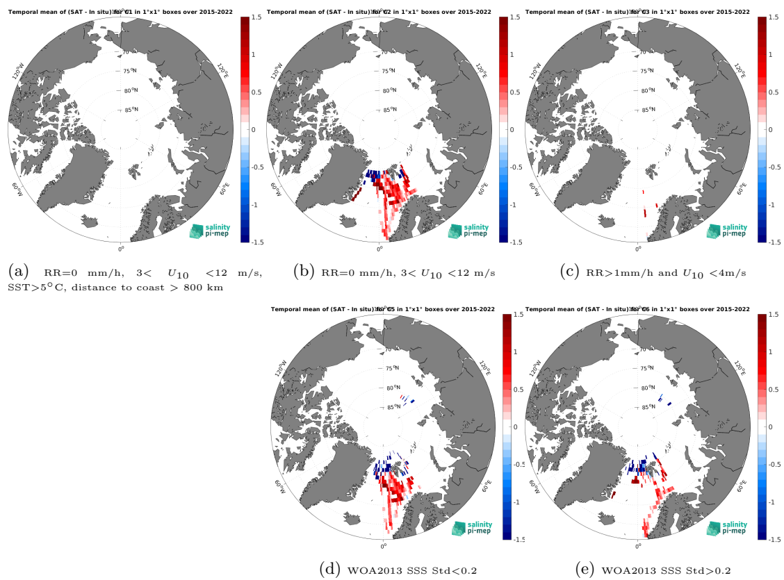
Figure 14: Temporal mean gridded over spatial boxes of size 1^\circ \times 1^\circ of \Delta\text{SSS} (SMAP SSS L3 v5.0 - 8-Day running (JPL) - TSG (Polarstern)) for 5 different subdatasets corresponding to:RR=0 mm/h, 3 < U_{10} < 12 m/s, SST > 5°C, distance to coast > 800 km (a), RR=0 mm/h, 3 < U_{10} < 12 m/s (b), RR > 1mm/h and U_{10} < 4 m/s (c), WOA2013 SSS Std < 0.2 (d), WOA2013 SSS Std > 0.2 (e).
