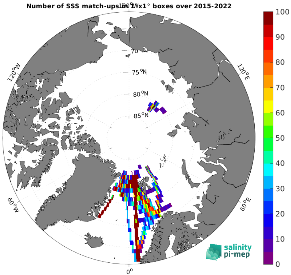
Figure 5: Number of SSS match-ups between TSG (Polarstern) SSS and the SMAP SSS L3 v5.0 - 8-Day running (JPL) SSS product for the Arctic Ocean Pi-MEP region over 1^\circ \times 1^\circ boxes and for the full satellite product period.
