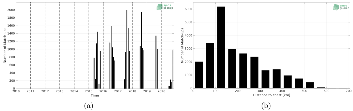
Figure 1: Number of match-ups between TSG (Polarstern) and SMAP SSS L3 v5.0 - 8-Day running (JPL) SSS as a function of time (a) and as function of the distance to coast (b) over the Arctic Ocean Pi-MEP region and for the full satellite product period.
