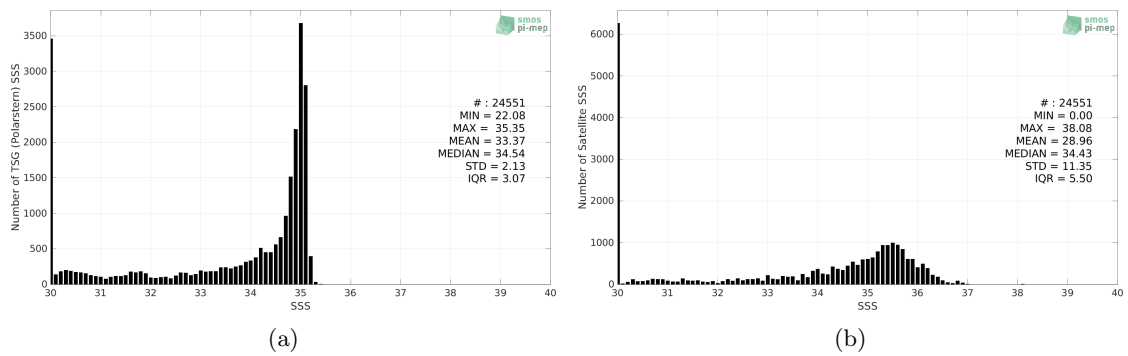
Figure 2: Histograms of SSS from TSG (Polarstern) (a) and SMAP SSS L3 v5.0 - 8-Day running (JPL) (b) considering all match-up pairs per bins of 0.1 over the Arctic Ocean Pi-MEP region and for the full satellite product period.
