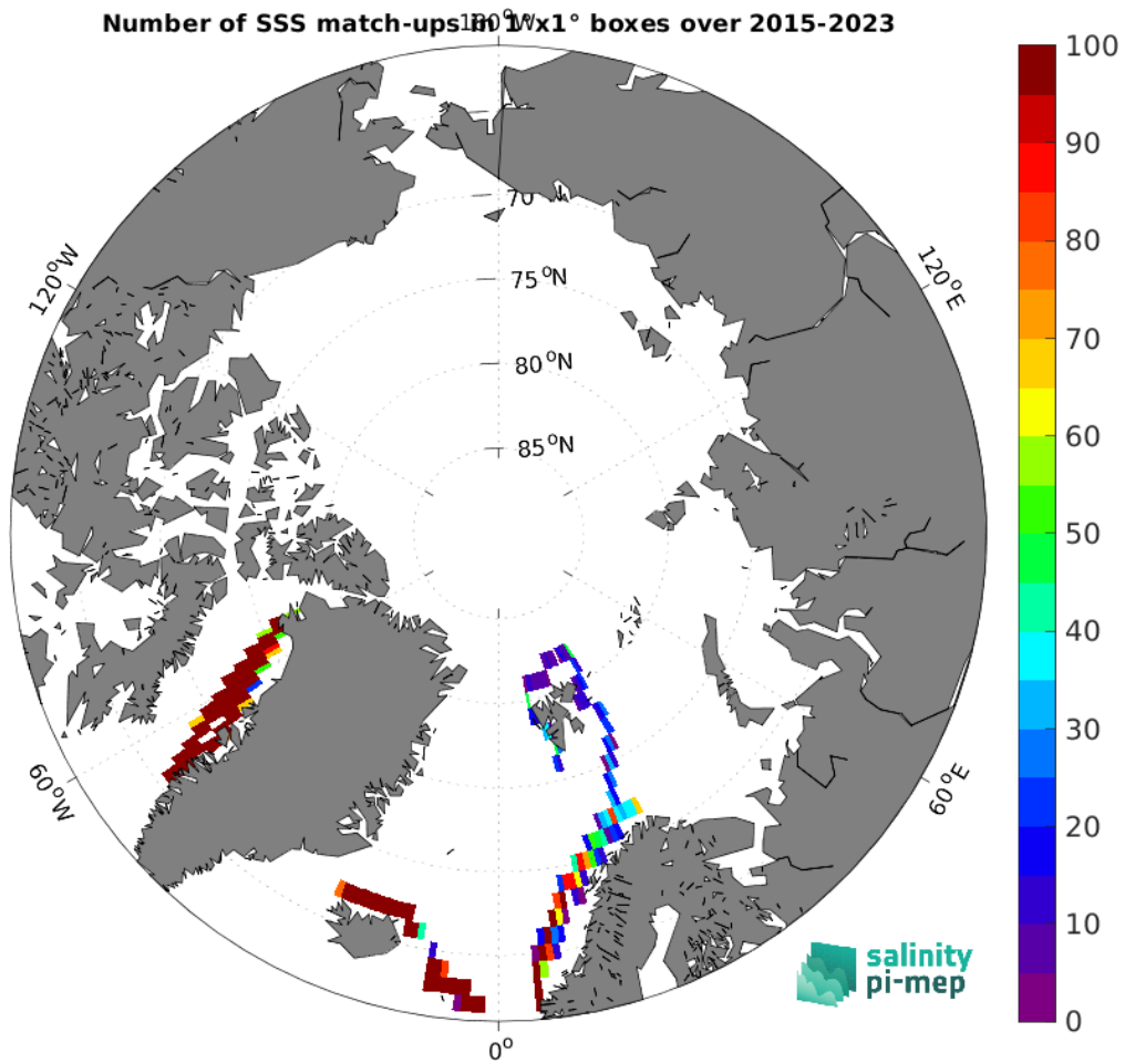
Figure 5: Number of SSS match-ups between TSG (LEGOS-DM) SSS and the SMAP SSS L3 v5.0 - 8-Day running (JPL) SSS product for the Arctic Ocean Pi-MEP region over 1^\circ \times 1^\circ boxes and for the full satellite product period.
