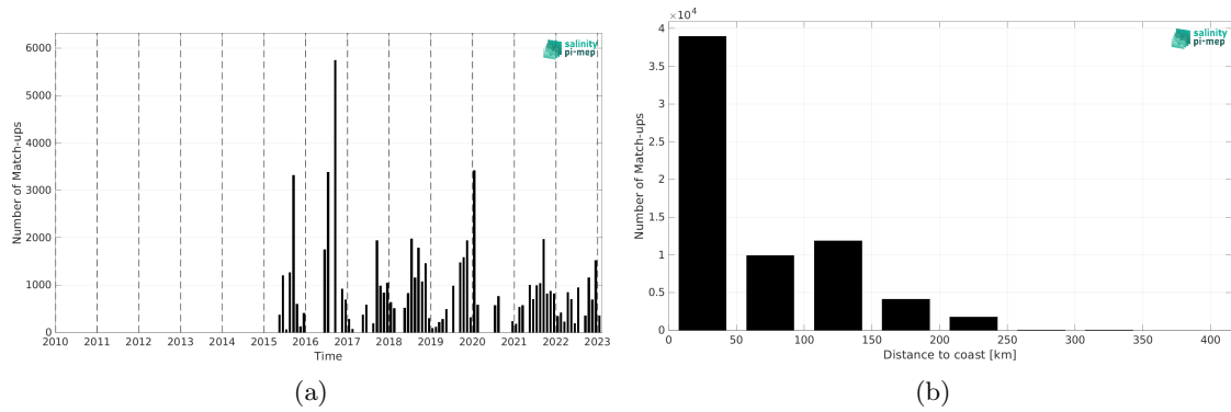
Figure 2: Number of match-ups between TSG (LEGOS-DM) and SMAP SSS L3 v5.0 - 8-Day running (JPL) SSS as a function of time (a) and as function of the distance to coast (b) over the Arctic Ocean Pi-MEP region and for the full satellite product period.
