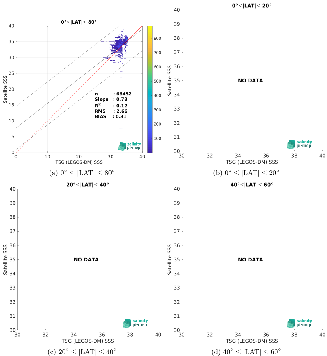
Figure 10: Contour maps of the concentration of SMAP SSS L3 v5.0 - 8-Day running (JPL) SSS (y-axis) versus TSG (LEGOS-DM) SSS (x-axis) at match-up pairs for different latitude bands. For each plot, the red line shows x=y . The black thin and dashed lines indicate a linear fit through the data cloud and the \pm 95\% confidence levels, respectively. The number match-up pairs n , the slope and R^2 coefficient of the linear fit, the root mean square (RMS) and the mean bias between satellite and in situ data are indicated for each latitude band in each plot.
