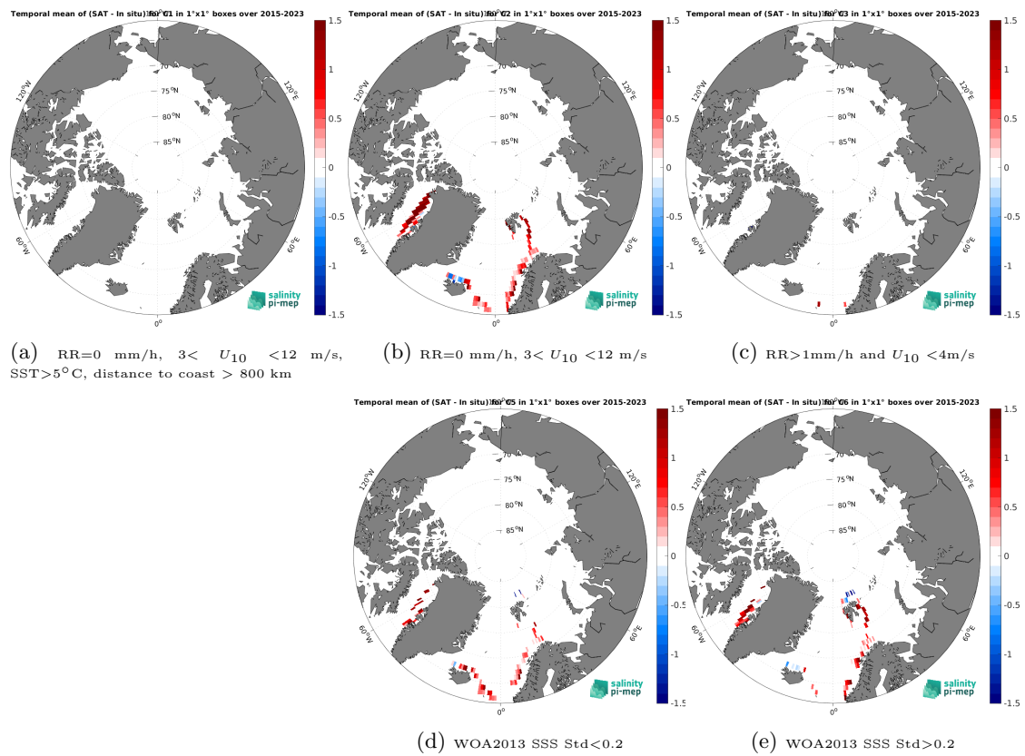
Figure 14: Temporal mean gridded over spatial boxes of size 1^\circ \times 1^\circ of \Delta\text{SSS} (SMAP SSS L3 v5.0 - 8-Day running (JPL) - TSG (LEGOS-DM)) for 5 different subdatasets corresponding to: RR=0 mm/h, 3 < U_{10} < 12 m/s, SST > 5°C, distance to coast > 800 km (a), RR=0 mm/h, 3 < U_{10} < 12 m/s (b), RR > 1mm/h and U_{10} < 4 m/s (c), WOA2013 SSS Std < 0.2 (d), WOA2013 SSS Std > 0.2 (e).
