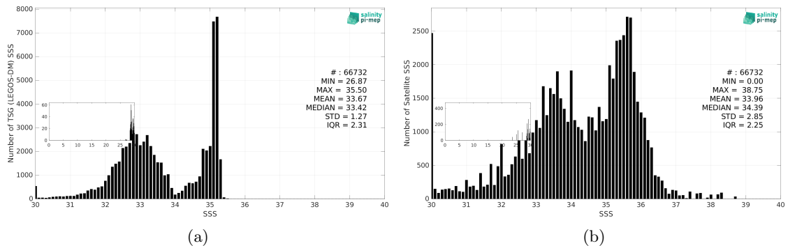
Figure 3: Histograms of SSS from TSG (LEGOS-DM) (a) and SMAP SSS L3 v5.0 - 8-Day running (JPL) (b) considering all match-up pairs per bins of 0.1 over the Arctic Ocean Pi-MEP region and for the full satellite product period.
