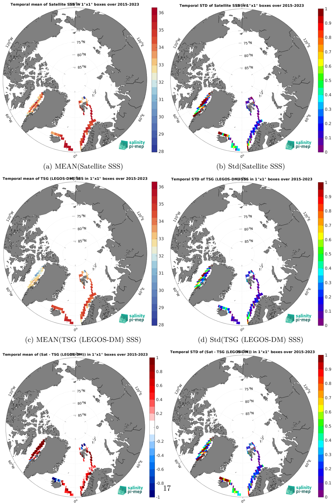
Figure 7: Temporal mean (left) and Std (right) of SSS from SMAP SSS L3 v5.0 - 8-Day running (JPL) (top), TSG (LEGOS-DM) (middle), and of \Delta SSS (Satellite - TSG (LEGOS-DM)). Only match-up pairs are used to generate these maps.
