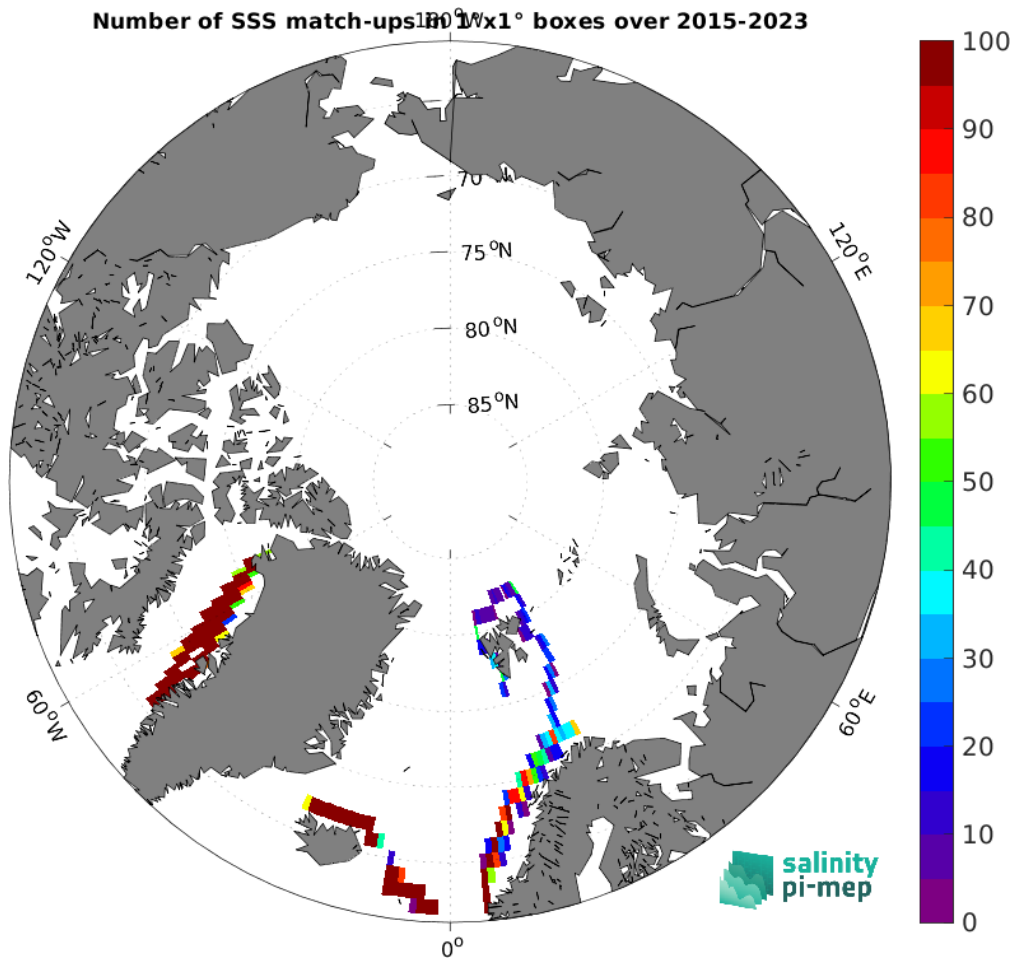
Figure 4: Number of SSS match-ups between TSG (LEGOS-DM) SSS and the SMAP SSS L3 v5.0 - 8-Day running (JPL) SSS product for the Arctic Ocean Pi-MEP region over 1^{\circ} \times 1^{\circ} boxes and for the full satellite product period.
