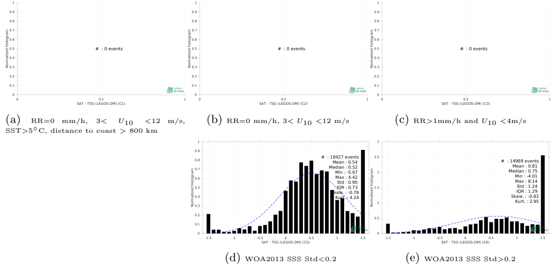
Figure 13: Normalized histogram of \Delta SSS (SMAP SSS L3 v5.0 - 8-Day running (JPL) - TSG (LEGOS-DM)) for 5 different subdatasets corresponding to: RR=0 mm/h, 3 < U_{10} < 12 m/s, SST >5^{\circ} C, distance to coast > 800 km (a), RR=0 mm/h, 3 < U_{10} < 12 m/s (b), RR >1 mm/h and U_{10} < 4 m/s (c), WOA2013 SSS Std <0.2 (d), WOA2013 SSS Std >0.2 (e).
