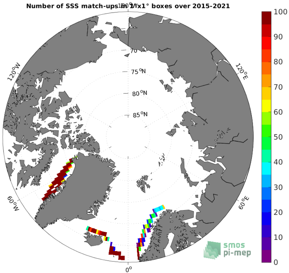
Figure 4: Number of SSS match-ups between TSG (LEGOS-DM) SSS and the SMAP SSS L3 v5.0 - 8-Day running (JPL) SSS product for the Arctic Ocean Pi-MEP region over 1°×1° boxes and for the full satellite product period.
