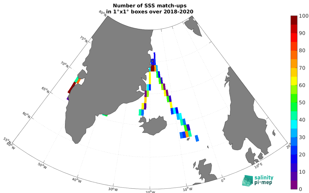
Figure 4: Number of SSS match-ups between TSG (Lauge-Koch) SSS and the SMAP SSS L3 v5.0 - 8-Day running (JPL) SSS product for the Arctic Ocean Pi-MEP region over 1^\circ \times 1^\circ boxes and for the full satellite product period.
