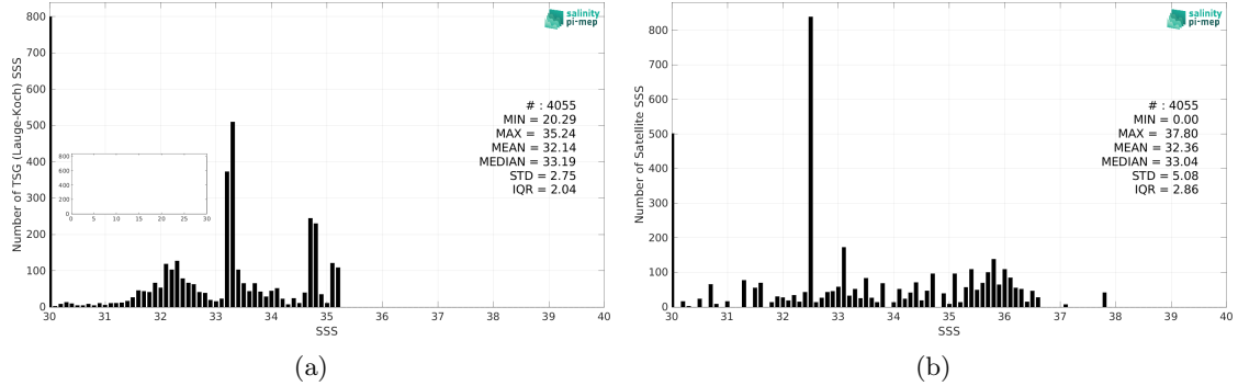
Figure 2: Histograms of SSS from TSG (Lauge-Koch) (a) and SMAP SSS L3 v5.0 - 8-Day running (JPL) (b) considering all match-up pairs per bins of 0.1 over the Arctic Ocean Pi-MEP region and for the full satellite product period.
