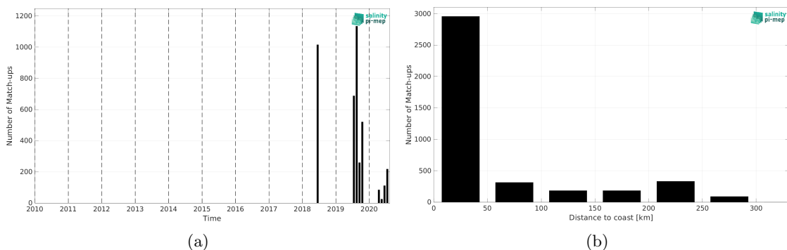
Figure 1: Number of match-ups between TSG (Lauge-Koch) and SMAP SSS L3 v5.0 - 8-Day running (JPL) SSS as a function of time (a) and as function of the distance to coast (b) over the Arctic Ocean Pi-MEP region and for the full satellite product period.
