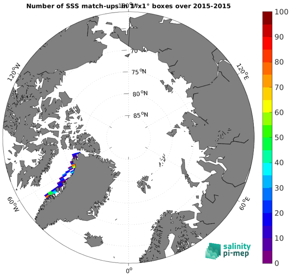
Figure 5: Number of SSS match-ups between TSG (GOSUD-Sailing-ship) SSS and the SMAP SSS L3 v5.0 - 8-Day running (JPL) SSS product for the Arctic Ocean Pi-MEP region over 1^\circ \times 1^\circ boxes and for the full satellite product period.
