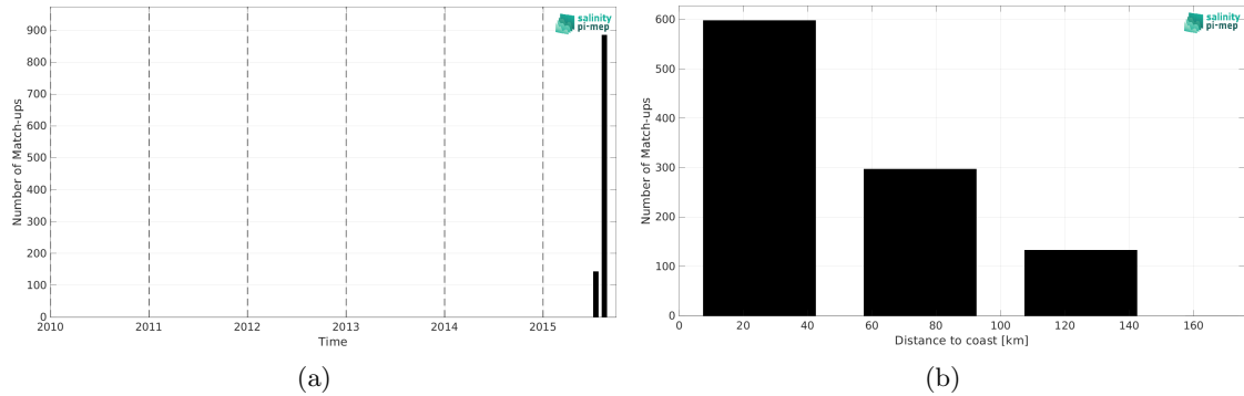
Figure 2: Number of match-ups between TSG (GOSUD-Sailing-ship) and SMAP SSS L3 v5.0 - 8-Day running (JPL) SSS as a function of time (a) and as function of the distance to coast (b) over the Arctic Ocean Pi-MEP region and for the full satellite product period.
