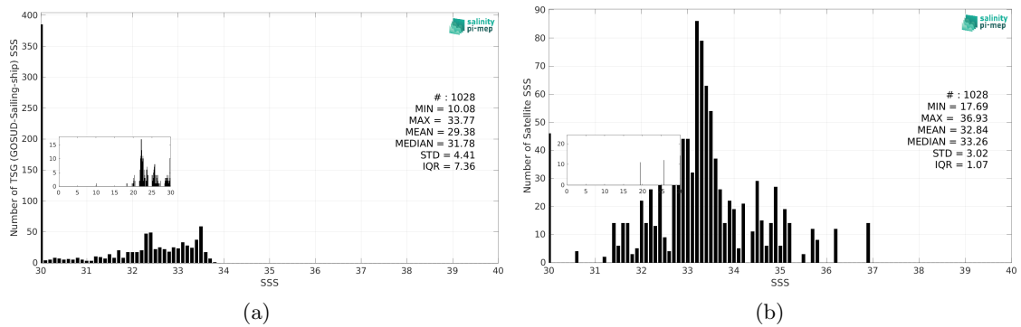
Figure 3: Histograms of SSS from TSG (GOSUD-Sailing-ship) (a) and SMAP SSS L3 v5.0 - 8-Day running (JPL) (b) considering all match-up pairs per bins of 0.1 over the Arctic Ocean Pi-MEP region and for the full satellite product period.
