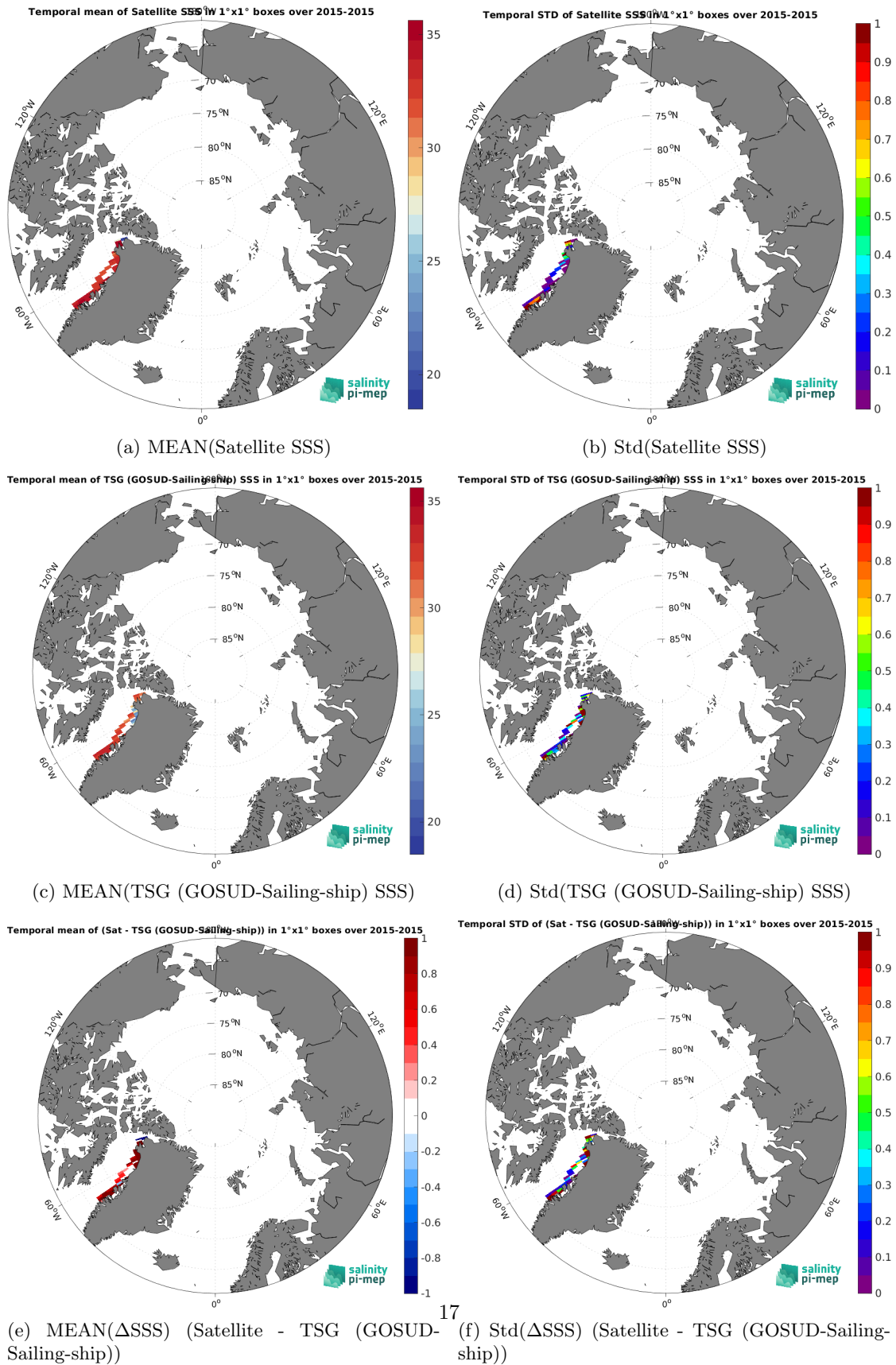
Figure 7: Temporal mean (left) and Std (right) of SSS from SMAP SSS L3 v5.0 - 8-Day running (JPL) (top), TSG (GOSUD-Sailing-ship) (middle), and of \Delta SSS (Satellite - TSG (GOSUD-Sailing-ship)). Only match-up pairs are used to generate these maps.
