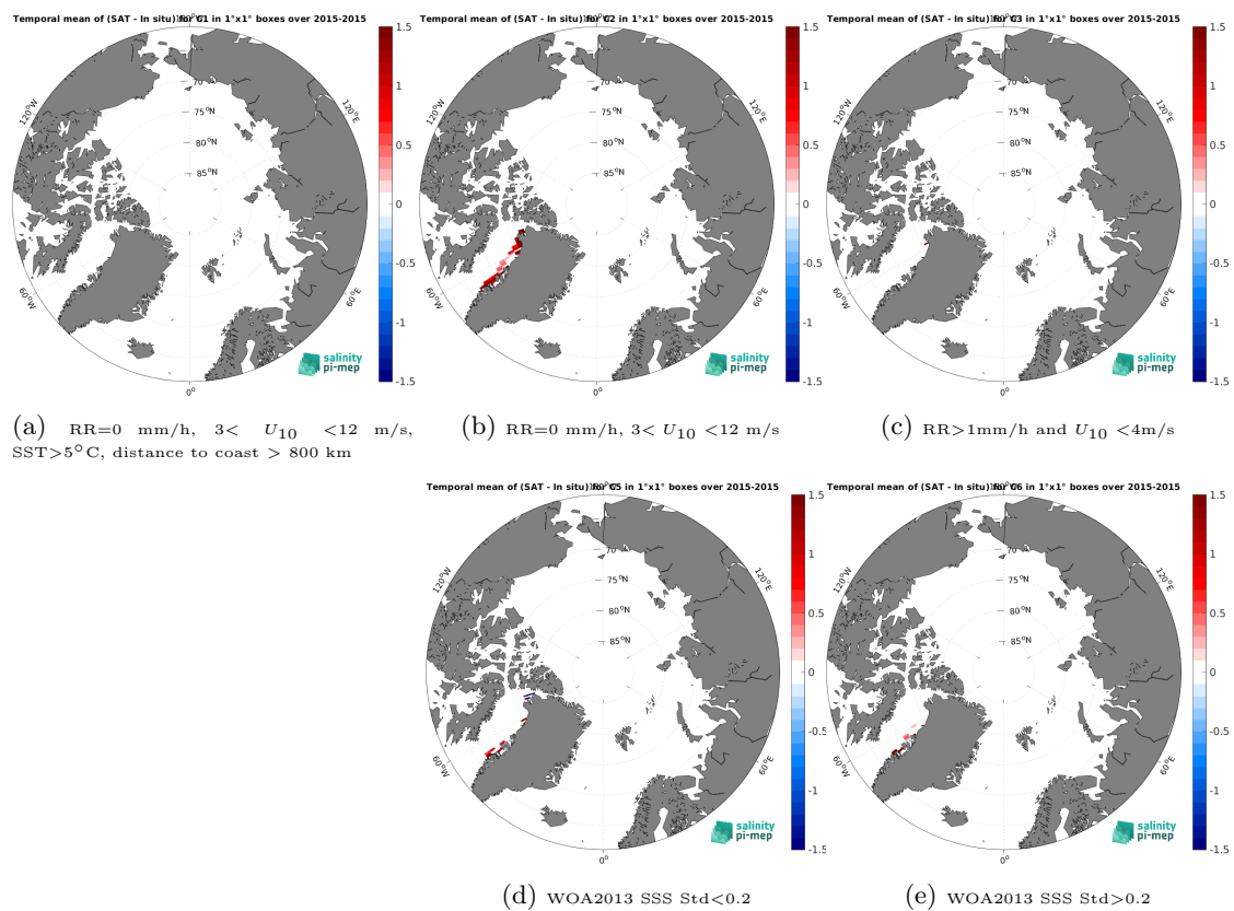
Figure 14: Temporal mean gridded over spatial boxes of size 1^\circ \times 1^\circ of \Delta\text{SSS} (SMAP SSS L3 v5.0 - 8-Day running (JPL) - TSG (GOSUD-Sailing-ship)) for 5 different subdatasets corresponding to: RR=0 mm/h, 3 < U_{10} < 12 m/s, SST > 5°C, distance to coast > 800 km (a), RR=0 mm/h, 3 < U_{10} < 12 m/s (b), RR > 1mm/h and U_{10} < 4 m/s (c), WOA2013 SSS Std < 0.2 (d), WOA2013 SSS Std > 0.2 (e).
