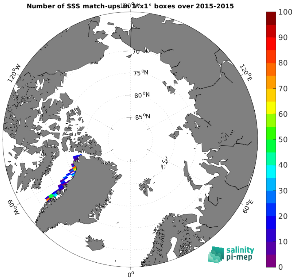
Figure 4: Number of SSS match-ups between TSG (GOSUD-Sailing-ship) SSS and the SMAP SSS L3 v5.0 - 8-Day running (JPL) SSS product for the Arctic Ocean Pi-MEP region over 1^\circ \times 1^\circ boxes and for the full satellite product period.
