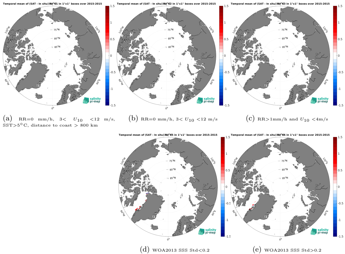
Figure 12: Temporal mean gridded over spatial boxes of size 1^{\circ} \times 1^{\circ} of \Delta SSS (SMAP SSS L3 v5.0 - 8-Day running (JPL) - TSG (GOSUD-Sailing-ship)) for 5 different subdatasets corresponding to: RR=0 mm/h, 3 < U_{10} < 12 m/s, SST > 5^{\circ}C , distance to coast > 800 km (a), RR=0 mm/h, 3 < U_{10} < 12 m/s (b), RR > 1 mm/h and U_{10} < 4 m/s (c), WOA2013 SSS Std < 0.2 (d), WOA2013 SSS Std > 0.2 (e).
