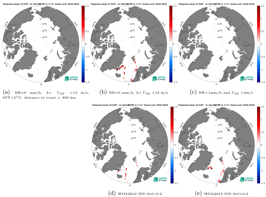
Figure 14: Temporal mean gridded over spatial boxes of size 1^\circ \times 1^\circ of \Delta\text{SSS} (SMAP SSS L3 v5.0 - 8-Day running (JPL) - TSG (GOSUD-Research-vessel)) for 5 different subdatasets corresponding to: RR=0 mm/h, 3 < U_{10} < 12 m/s, SST > 5°C, distance to coast > 800 km (a), RR=0 mm/h, 3 < U_{10} < 12 m/s (b), RR > 1mm/h and U_{10} < 4 m/s (c), WOA2013 SSS Std < 0.2 (d), WOA2013 SSS Std > 0.2 (e).
