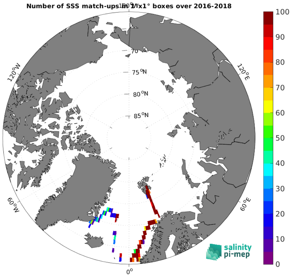
Figure 4: Number of SSS match-ups between TSG (GOSUD-Research-vessel) SSS and the SMAP SSS L3 v5.0 - 8-Day running (JPL) SSS product for the Arctic Ocean Pi-MEP region over 1^\circ \times 1^\circ boxes and for the full satellite product period.
