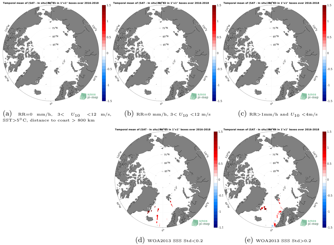
Figure 12: Temporal mean gridded over spatial boxes of size 1^\circ \times 1^\circ of \Delta SSS (SMAP SSS L3 v5.0 - 8-Day running (JPL) - TSG (GOSUD-Research-vessel)) for 5 different subdatasets corresponding to: RR=0 mm/h, 3 < U_{10} < 12 m/s, SST > 5^\circ\text{C} , distance to coast > 800 km (a), RR=0 mm/h, 3 < U_{10} < 12 m/s (b), RR > 1 mm/h and U_{10} < 4 m/s (c), WOA2013 SSS Std < 0.2 (d), WOA2013 SSS Std > 0.2 (e).
