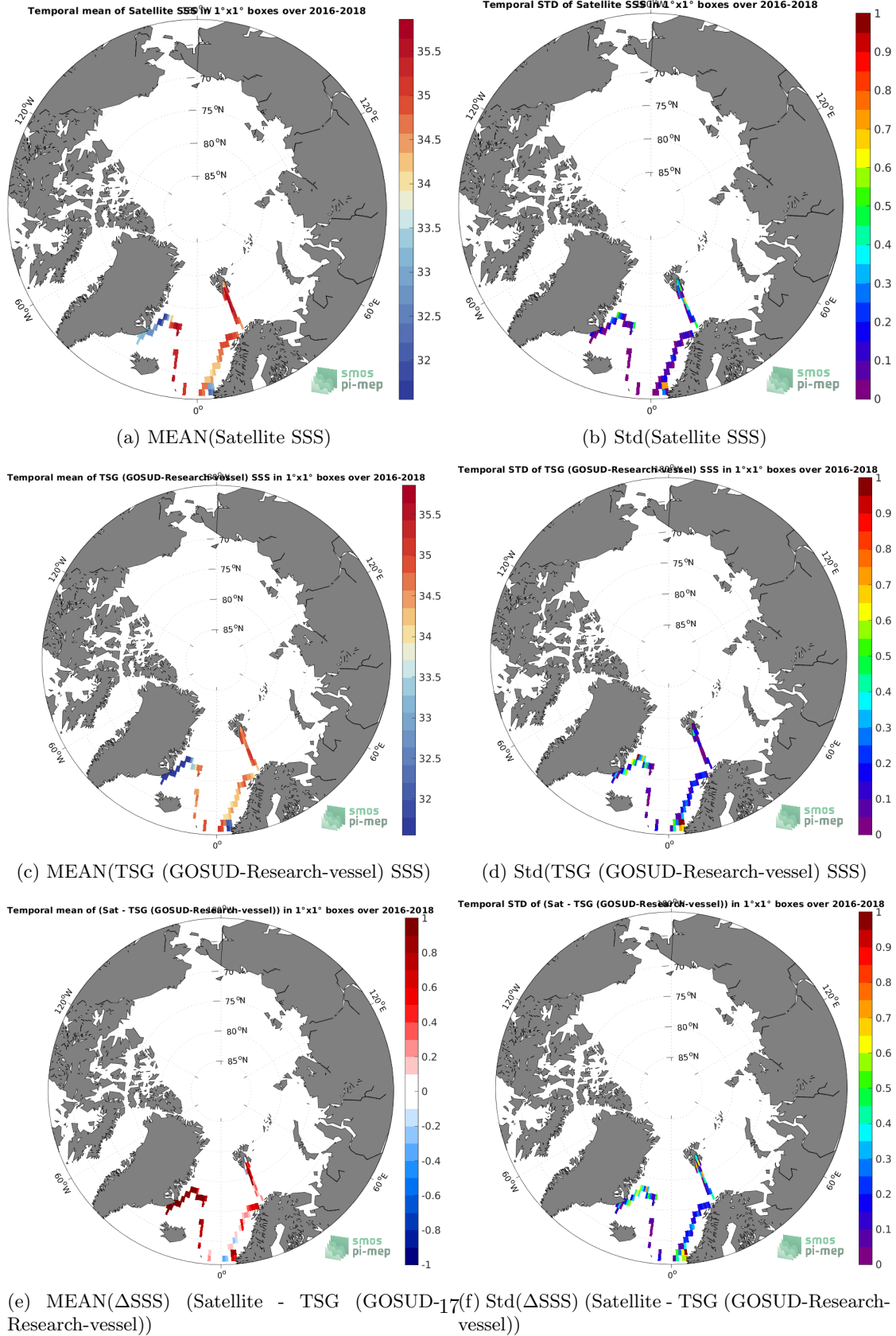
Figure 6: Temporal mean (left) and Std (right) of SSS from SMAP SSS L3 v5.0 - 8-Day running (JPL) (top), TSG (GOSUD-Research-vessel) (middle), and of \Delta SSS (Satellite - TSG (GOSUD-Research-vessel)). Only match-up pairs are used to generate these maps.
