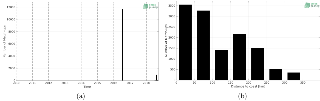
Figure 1: Number of match-ups between TSG (GOSUD-Research-vessel) and SMAP SSS L3 v5.0 - 8-Day running (JPL) SSS as a function of time (a) and as function of the distance to coast (b) over the Arctic Ocean Pi-MEP region and for the full satellite product period.
