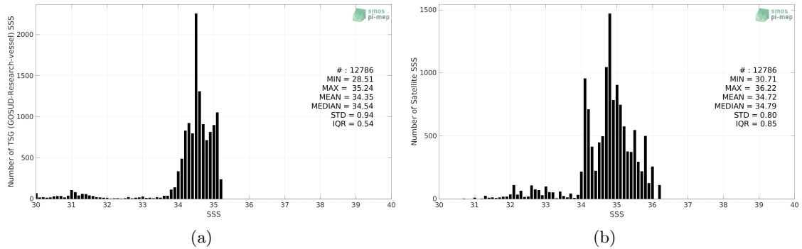
Figure 2: Histograms of SSS from TSG (GOSUD-Research-vessel) (a) and SMAP SSS L3 v5.0 - 8-Day running (JPL) (b) considering all match-up pairs per bins of 0.1 over the Arctic Ocean Pi-MEP region and for the full satellite product period.
