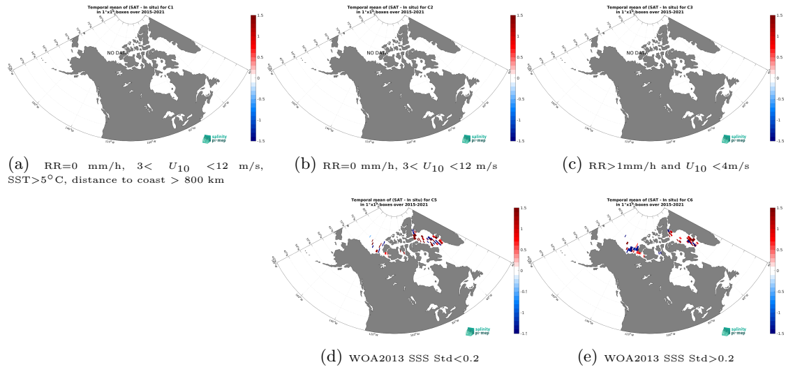
Figure 12: Temporal mean gridded over spatial boxes of size 1^{\circ}\times 1^{\circ} of \Delta\text{SSS} (SMAP SSS L3 v5.0 - 8-Day running (JPL) - TSG (Amundsen)) for 5 different subdatasets corresponding to:RR=0 mm/h, 3 < U_{10} < 12 m/s, SST >5^{\circ}\text{C} , distance to coast > 800 km (a), RR=0 mm/h, 3 < U_{10} < 12 m/s (b), RR >1 mm/h and U_{10} < 4 m/s (c), WOA2013 SSS Std <0.2 (d), WOA2013 SSS Std >0.2 (e).
