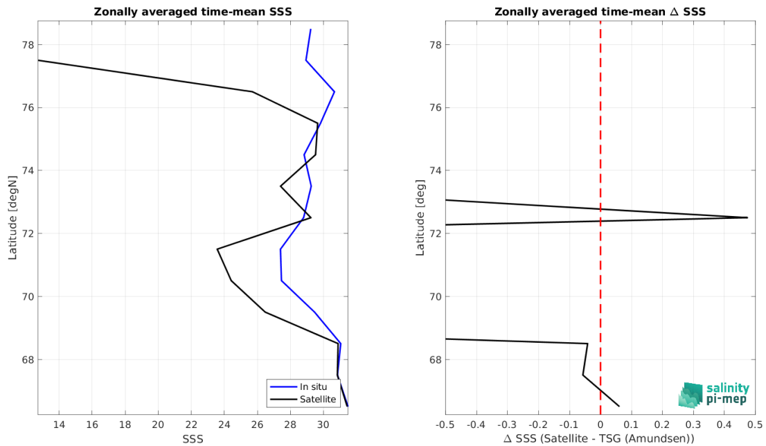
Figure 8: Left panel: Zonal mean SSS from SMAP SSS L3 v5.0 - 8-Day running (JPL) satellite product (black) and from TSG (Amundsen) (blue). Right panel: Zonal mean of \Delta SSS (Satellite - TSG (Amundsen)) for all the collected Pi-MEP match-up pairs estimated over the full satellite product period.
