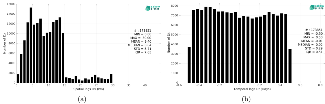
Figure 5: Histograms of the spatial (a) and temporal (b) lags between the location/time of the TSG (Amundsen) measurement and the date of the corresponding SMAP SSS L3 v5.0 - 8-Day running (JPL) SSS pixel.
