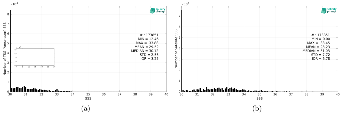
Figure 2: Histograms of SSS from TSG (Amundsen) (a) and SMAP SSS L3 v5.0 - 8-Day running (JPL) (b) considering all match-up pairs per bins of 0.1 over the Arctic Ocean Pi-MEP region and for the full satellite product period.
