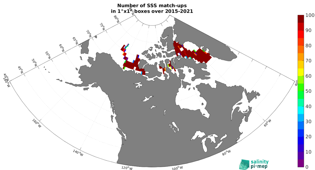
Figure 4: Number of SSS match-ups between TSG (Amundsen) SSS and the SMAP SSS L3 v5.0 - 8-Day running (JPL) SSS product for the Arctic Ocean Pi-MEP region over 1^\circ \times 1^\circ boxes and for the full satellite product period.
