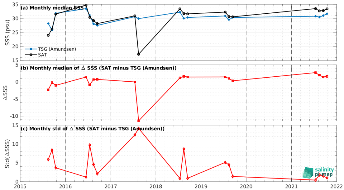
Figure 7: Time series of the monthly median SSS (top), median of \Delta SSS (Satellite - TSG (Amundsen)) and Std of \Delta SSS (Satellite - TSG (Amundsen)) over the Arctic Ocean Pi-MEP region considering all match-ups collected by the Pi-MEP.
