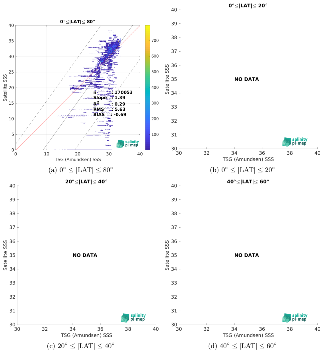
Figure 9: Contour maps of the concentration of SMAP SSS L3 v5.0 - 8-Day running (JPL) SSS (y-axis) versus TSG (Amundsen) SSS (x-axis) at match-up pairs for different latitude bands. For each plot, the red line shows x=y . The black thin and dashed lines indicate a linear fit through the data cloud and the \pm 95\% confidence levels, respectively. The number match-up pairs n , the slope and R^2 coefficient of the linear fit, the root mean square (RMS) and the mean bias between satellite and in situ data are indicated for each latitude band in each plots.
