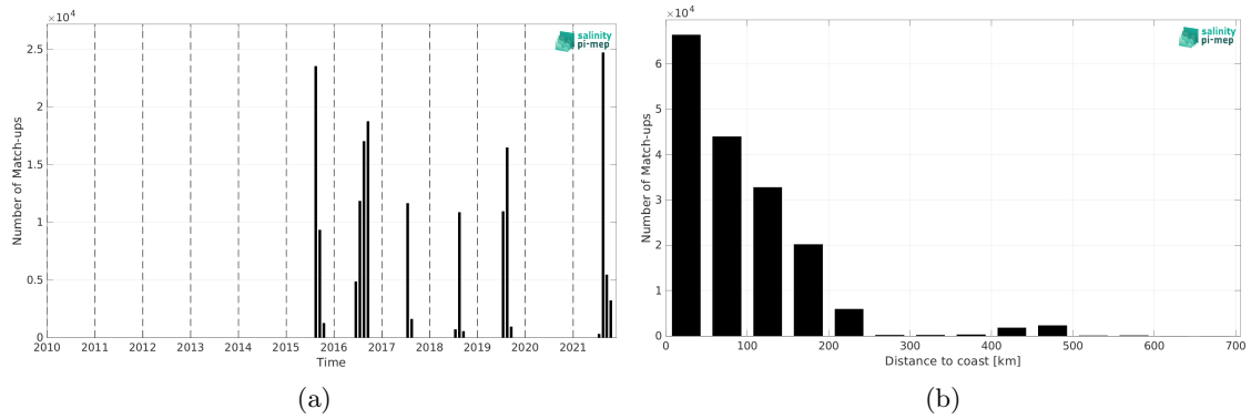
Figure 1: Number of match-ups between TSG (Amundsen) and SMAP SSS L3 v5.0 - 8-Day running (JPL) SSS as a function of time (a) and as function of the distance to coast (b) over the Arctic Ocean Pi-MEP region and for the full satellite product period.
