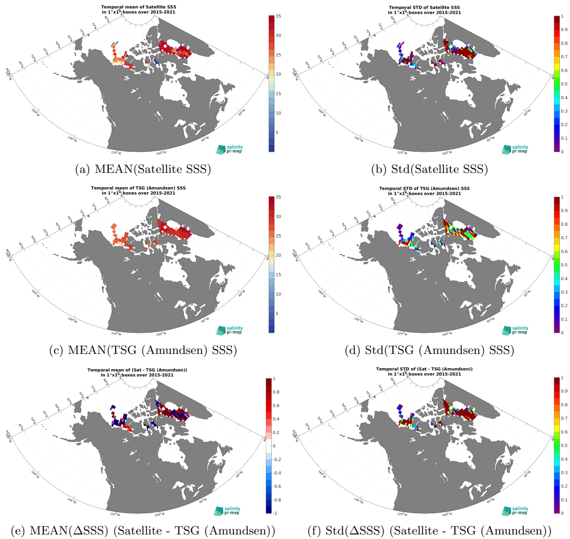
Figure 6: Temporal mean (left) and Std (right) of SSS from SMAP SSS L3 v5.0 - 8-Day running (JPL) (top), TSG (Amundsen) (middle), and of \Delta SSS (Satellite - TSG (Amundsen)). Only match-up pairs are used to generate these maps.
