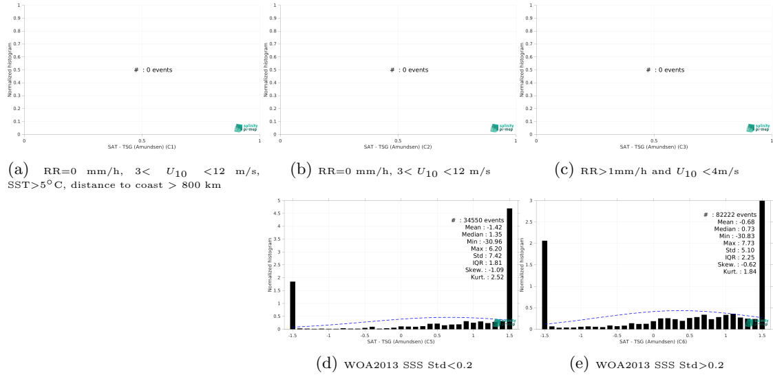
Figure 13: Normalized histogram of \Delta SSS (SMAP SSS L3 v5.0 - 8-Day running (JPL) - TSG (Amundsen)) for 5 different subdatasets corresponding to: RR=0 mm/h, 3 < U_{10} < 12 m/s, SST>5°C, distance to coast > 800 km (a), RR=0 mm/h, 3 < U_{10} < 12 m/s (b), RR>1mm/h and U_{10} < 4 m/s (c), WOA2013 SSS Std<0.2 (d), WOA2013 SSS Std>0.2 (e).
