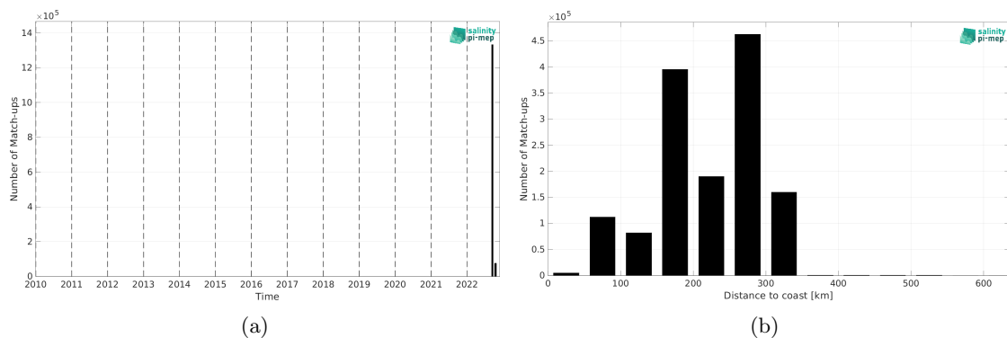
Figure 2: Number of match-ups between SASSIE and SMAP SSS L3 v5.0 - 8-Day running (JPL) SSS as a function of time (a) and as function of the distance to coast (b) over the Arctic Ocean Pi-MEP region and for the full satellite product period.
