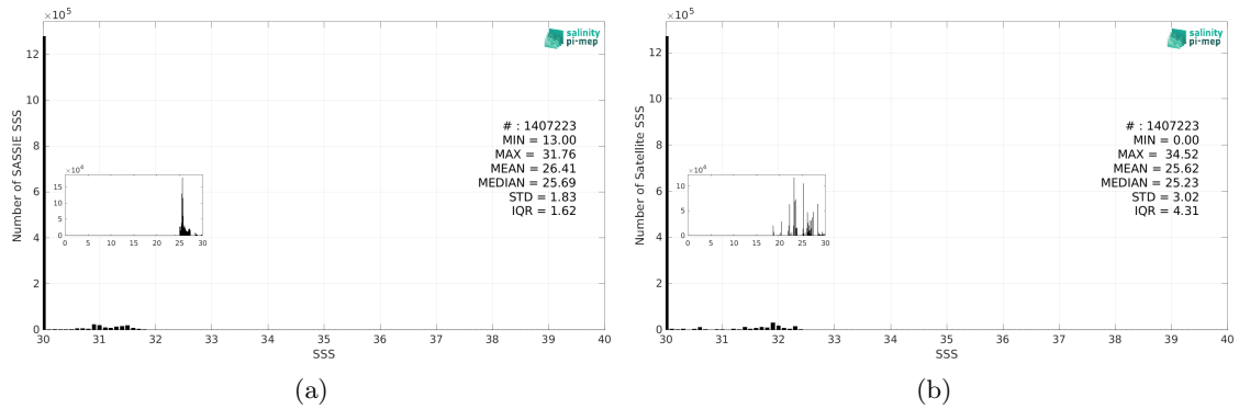
Figure 3: Histograms of SSS from SASSIE (a) and SMAP SSS L3 v5.0 - 8-Day running (JPL) (b) considering all match-up pairs per bins of 0.1 over the Arctic Ocean Pi-MEP region and for the full satellite product period.
