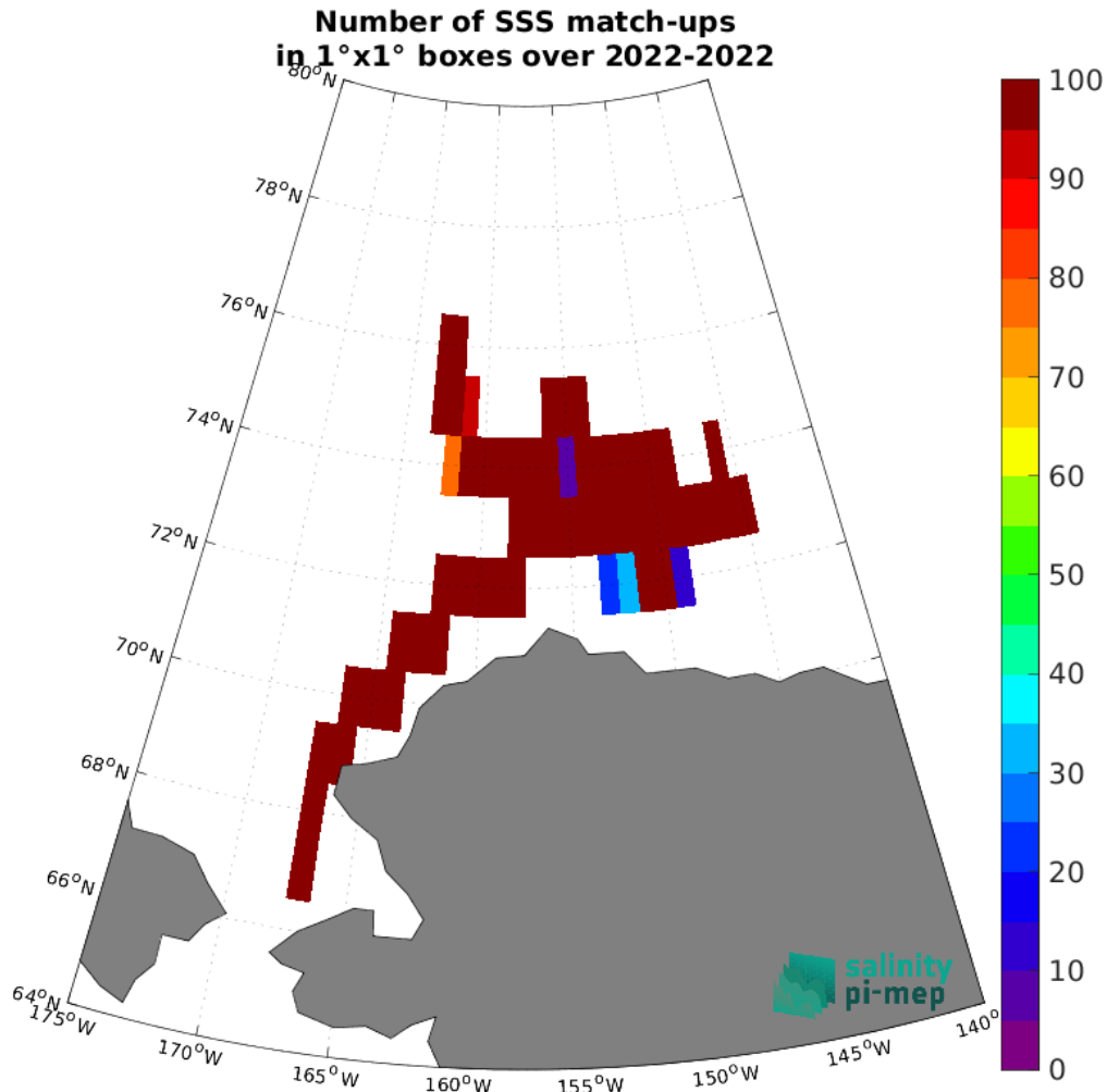
Figure 5: Number of SSS match-ups between SASSIE SSS and the SMAP SSS L3 v5.0 - 8-Day running (JPL) SSS product for the Arctic Ocean Pi-MEP region over 1^\circ \times 1^\circ boxes and for the full satellite product period.
