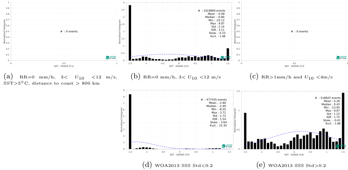
Figure 15: Normalized histogram of \Delta SSS (SMAP SSS L3 v5.0 - 8-Day running (JPL) - SASSIE) for 5 different subdatasets corresponding to: RR=0 mm/h, 3 < U_{10} < 12 m/s, SST>5°C, distance to coast > 800 km (a), RR=0 mm/h, 3 < U_{10} < 12 m/s (b), RR>1mm/h and U_{10} < 4 m/s (c), WOA2013 SSS Std<0.2 (d), WOA2013 SSS Std>0.2 (e).
