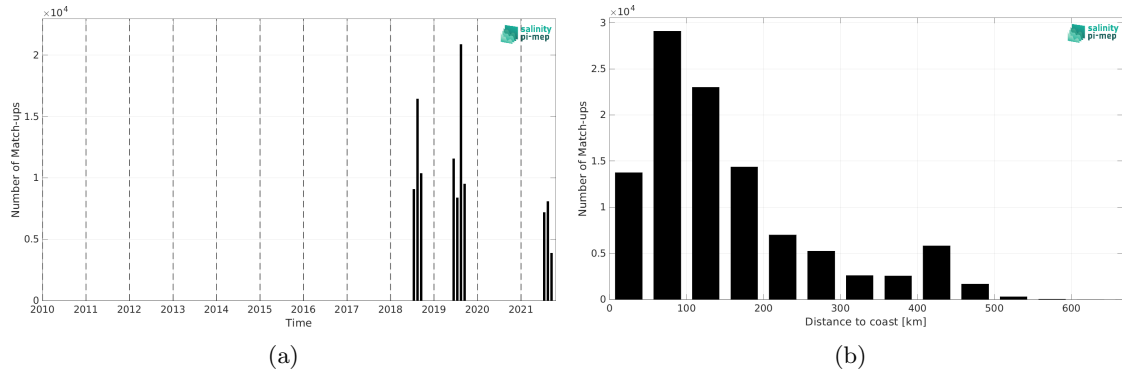
Figure 2: Number of match-ups between Sairdrone and SMAP SSS L3 v5.0 - 8-Day running (JPL) SSS as a function of time (a) and as function of the distance to coast (b) over the Arctic Ocean Pi-MEP region and for the full satellite product period.
