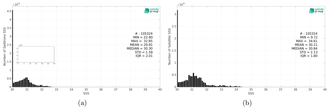
Figure 2: Histograms of SSS from Sairdrone (a) and SMAP SSS L3 v5.0 - 8-Day running (JPL) (b) considering all match-up pairs per bins of 0.1 over the Arctic Ocean Pi-MEP region and for the full satellite product period.
