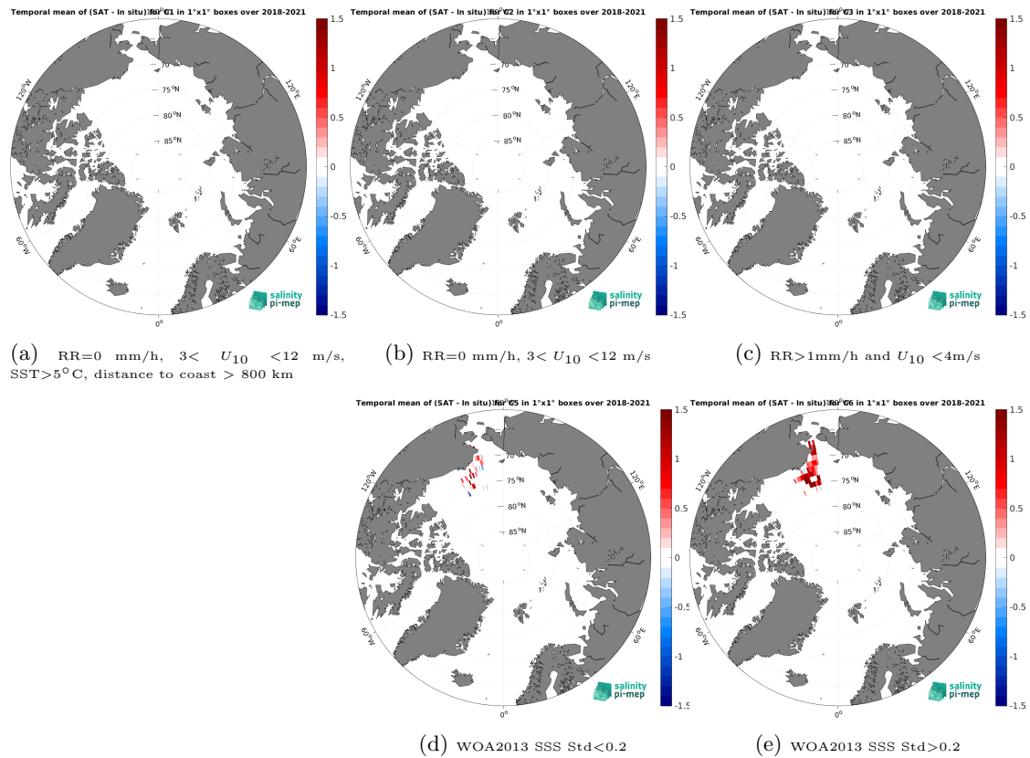
Figure 12: Temporal mean gridded over spatial boxes of size 1^{\circ}\times 1^{\circ} of \Delta\text{SSS} (SMAP SSS L3 v5.0 - 8-Day running (JPL) - Sairdrone) for 5 different subdatasets corresponding to:RR=0 mm/h, 3 < U_{10} < 12 m/s, SST > 5^{\circ}\text{C} , distance to coast > 800 km (a), RR=0 mm/h, 3 < U_{10} < 12 m/s (b), RR > 1 mm/h and U_{10} < 4 m/s (c), WOA2013 SSS Std < 0.2 (d), WOA2013 SSS Std > 0.2 (e).
