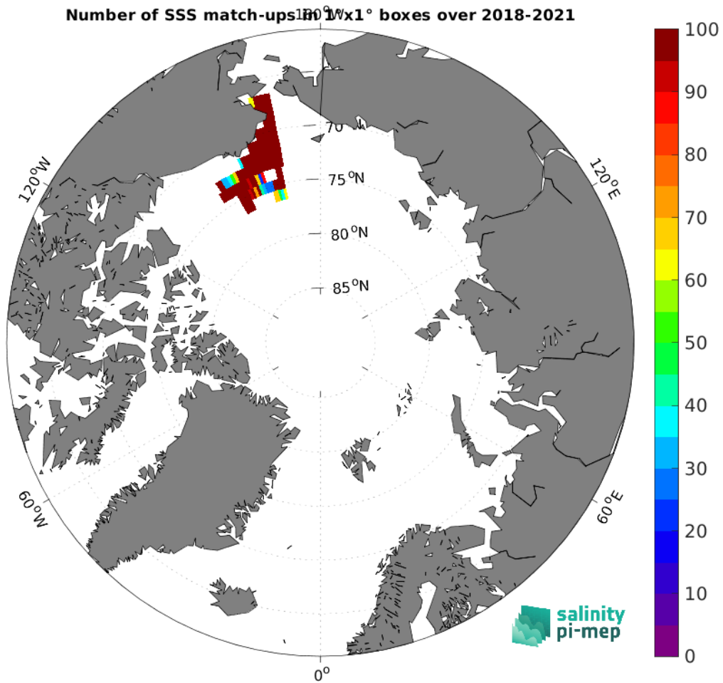
Figure 4: Number of SSS match-ups between Saildrone SSS and the SMAP SSS L3 v5.0 - 8-Day running (JPL) SSS product for the Arctic Ocean Pi-MEP region over 1^\circ \times 1^\circ boxes and for the full satellite product period.
