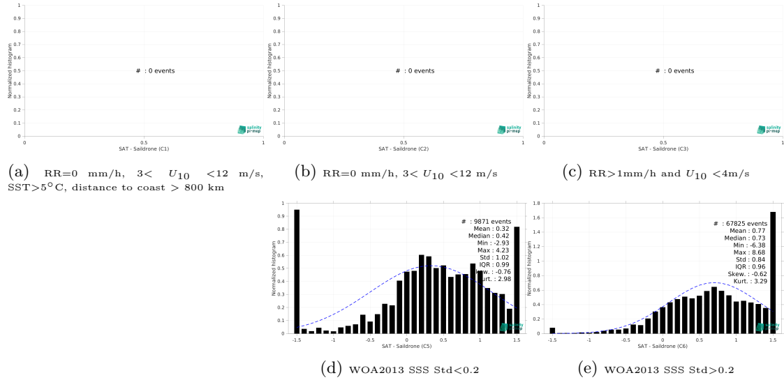
Figure 13: Normalized histogram of \Delta SSS (SMAP SSS L3 v5.0 - 8-Day running (JPL) - Saïdrone) for 5 different subdatasets corresponding to: RR=0 mm/h, 3 < U_{10} < 12 m/s, SST > 5°C, distance to coast > 800 km (a), RR=0 mm/h, 3 < U_{10} < 12 m/s (b), RR > 1mm/h and U_{10} < 4 m/s (c), WOA2013 SSS Std < 0.2 (d), WOA2013 SSS Std > 0.2 (e).
