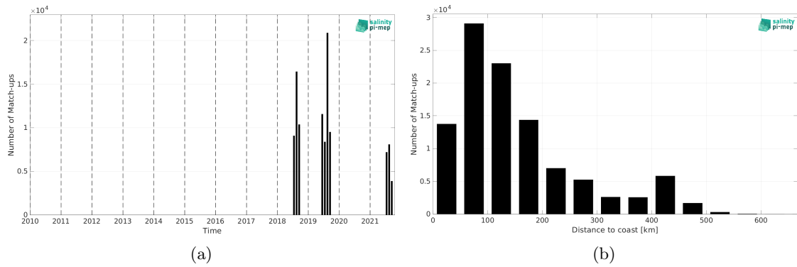
Figure 1: Number of match-ups between Sairdrone and SMAP SSS L3 v5.0 - 8-Day running (JPL) SSS as a function of time (a) and as function of the distance to coast (b) over the Arctic Ocean Pi-MEP region and for the full satellite product period.
