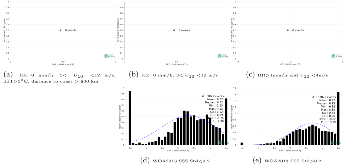
Figure 13: Normalized histogram of \Delta SSS (SMAP SSS L3 v5.0 - 8-Day running (JPL) - Saikdrone) for 5 different subdatasets corresponding to: RR=0 mm/h, 3 < U_{10} < 12 m/s, SST > 5°C, distance to coast > 800 km (a), RR=0 mm/h, 3 < U_{10} < 12 m/s (b), RR > 1mm/h and U_{10} < 4 m/s (c), WOA2013 SSS Std < 0.2 (d), WOA2013 SSS Std > 0.2 (e).
