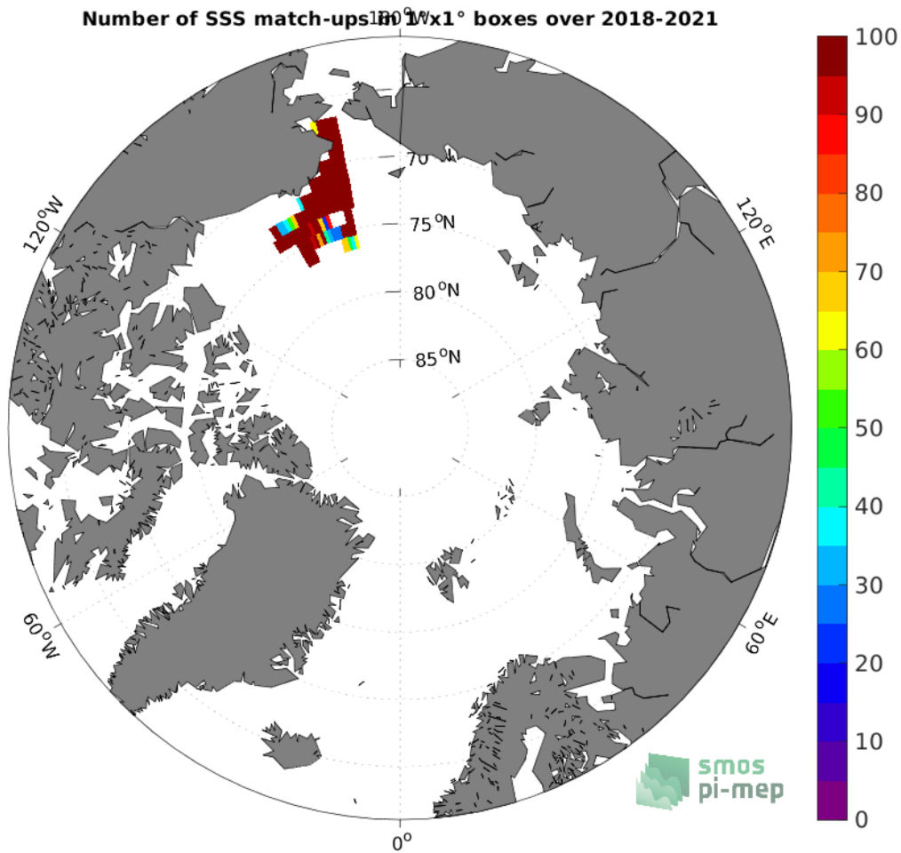
Figure 4: Number of SSS match-ups between Saildrone SSS and the SMAP SSS L3 v5.0 - 8-Day running (JPL) SSS product for the Arctic Ocean Pi-MEP region over 1^{\circ} \times 1^{\circ} boxes and for the full satellite product period.
