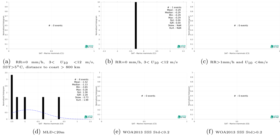
Figure 15: Normalized histogram of \Delta SSS (SMAP SSS L3 v5.0 - 8-Day running (JPL) - Marine mammals) for 6 different subdatasets corresponding to: RR=0 mm/h, 3 < U_{10} < 12 m/s, SST >5^{\circ} C, distance to coast > 800 km (a), RR=0 mm/h, 3 < U_{10} < 12 m/s (b), RR >1 mm/h and U_{10} < 4 m/s (c), MLD <20 m (d), WOA2013 SSS Std <0.2 (e), WOA2013 SSS Std >0.2 (f).
