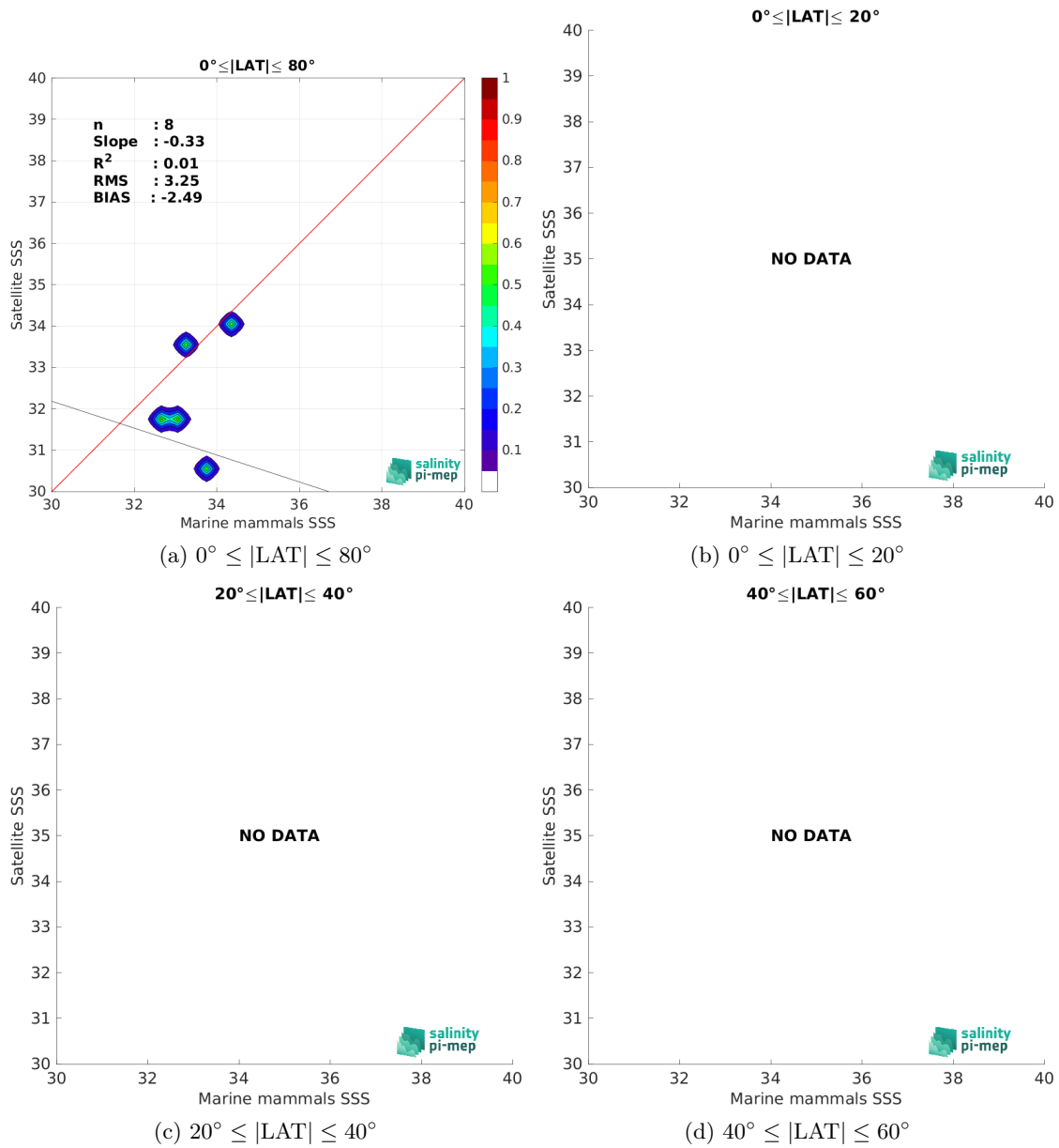
Figure 10: Contour maps of the concentration of SMAP SSS L3 v5.0 - 8-Day running (JPL) SSS (y-axis) versus Marine mammals SSS (x-axis) at match-up pairs for different latitude bands. For each plot, the red line shows x=y . The black thin and dashed lines indicate a linear fit through the data cloud and the \pm 95\% confidence levels, respectively. The number match-up pairs n , the slope and R^2 coefficient of the linear fit, the root mean square (RMS) and the mean bias between satellite and in situ data are indicated for each latitude band in each plots.
