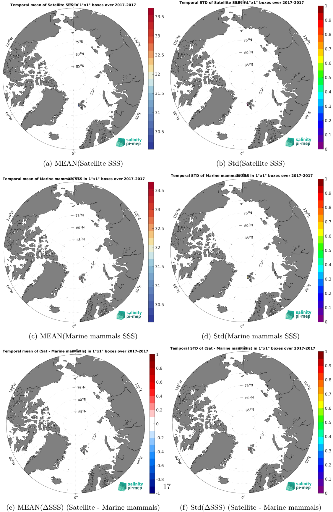
Figure 7: Temporal mean (left) and Std (right) of SSS from SMAP SSS L3 v5.0 - 8-Day running (JPL) (top), Marine mammals (middle), and of \Delta SSS (Satellite - Marine mammals). Only match-up pairs are used to generate these maps.
