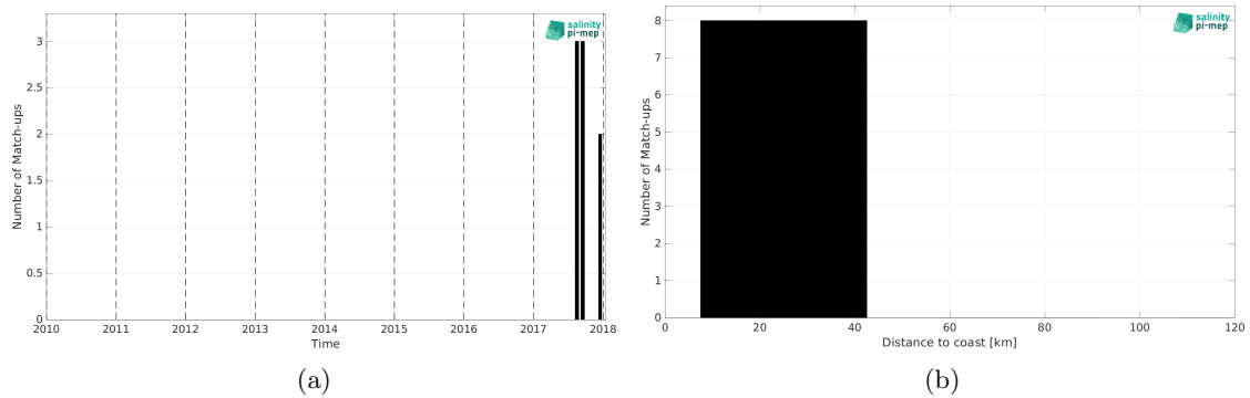
Figure 2: Number of match-ups between Marine mammals and SMAP SSS L3 v5.0 - 8-Day running (JPL) SSS as a function of time (a) and as function of the distance to coast (b) over the Arctic Ocean Pi-MEP region and for the full satellite product period.
