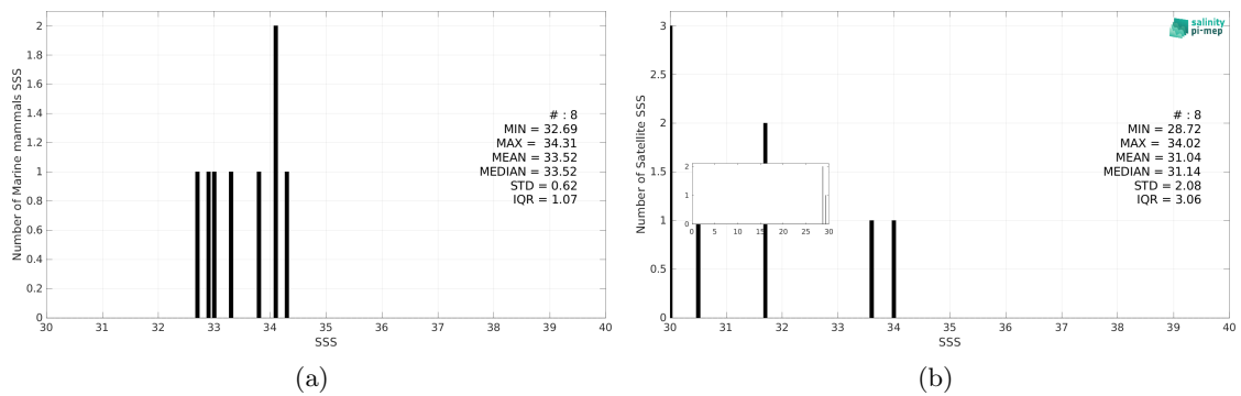
Figure 3: Histograms of SSS from Marine mammals (a) and SMAP SSS L3 v5.0 - 8-Day running (JPL) (b) considering all match-up pairs per bins of 0.1 over the Arctic Ocean Pi-MEP region and for the full satellite product period.
