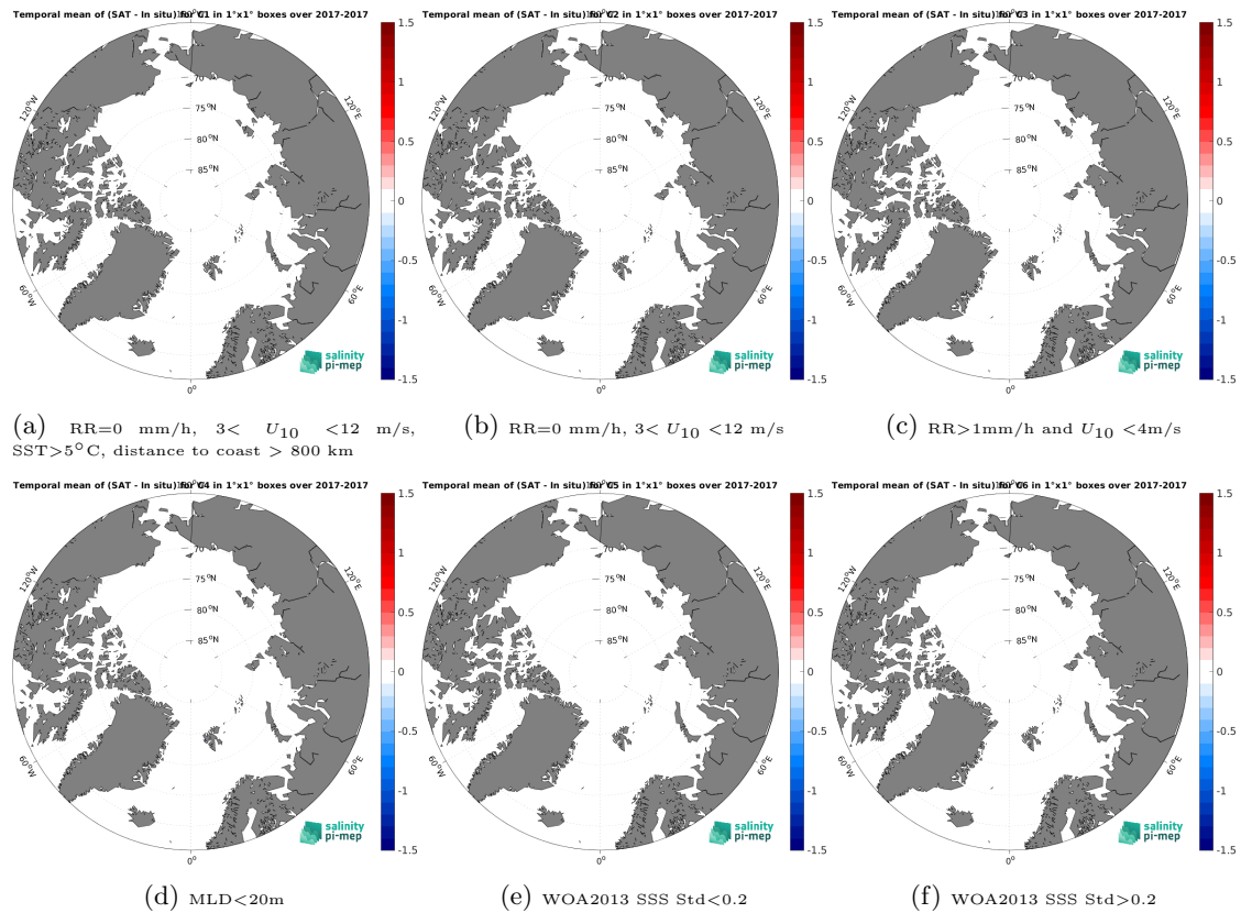
Figure 14: Temporal mean gridded over spatial boxes of size 1^\circ \times 1^\circ of \Delta SSS (SMAP SSS L3 v5.0 - 8-Day running (JPL) - Marine mammals) for 6 different subdatasets corresponding to:RR=0 mm/h, 3 < U_{10} < 12 m/s, SST>5°C, distance to coast > 800 km (a), RR=0 mm/h, 3 < U_{10} < 12 m/s (b), RR>1mm/h and U_{10} < 4 m/s (c),MLD<20m (d),WOA2013 SSS Std<0.2 (e),WOA2013 SSS Std>0.2 (f).
