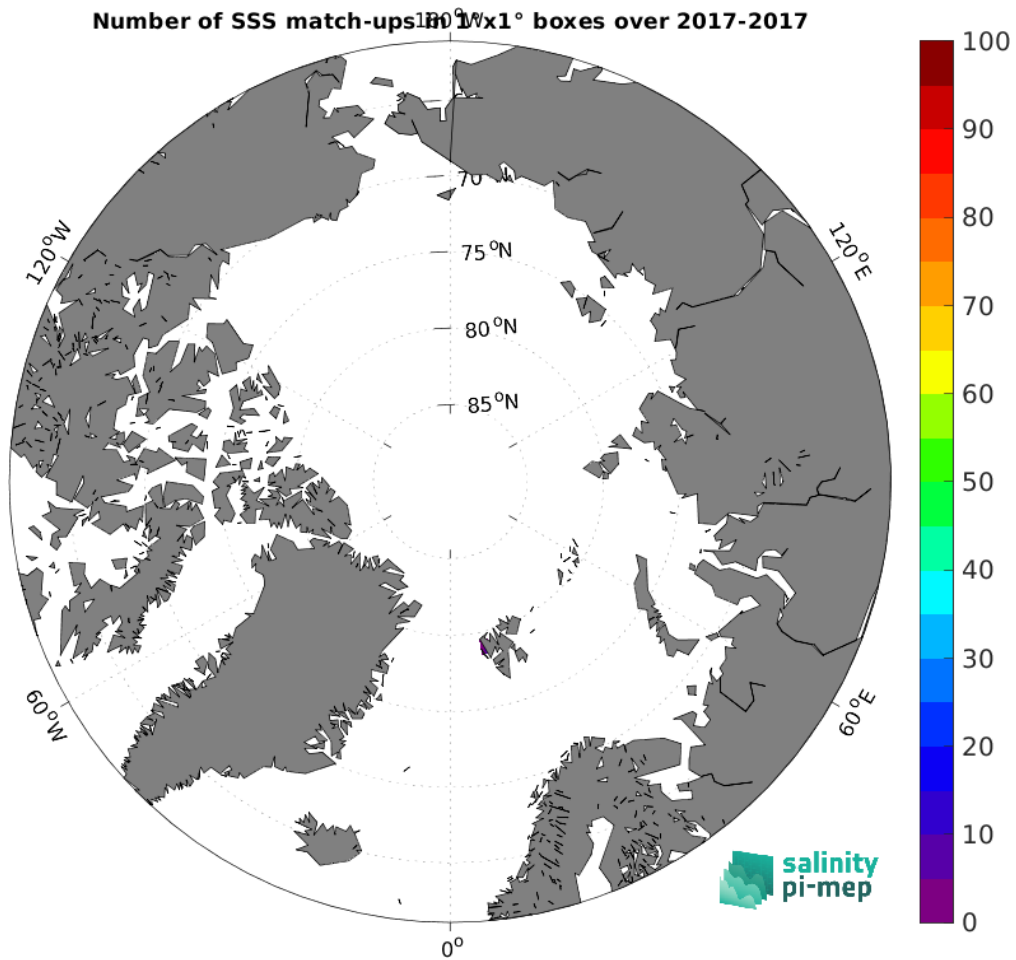
Figure 5: Number of SSS match-ups between Marine mammals SSS and the SMAP SSS L3 v5.0 - 8-Day running (JPL) SSS product for the Arctic Ocean Pi-MEP region over 1^\circ \times 1^\circ boxes and for the full satellite product period.
