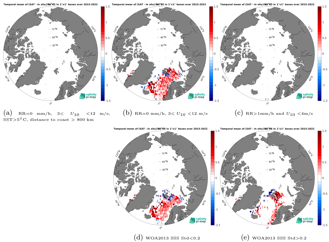
Figure 14: Temporal mean gridded over spatial boxes of size 1^\circ \times 1^\circ of \Delta SSS (SMAP SSS L3 v5.0 - 8-Day running (JPL) - ICES) for 5 different subdatasets corresponding to:RR=0 mm/h, 3 < U_{10} < 12 m/s, SST>5°C, distance to coast > 800 km (a), RR=0 mm/h, 3 < U_{10} < 12 m/s (b), RR>1mm/h and U_{10} < 4 m/s (c), WOA2013 SSS Std<0.2 (d), WOA2013 SSS Std>0.2 (e).
