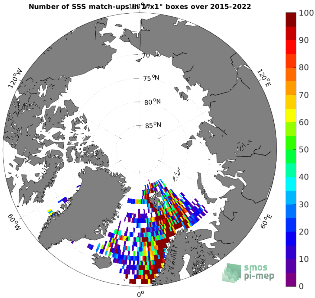
Figure 4: Number of SSS match-ups between ICES SSS and the SMAP SSS L3 v5.0 - 8-Day running (JPL) SSS product for the Arctic Ocean Pi-MEP region over 1^{\circ} \times 1^{\circ} boxes and for the full satellite product period.
