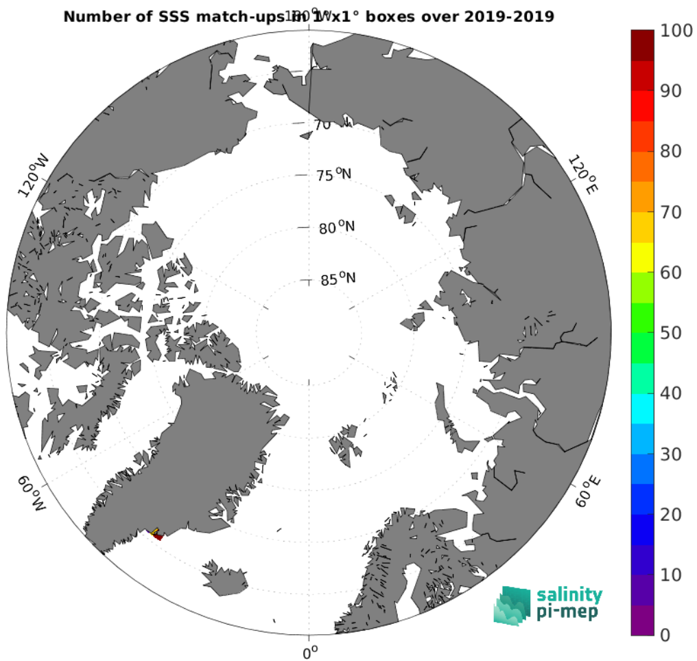
Figure 3: Number of SSS match-ups between Surface drifters SSS and the SMAP SSS L3 v5.0 - 8-Day running (JPL) SSS product for the Arctic Ocean Pi-MEP region over 1^\circ \times 1^\circ boxes and for the full satellite product period.
