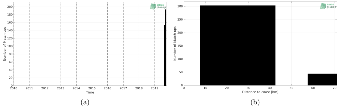
Figure 1: Number of match-ups between Surface drifters and SMAP SSS L3 v5.0 - 8-Day running (JPL) SSS as a function of time (a) and as function of the distance to coast (b) over the Arctic Ocean Pi-MEP region and for the full satellite product period.
