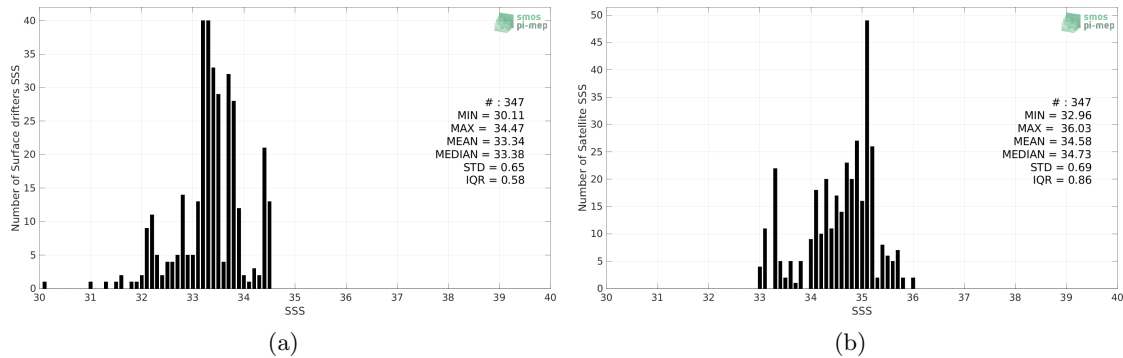
Figure 2: Histograms of SSS from Surface drifters (a) and SMAP SSS L3 v5.0 - 8-Day running (JPL) (b) considering all match-up pairs per bins of 0.1 over the Arctic Ocean Pi-MEP region and for the full satellite product period.
