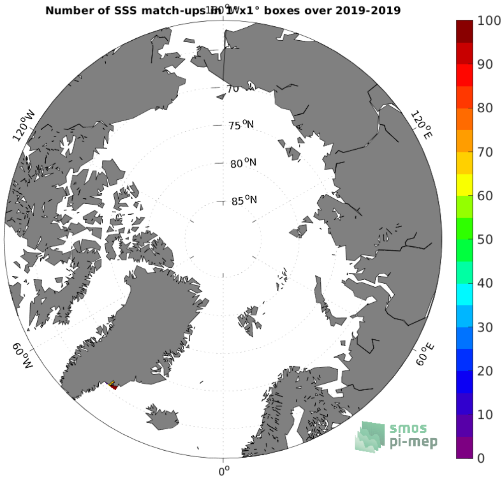
Figure 3: Number of SSS match-ups between Surface drifters SSS and the SMAP SSS L3 v5.0 - 8-Day running (JPL) SSS product for the Arctic Ocean Pi-MEP region over 1^{\circ} \times 1^{\circ} boxes and for the full satellite product period.
