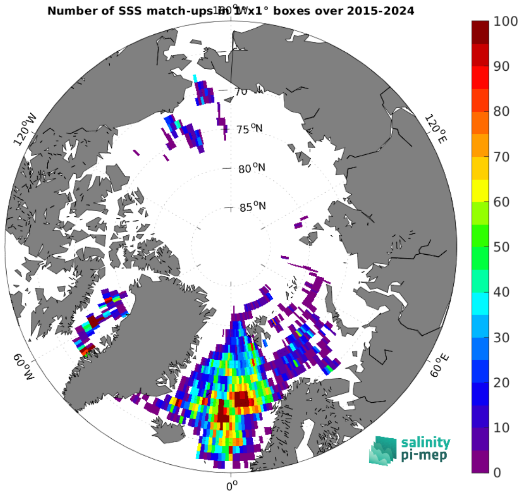
Figure 5: Number of SSS match-ups between Argo SSS and the SMAP SSS L3 v5.0 - 8-Day running (JPL) SSS product for the Arctic Ocean Pi-MEP region over 1^\circ \times 1^\circ boxes and for the full satellite product period.
