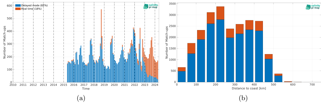
Figure 2: Number of match-ups between Argo and SMAP SSS L3 v5.0 - 8-Day running (JPL) SSS as a function of time (a) and as function of the distance to coast (b) over the Arctic Ocean Pi-MEP region and for the full satellite product period.
