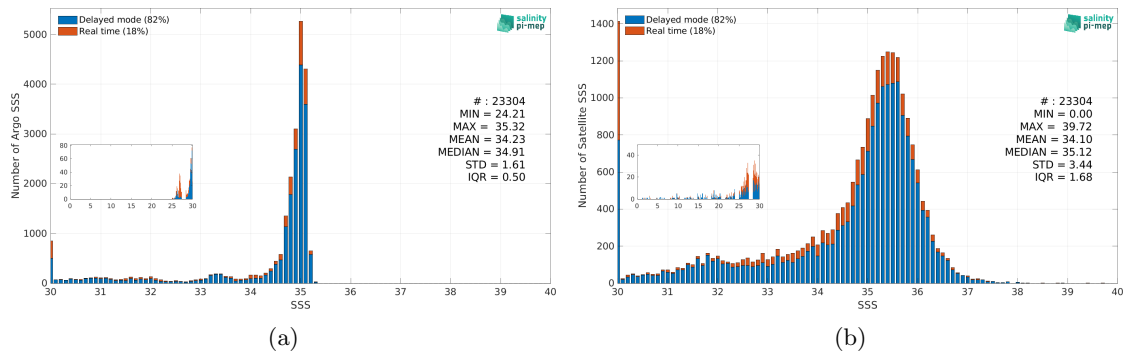
Figure 3: Histograms of SSS from Argo (a) and SMAP SSS L3 v5.0 - 8-Day running (JPL) (b) considering all match-up pairs per bins of 0.1 over the Arctic Ocean Pi-MEP region and for the full satellite product period.
