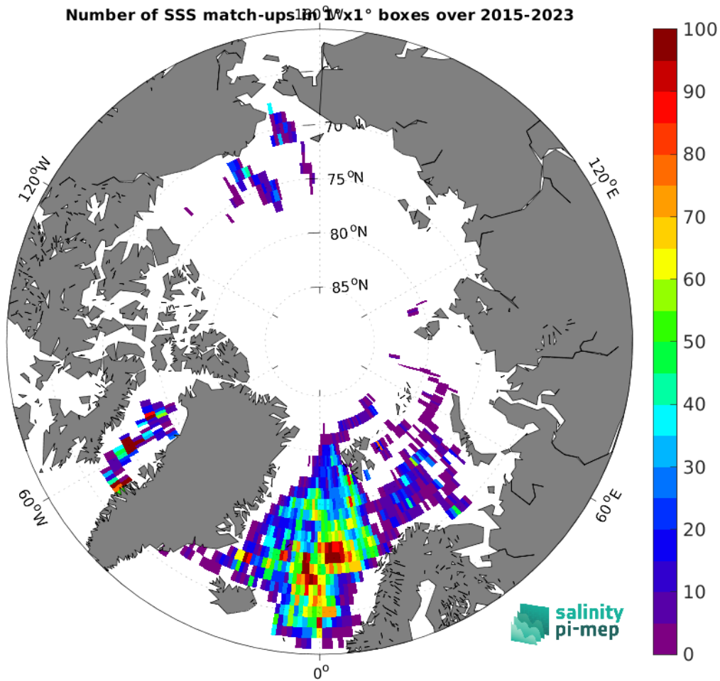
Figure 4: Number of SSS match-ups between Argo SSS and the SMAP SSS L3 v5.0 - 8-Day running (JPL) SSS product for the Arctic Ocean Pi-MEP region over 1^\circ \times 1^\circ boxes and for the full satellite product period.
