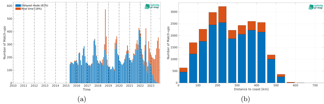
Figure 1: Number of match-ups between Argo and SMAP SSS L3 v5.0 - 8-Day running (JPL) SSS as a function of time (a) and as function of the distance to coast (b) over the Arctic Ocean Pi-MEP region and for the full satellite product period.
