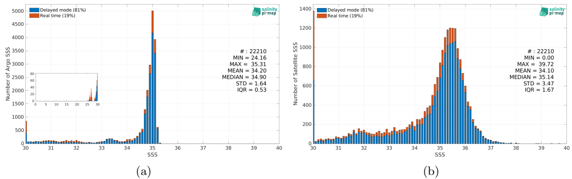
Figure 2: Histograms of SSS from Argo (a) and SMAP SSS L3 v5.0 - 8-Day running (JPL) (b) considering all match-up pairs per bins of 0.1 over the Arctic Ocean Pi-MEP region and for the full satellite product period.
