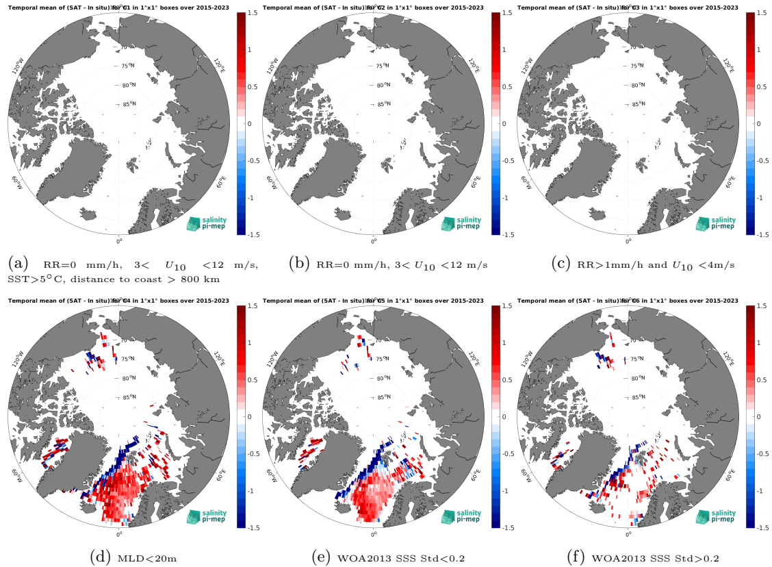
Figure 12: Temporal mean gridded over spatial boxes of size 1^{\circ}\times 1^{\circ} of \Delta\text{SSS} (SMAP SSS L3 v5.0 - 8-Day running (JPL) - Argo) for 6 different subdatasets corresponding to:RR=0 mm/h, 3 < U_{10} < 12 m/s, SST >5^{\circ}\text{C} , distance to coast > 800 km (a), RR=0 mm/h, 3 < U_{10} < 12 m/s (b), RR >1 mm/h and U_{10} < 4 m/s (c),MLD <20 m (d),WOA2013 SSS Std <0.2 (e),WOA2013 SSS Std >0.2 (f).
