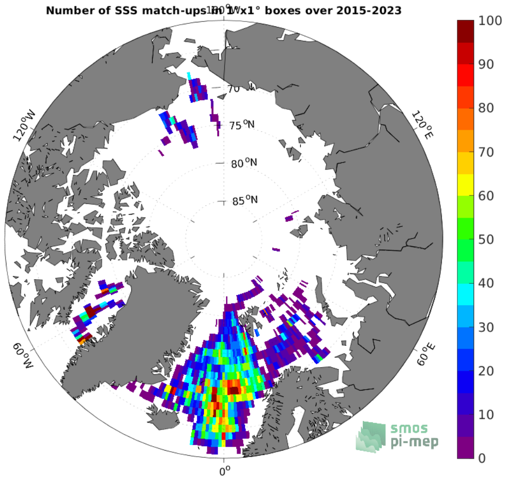
Figure 4: Number of SSS match-ups between Argo SSS and the SMAP SSS L3 v5.0 - 8-Day running (JPL) SSS product for the Arctic Ocean Pi-MEP region over 1^{\circ} \times 1^{\circ} boxes and for the full satellite product period.
