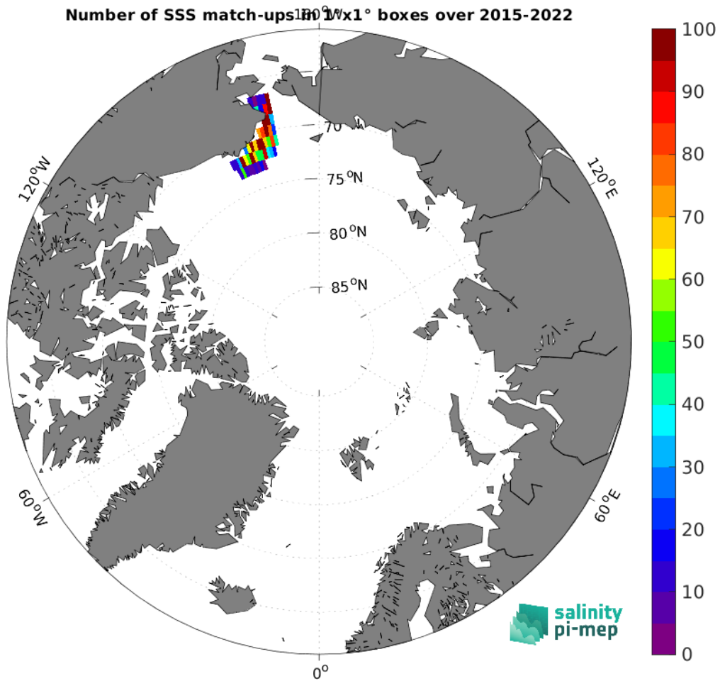
Figure 5: Number of SSS match-ups between TSG (SAMOS) SSS and the SMAP SSS L3 v5.0 - Monthly (JPL) SSS product for the Arctic Ocean Pi-MEP region over 1^\circ \times 1^\circ boxes and for the full satellite product period.
