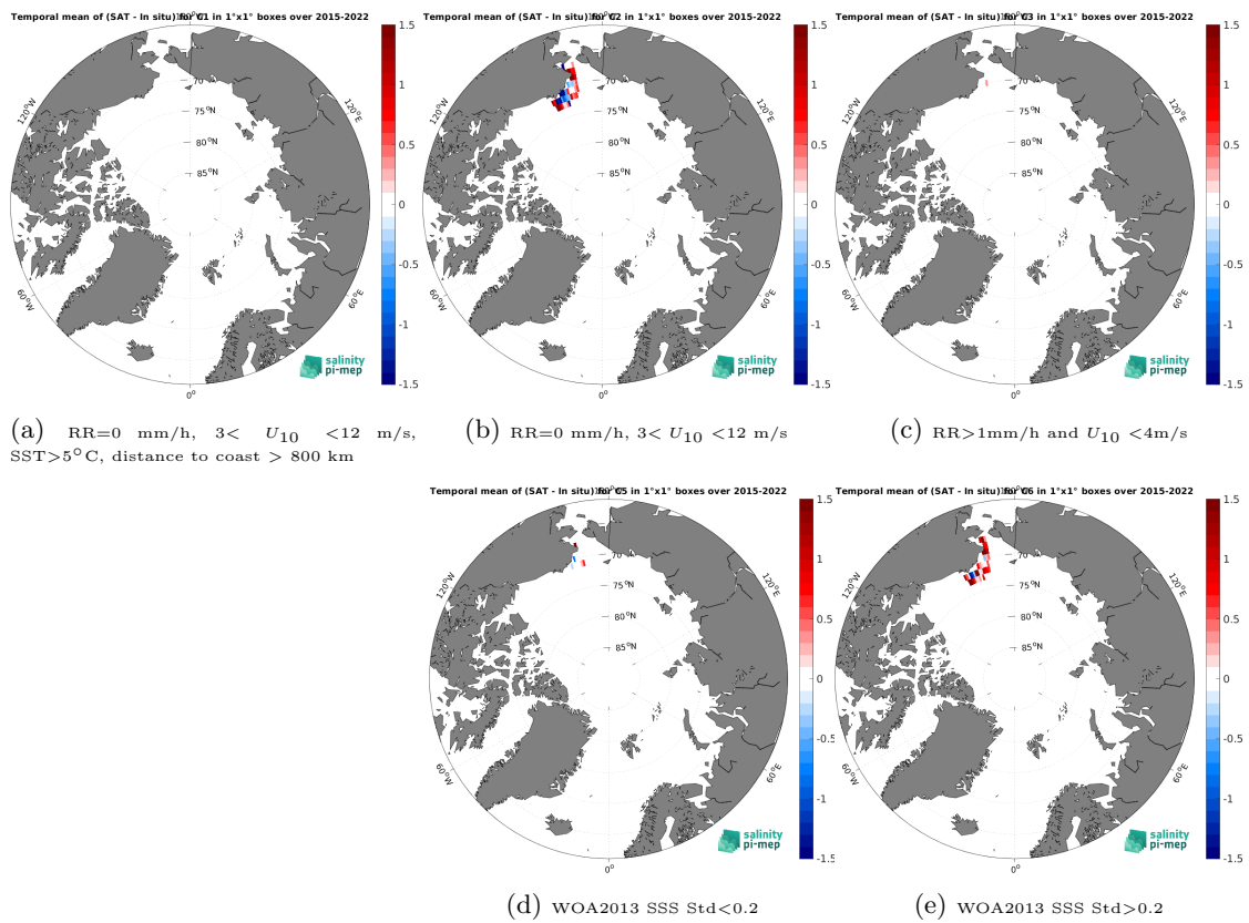
Figure 14: Temporal mean gridded over spatial boxes of size 1^\circ \times 1^\circ of \Delta SSS (SMAP SSS L3 v5.0 - Monthly (JPL) - TSG (SAMOS)) for 5 different subdatasets corresponding to:RR=0 mm/h, 3 < U_{10} < 12 m/s, SST > 5°C, distance to coast > 800 km (a), RR=0 mm/h, 3 < U_{10} < 12 m/s (b), RR > 1mm/h and U_{10} < 4 m/s (c), WOA2013 SSS Std < 0.2 (d), WOA2013 SSS Std > 0.2 (e).
