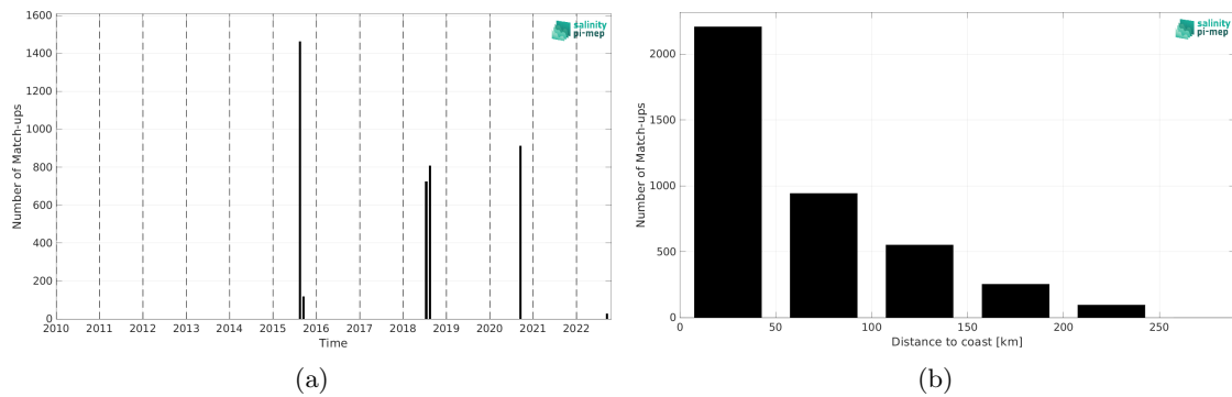
Figure 2: Number of match-ups between TSG (SAMOS) and SMAP SSS L3 v5.0 - Monthly (JPL) SSS as a function of time (a) and as function of the distance to coast (b) over the Arctic Ocean Pi-MEP region and for the full satellite product period.
