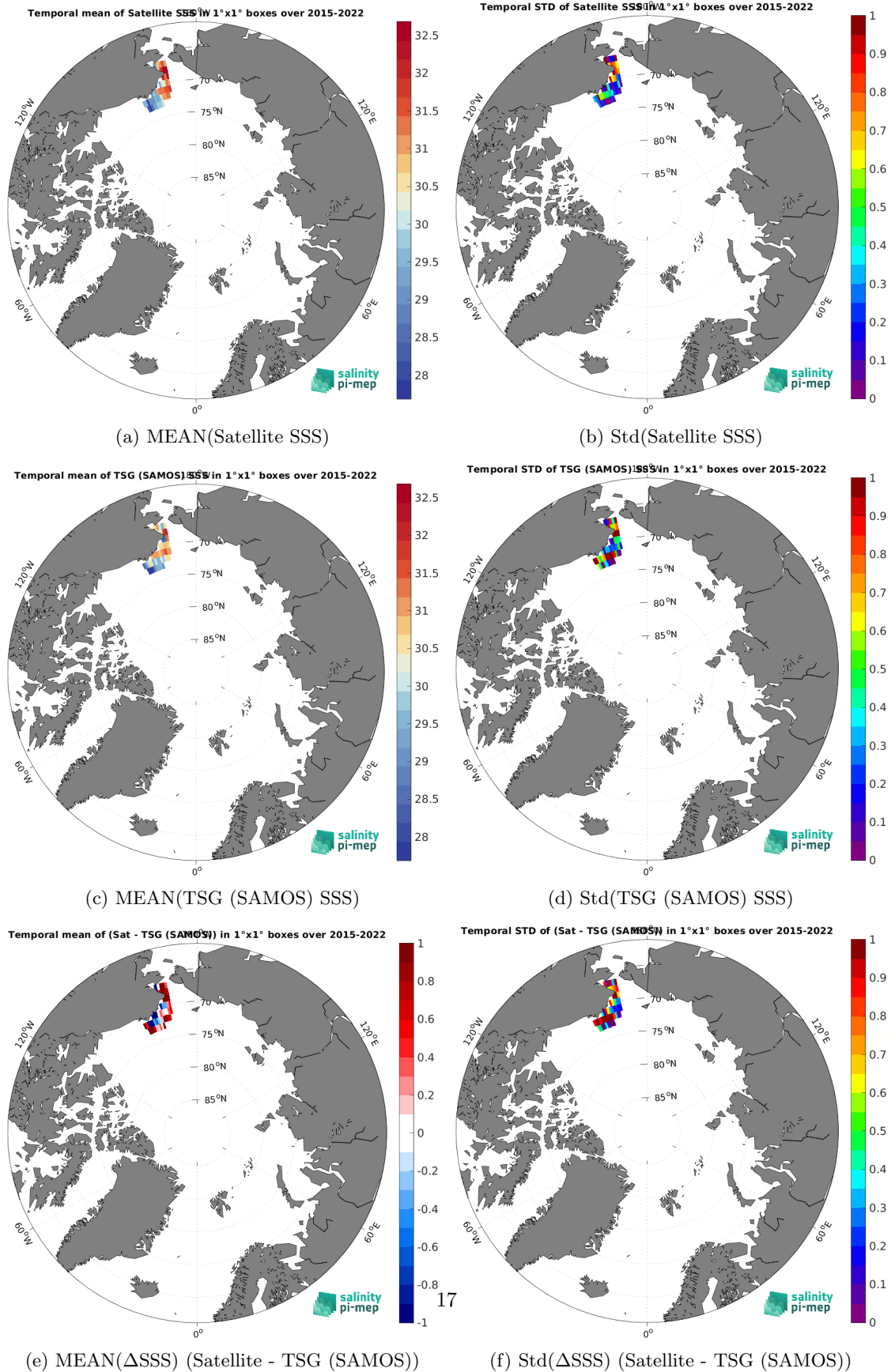
Figure 7: Temporal mean (left) and Std (right) of SSS from SMAP SSS L3 v5.0 - Monthly (JPL) (top), TSG (SAMOS) (middle), and of \Delta SSS (Satellite - TSG (SAMOS)). Only match-up pairs are used to generate these maps.
