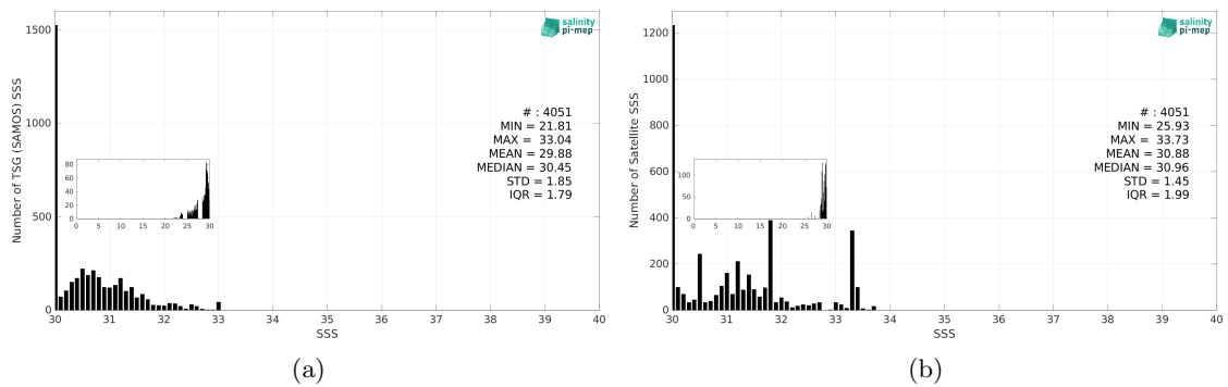
Figure 3: Histograms of SSS from TSG (SAMOS) (a) and SMAP SSS L3 v5.0 - Monthly (JPL) (b) considering all match-up pairs per bins of 0.1 over the Arctic Ocean Pi-MEP region and for the full satellite product period.
