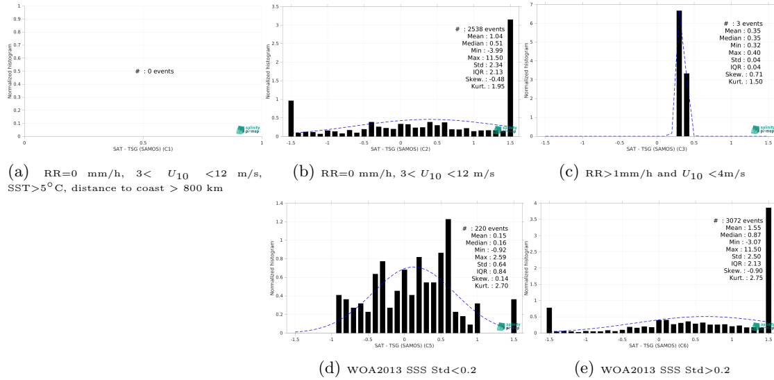
Figure 15: Normalized histogram of \Delta\text{SSS} (SMAP SSS L3 v5.0 - Monthly (JPL) - TSG (SAMOS)) for 5 different subdatasets corresponding to: RR=0 mm/h, 3 < U_{10} < 12 m/s, SST > 5^\circ\text{C} , distance to coast > 800 km (a), RR=0 mm/h, 3 < U_{10} < 12 m/s (b), RR > 1\text{mm/h} and U_{10} < 4\text{m/s} (c), WOA2013 SSS Std < 0.2 (d), WOA2013 SSS Std > 0.2 (e).
