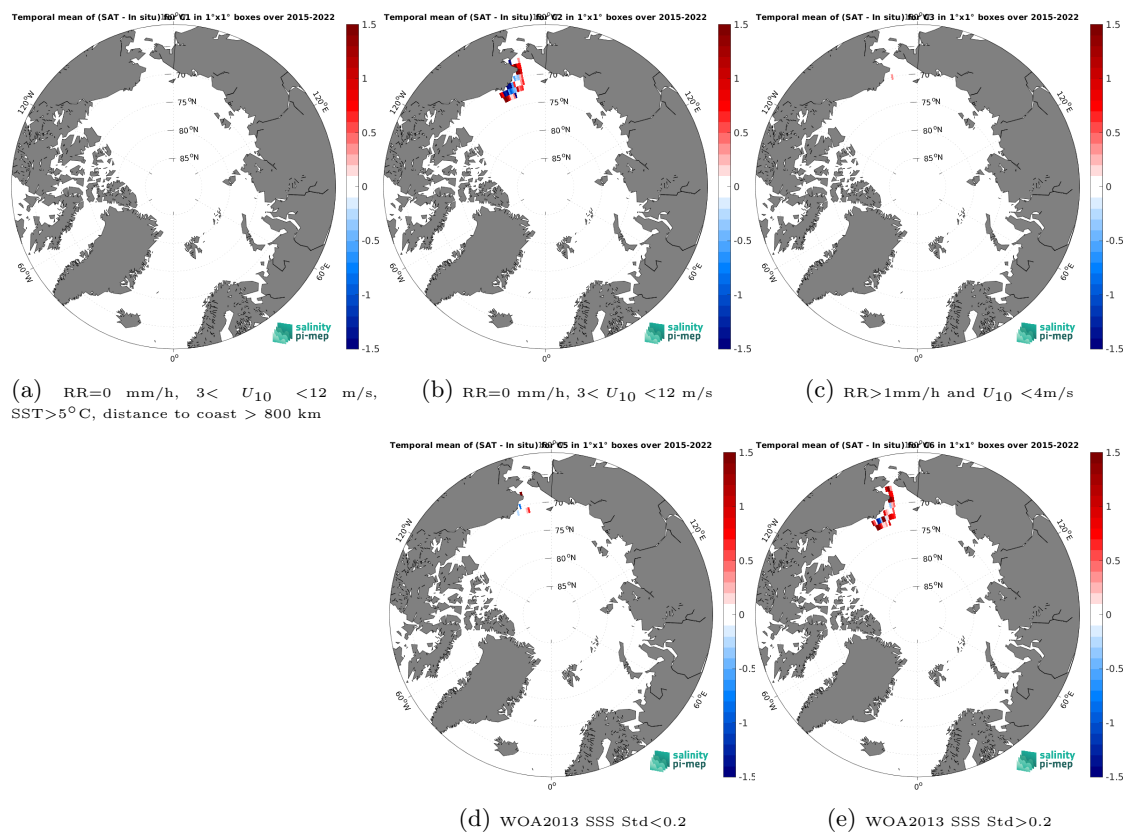
Figure 14: Temporal mean gridded over spatial boxes of size 1^\circ \times 1^\circ of \Delta\text{SSS} (SMAP SSS L3 v5.0 - Monthly (JPL) - TSG (SAMOS)) for 5 different subdatasets corresponding to: RR=0 mm/h, 3 < U_{10} < 12 m/s, SST > 5°C, distance to coast > 800 km (a), RR=0 mm/h, 3 < U_{10} < 12 m/s (b), RR > 1mm/h and U_{10} < 4 m/s (c), WOA2013 SSS Std < 0.2 (d), WOA2013 SSS Std > 0.2 (e).
