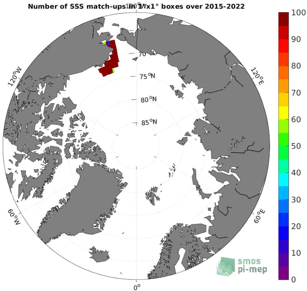
Figure 4: Number of SSS match-ups between TSG (SAMOS) SSS and the SMAP SSS L3 v5.0 - Monthly (JPL) SSS product for the Arctic Ocean Pi-MEP region over 1^{\circ} \times 1^{\circ} boxes and for the full satellite product period.
