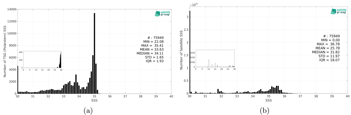
Figure 3: Histograms of SSS from TSG (Polarstern) (a) and SMAP SSS L3 v5.0 - Monthly (JPL) (b) considering all match-up pairs per bins of 0.1 over the Arctic Ocean Pi-MEP region and for the full satellite product period.
