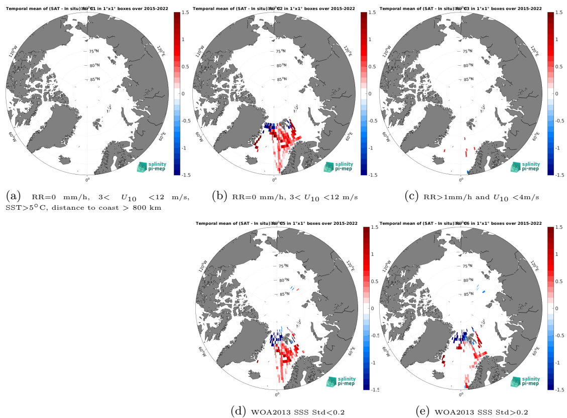
Figure 14: Temporal mean gridded over spatial boxes of size 1^\circ \times 1^\circ of \Delta SSS (SMAP SSS L3 v5.0 - Monthly (JPL) - TSG (Polarstern)) for 5 different subdatasets corresponding to: RR=0 mm/h, 3 < U_{10} < 12 m/s, SST > 5°C, distance to coast > 800 km (a), RR=0 mm/h, 3 < U_{10} < 12 m/s (b), RR > 1mm/h and U_{10} < 4 m/s (c), WOA2013 SSS Std < 0.2 (d), WOA2013 SSS Std > 0.2 (e).
