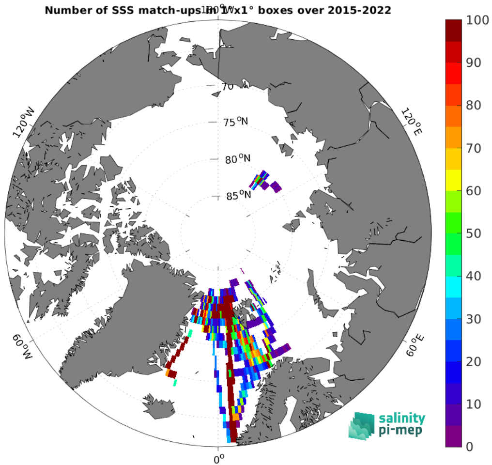
Figure 5: Number of SSS match-ups between TSG (Polarstern) SSS and the SMAP SSS L3 v5.0 - Monthly (JPL) SSS product for the Arctic Ocean Pi-MEP region over 1^\circ \times 1^\circ boxes and for the full satellite product period.
