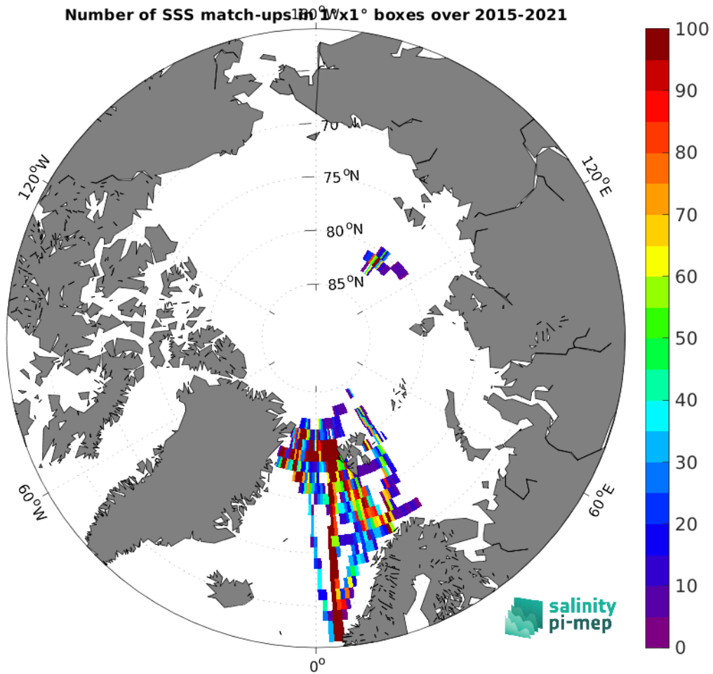
Figure 4: Number of SSS match-ups between TSG (Polarstern) SSS and the SMAP SSS L3 v5.0 - Monthly (JPL) SSS product for the Arctic Ocean Pi-MEP region over 1^\circ \times 1^\circ boxes and for the full satellite product period.
