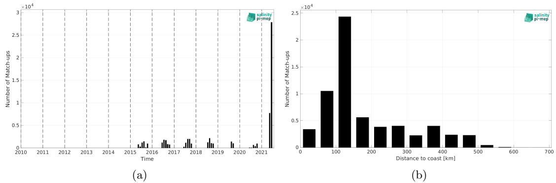
Figure 1: Number of match-ups between TSG (Polarstern) and SMAP SSS L3 v5.0 - Monthly (JPL) SSS as a function of time (a) and as function of the distance to coast (b) over the Arctic Ocean Pi-MEP region and for the full satellite product period.
