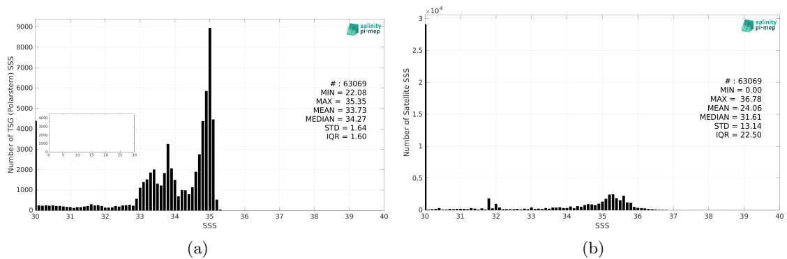
Figure 2: Histograms of SSS from TSG (Polarstern) (a) and SMAP SSS L3 v5.0 - Monthly (JPL) (b) considering all match-up pairs per bins of 0.1 over the Arctic Ocean Pi-MEP region and for the full satellite product period.
