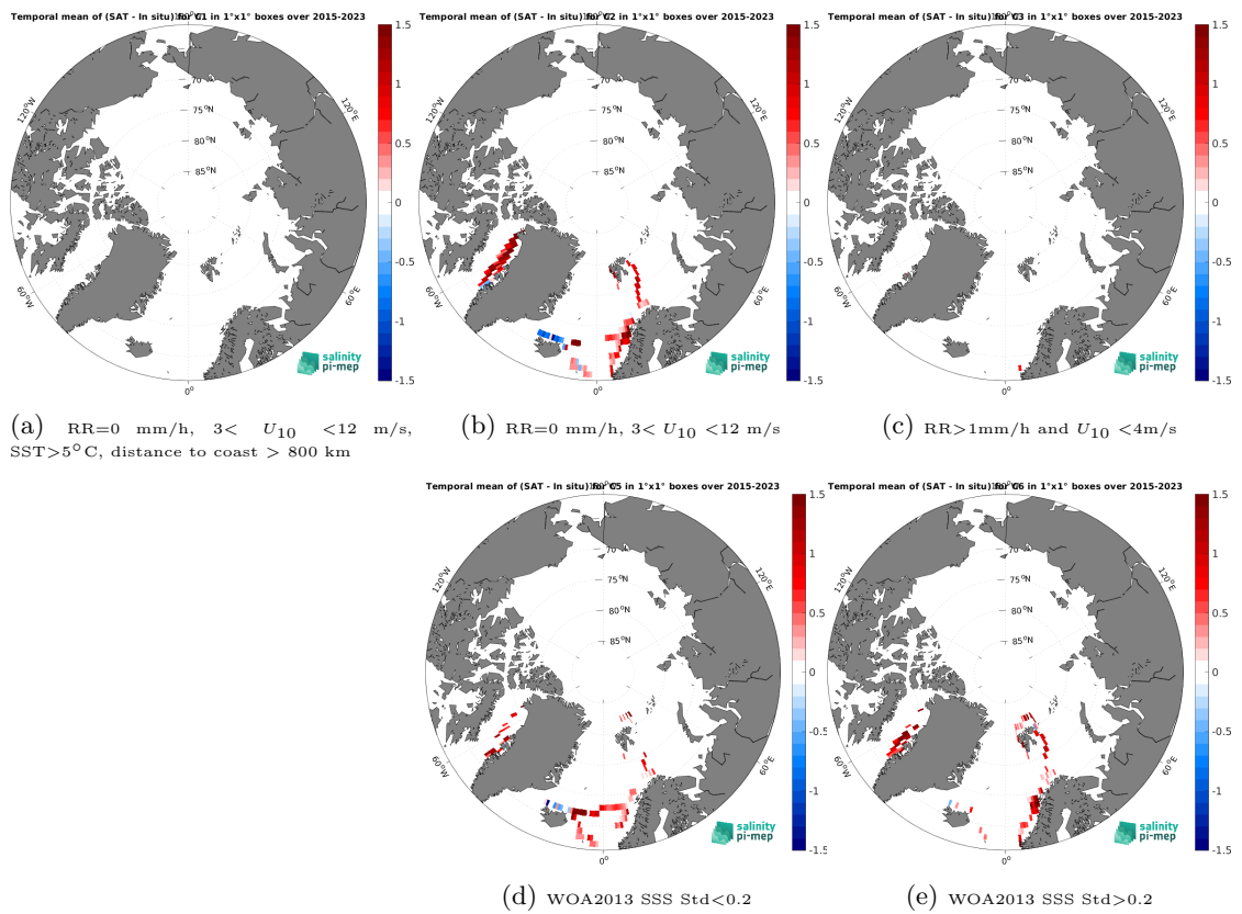
Figure 14: Temporal mean gridded over spatial boxes of size 1^\circ \times 1^\circ of \Delta SSS (SMAP SSS L3 v5.0 - Monthly (JPL) - TSG (LEGOS-DM)) for 5 different subdatasets corresponding to:RR=0 mm/h, 3 < U_{10} < 12 m/s, SST > 5°C, distance to coast > 800 km (a), RR=0 mm/h, 3 < U_{10} < 12 m/s (b), RR > 1mm/h and U_{10} < 4 m/s (c), WOA2013 SSS Std < 0.2 (d), WOA2013 SSS Std > 0.2 (e).
