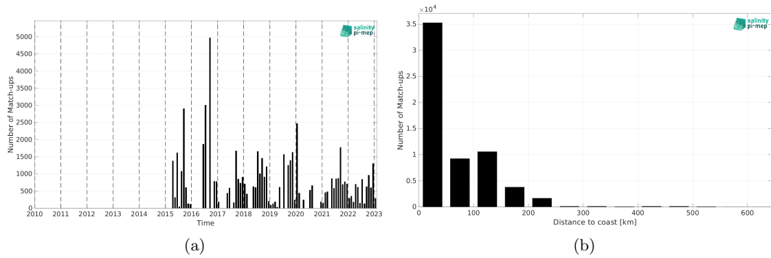
Figure 2: Number of match-ups between TSG (LEGOS-DM) and SMAP SSS L3 v5.0 - Monthly (JPL) SSS as a function of time (a) and as function of the distance to coast (b) over the Arctic Ocean Pi-MEP region and for the full satellite product period.
