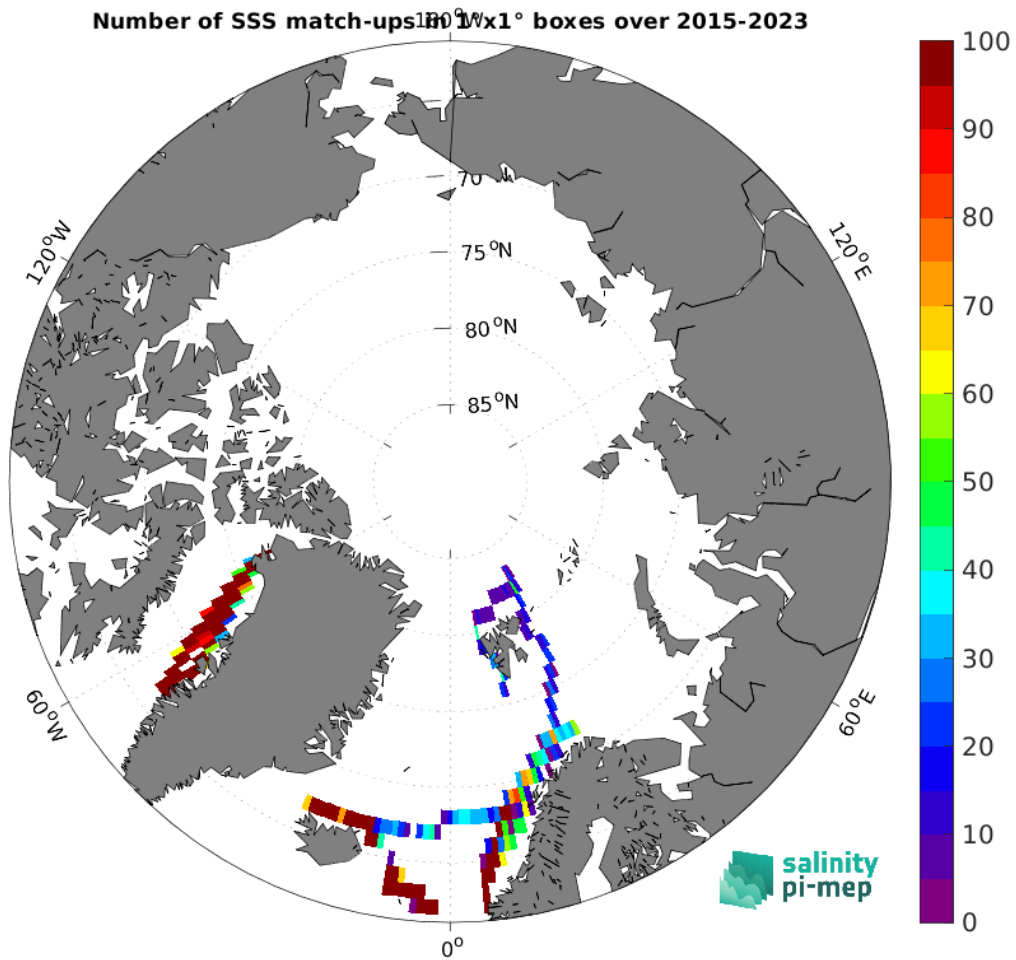
Figure 5: Number of SSS match-ups between TSG (LEGOS-DM) SSS and the SMAP SSS L3 v5.0 - Monthly (JPL) SSS product for the Arctic Ocean Pi-MEP region over 1^\circ \times 1^\circ boxes and for the full satellite product period.
