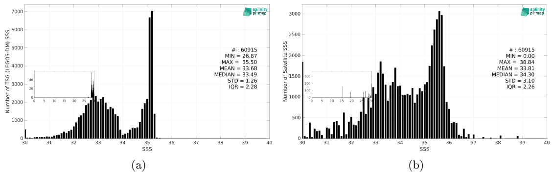
Figure 3: Histograms of SSS from TSG (LEGOS-DM) (a) and SMAP SSS L3 v5.0 - Monthly (JPL) (b) considering all match-up pairs per bins of 0.1 over the Arctic Ocean Pi-MEP region and for the full satellite product period.
