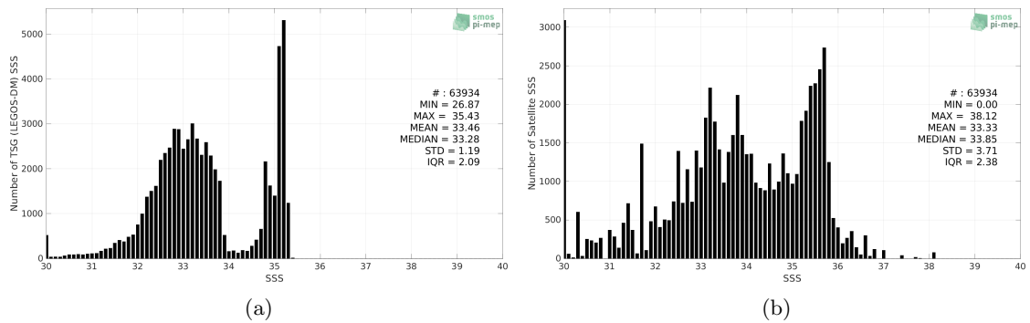
Figure 2: Histograms of SSS from TSG (LEGOS-DM) (a) and SMAP SSS L3 v5.0 - Monthly (JPL) (b) considering all match-up pairs per bins of 0.1 over the Arctic Ocean Pi-MEP region and for the full satellite product period.
