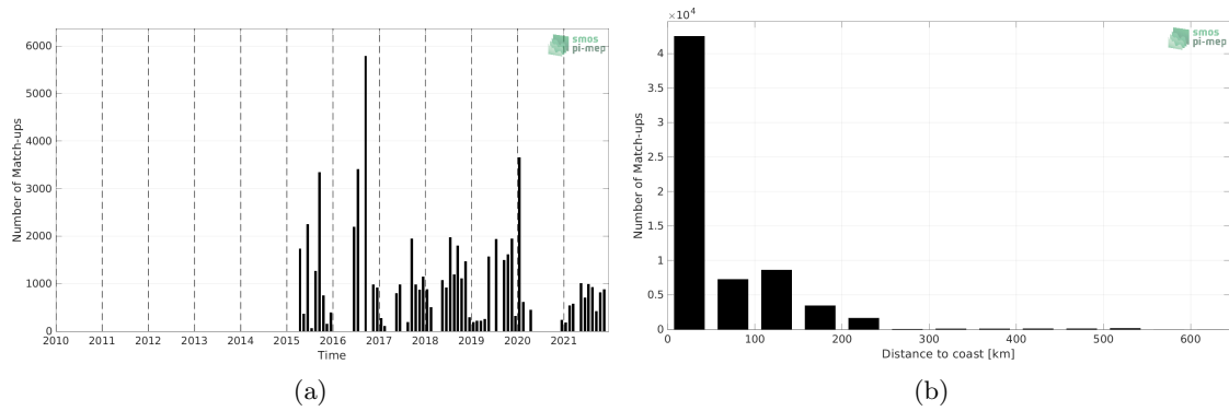
Figure 1: Number of match-ups between TSG (LEGOS-DM) and SMAP SSS L3 v5.0 - Monthly (JPL) SSS as a function of time (a) and as function of the distance to coast (b) over the Arctic Ocean Pi-MEP region and for the full satellite product period.
