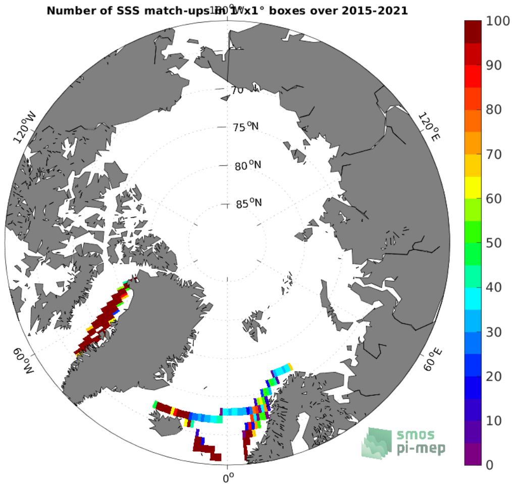
Figure 4: Number of SSS match-ups between TSG (LEGOS-DM) SSS and the SMAP SSS L3 v5.0 - Monthly (JPL) SSS product for the Arctic Ocean Pi-MEP region over 1^\circ \times 1^\circ boxes and for the full satellite product period.
