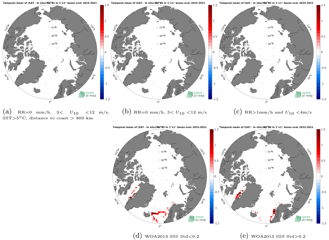
Figure 12: Temporal mean gridded over spatial boxes of size 1^{\circ}\times 1^{\circ} of \Delta\text{SSS} (SMAP SSS L3 v5.0 - Monthly (JPL) - TSG (LEGOS-DM)) for 5 different subdatasets corresponding to:RR=0 mm/h, 3 < U_{10} < 12 m/s, SST >5^{\circ}\text{C} , distance to coast > 800 km (a), RR=0 mm/h, 3 < U_{10} < 12 m/s (b), RR >1 mm/h and U_{10} < 4 m/s (c), WOA2013 SSS Std <0.2 (d), WOA2013 SSS Std >0.2 (e).
