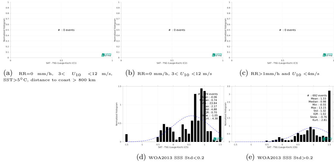
Figure 13: Normalized histogram of \Delta SSS (SMAP SSS L3 v5.0 - Monthly (JPL) - TSG (Lauge-Koch)) for 5 different subdatasets corresponding to: RR=0 mm/h, 3 < U_{10} < 12 m/s, SST>5°C, distance to coast > 800 km (a), RR=0 mm/h, 3 < U_{10} < 12 m/s (b), RR>1mm/h and U_{10} < 4 m/s (c), WOA2013 SSS Std<0.2 (d), WOA2013 SSS Std>0.2 (e).
