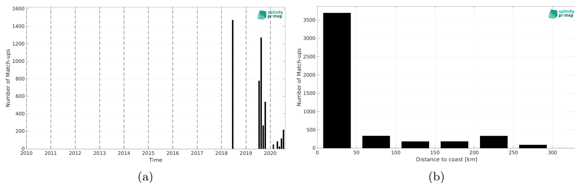
Figure 1: Number of match-ups between TSG (Lauge-Koch) and SMAP SSS L3 v5.0 - Monthly (JPL) SSS as a function of time (a) and as function of the distance to coast (b) over the Arctic Ocean Pi-MEP region and for the full satellite product period.
