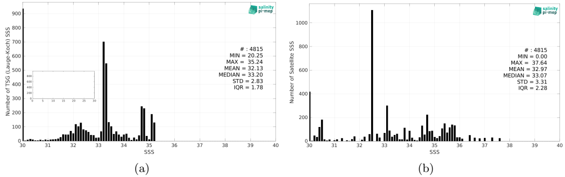
Figure 2: Histograms of SSS from TSG (Lauge-Koch) (a) and SMAP SSS L3 v5.0 - Monthly (JPL) (b) considering all match-up pairs per bins of 0.1 over the Arctic Ocean Pi-MEP region and for the full satellite product period.
