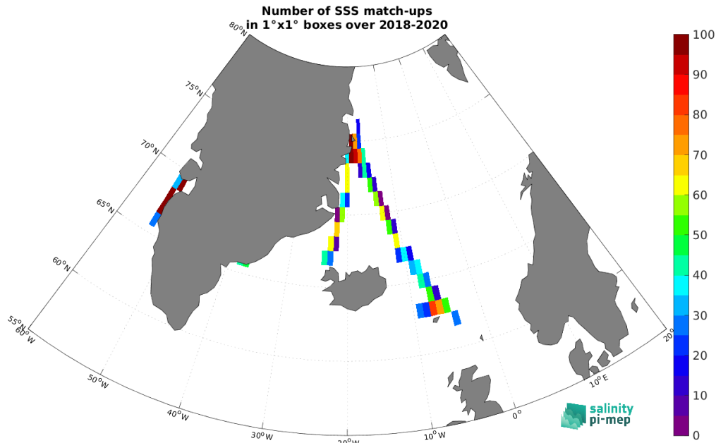
Figure 4: Number of SSS match-ups between TSG (Lauge-Koch) SSS and the SMAP SSS L3 v5.0 - Monthly (JPL) SSS product for the Arctic Ocean Pi-MEP region over 1^\circ \times 1^\circ boxes and for the full satellite product period.
