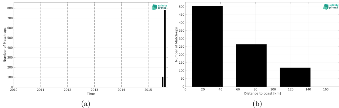
Figure 2: Number of match-ups between TSG (GOSUD-Sailing-ship) and SMAP SSS L3 v5.0 - Monthly (JPL) SSS as a function of time (a) and as function of the distance to coast (b) over the Arctic Ocean Pi-MEP region and for the full satellite product period.
