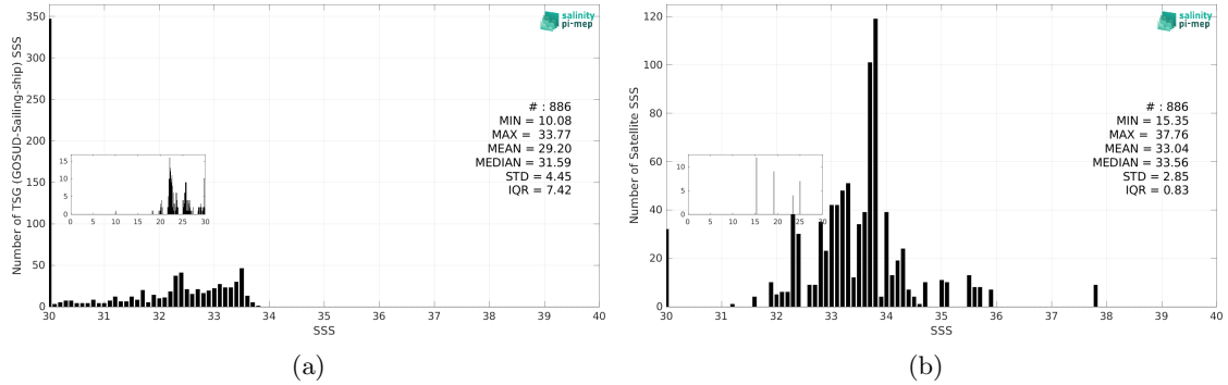
Figure 3: Histograms of SSS from TSG (GOSUD-Sailing-ship) (a) and SMAP SSS L3 v5.0 - Monthly (JPL) (b) considering all match-up pairs per bins of 0.1 over the Arctic Ocean Pi-MEP region and for the full satellite product period.
