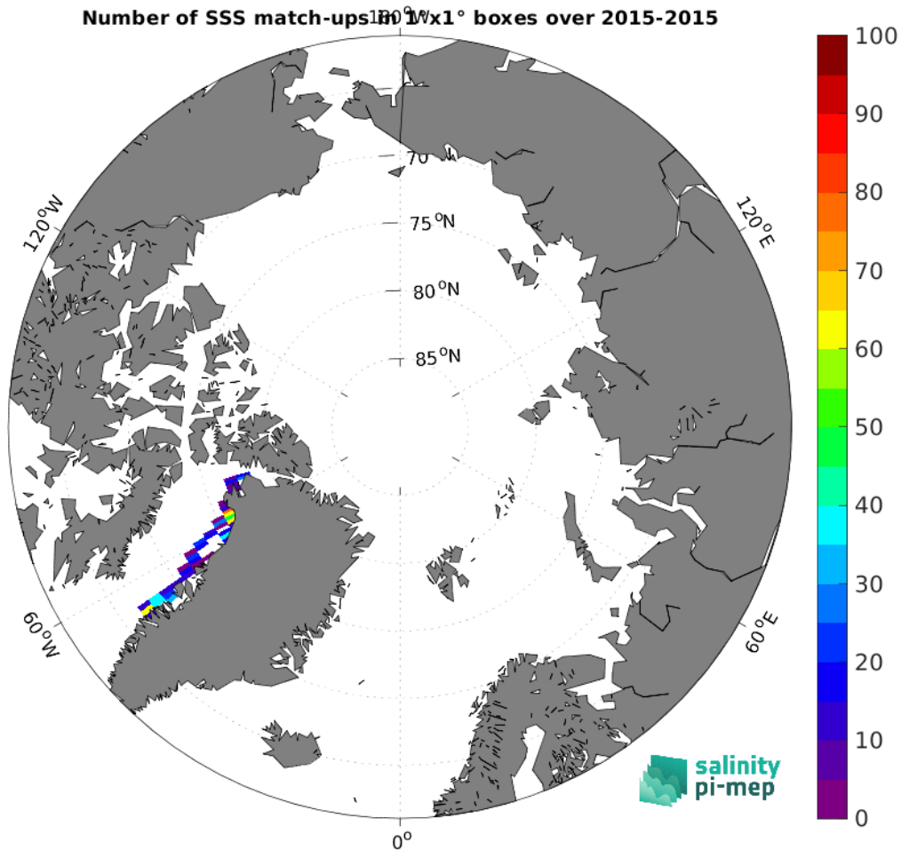
Figure 5: Number of SSS match-ups between TSG (GOSUD-Sailing-ship) SSS and the SMAP SSS L3 v5.0 - Monthly (JPL) SSS product for the Arctic Ocean Pi-MEP region over 1^\circ \times 1^\circ boxes and for the full satellite product period.
