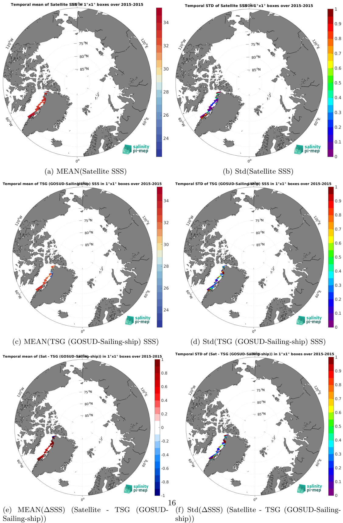
Figure 7: Temporal mean (left) and Std (right) of SSS from SMAP SSS L3 v5.0 - Monthly (JPL) (top), TSG (GOSUD-Sailing-ship) (middle), and of \Delta SSS (Satellite - TSG (GOSUD-Sailing-ship)). Only match-up pairs are used to generate these maps.
