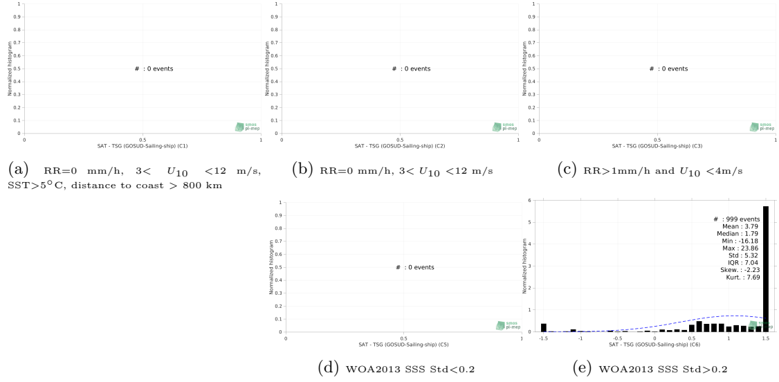
Figure 13: Normalized histogram of \Delta\text{SSS} (SMAP SSS L3 v5.0 - Monthly (JPL) - TSG (GOSUD-Sailing-ship)) for 5 different subdatasets corresponding to: RR=0 mm/h, 3 < U_{10} < 12 m/s, SST > 5^\circ\text{C} , distance to coast > 800 km (a), RR=0 mm/h, 3 < U_{10} < 12 m/s (b), RR > 1\text{mm/h} and U_{10} < 4\text{m/s} (c), WOA2013 SSS Std < 0.2 (d), WOA2013 SSS Std > 0.2 (e).
