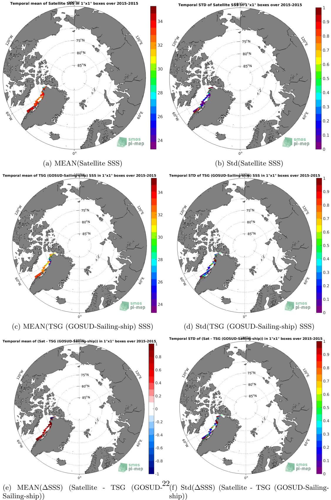
Figure 6: Temporal mean (left) and Std (right) of SSS from SMAP SSS L3 v5.0 - Monthly (JPL) (top), TSG (GOSUD-Sailing-ship) (middle), and of \Delta SSS (Satellite - TSG (GOSUD-Sailing-ship)). Only match-up pairs are used to generate these maps.
