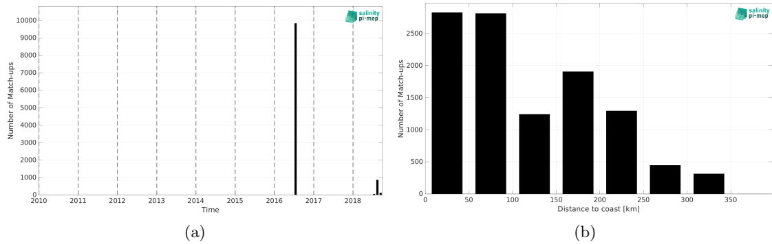
Figure 2: Number of match-ups between TSG (GOSUD-Research-vessel) and SMAP SSS L3 v5.0 - Monthly (JPL) SSS as a function of time (a) and as function of the distance to coast (b) over the Arctic Ocean Pi-MEP region and for the full satellite product period.
