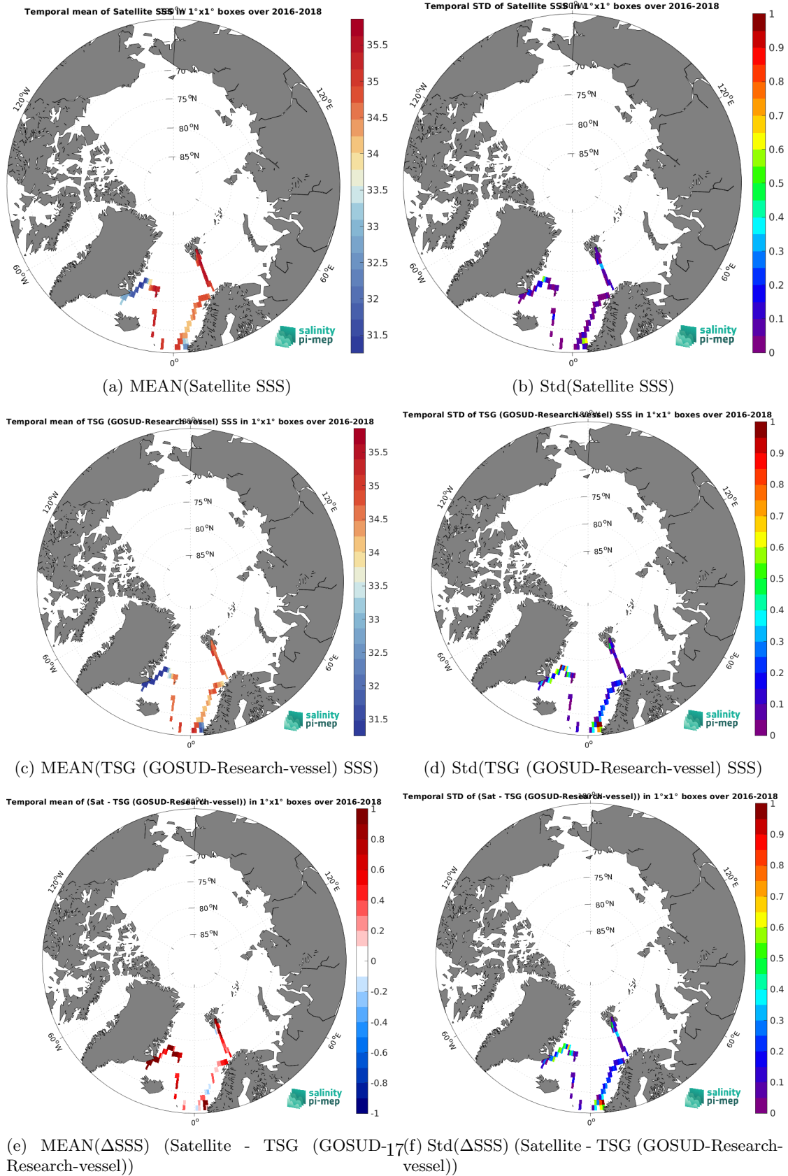
Figure 7: Temporal mean (left) and Std (right) of SSS from SMAP SSS L3 v5.0 - Monthly (JPL) (top), TSG (GOSUD-Research-vessel) (middle), and of \Delta SSS (Satellite - TSG (GOSUD-Research-vessel)). Only match-up pairs are used to generate these maps.
