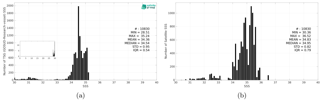
Figure 3: Histograms of SSS from TSG (GOSUD-Research-vessel) (a) and SMAP SSS L3 v5.0 - Monthly (JPL) (b) considering all match-up pairs per bins of 0.1 over the Arctic Ocean Pi-MEP region and for the full satellite product period.
