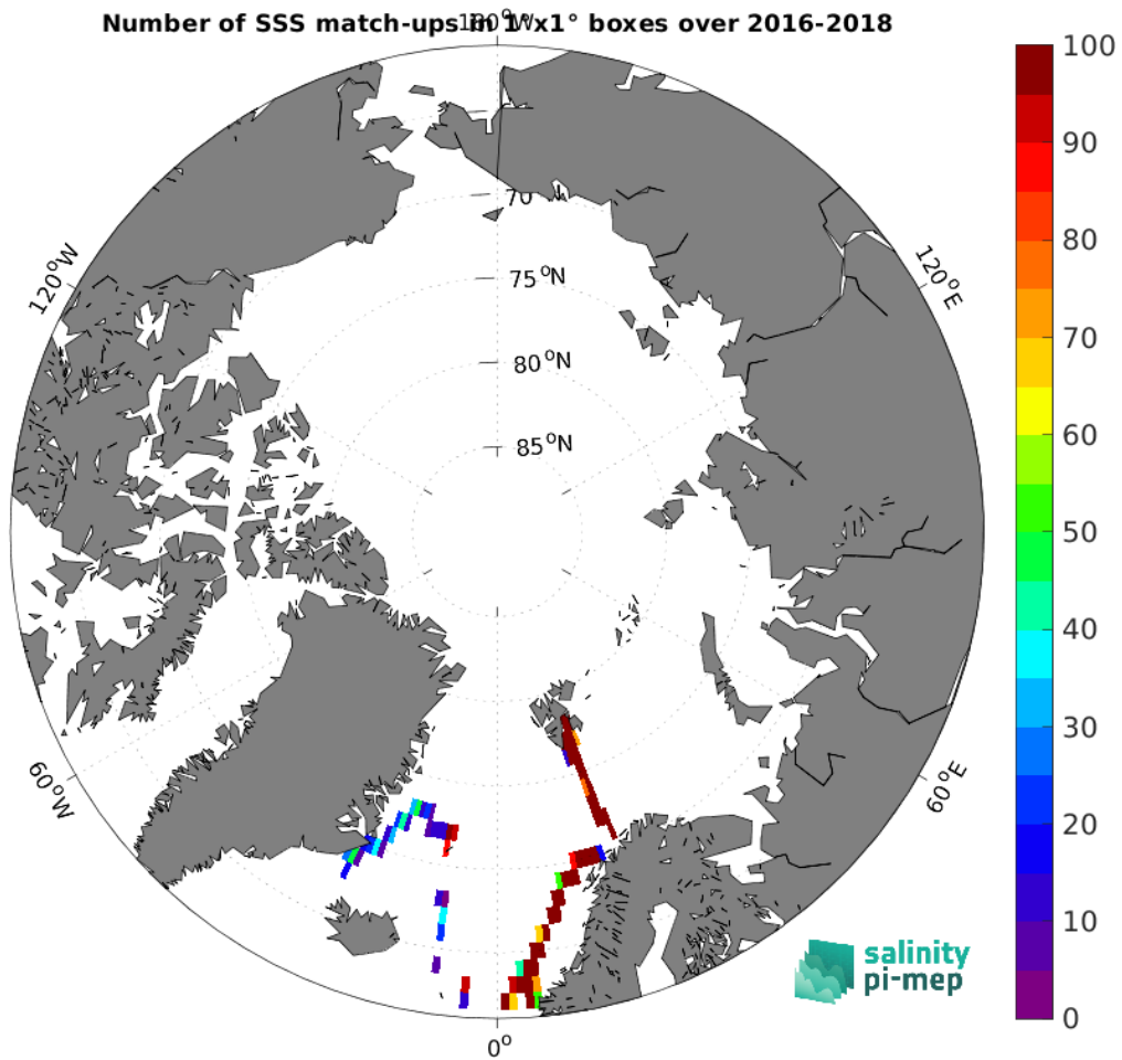
Figure 5: Number of SSS match-ups between TSG (GOSUD-Research-vessel) SSS and the SMAP SSS L3 v5.0 - Monthly (JPL) SSS product for the Arctic Ocean Pi-MEP region over 1^\circ \times 1^\circ boxes and for the full satellite product period.
