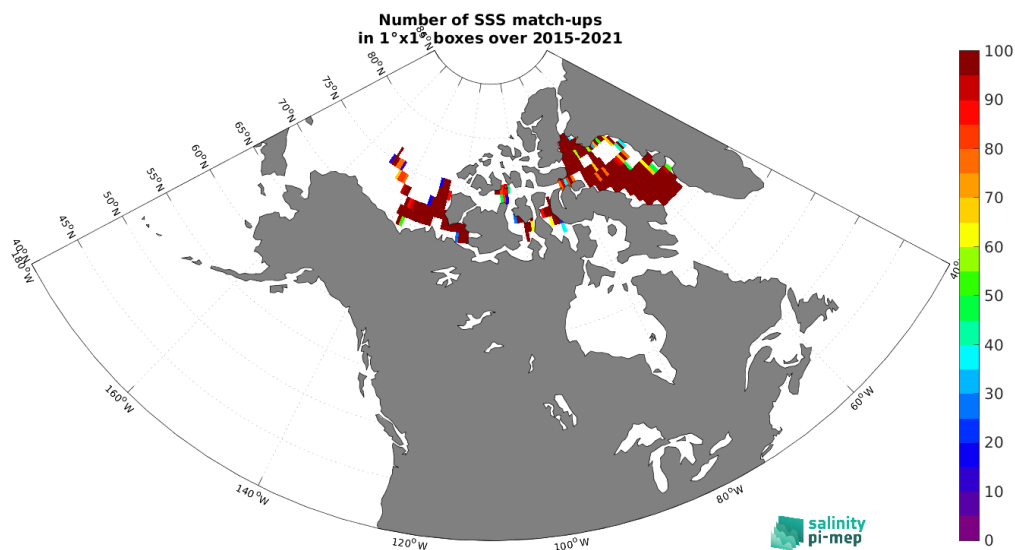
Figure 5: Number of SSS match-ups between TSG (Amundsen) SSS and the SMAP SSS L3 v5.0 - Monthly (JPL) SSS product for the Arctic Ocean Pi-MEP region over 1^\circ \times 1^\circ boxes and for the full satellite product period.
