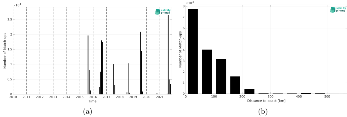
Figure 2: Number of match-ups between TSG (Amundsen) and SMAP SSS L3 v5.0 - Monthly (JPL) SSS as a function of time (a) and as function of the distance to coast (b) over the Arctic Ocean Pi-MEP region and for the full satellite product period.
