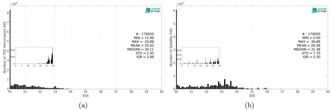
Figure 3: Histograms of SSS from TSG (Amundsen) (a) and SMAP SSS L3 v5.0 - Monthly (JPL) (b) considering all match-up pairs per bins of 0.1 over the Arctic Ocean Pi-MEP region and for the full satellite product period.
