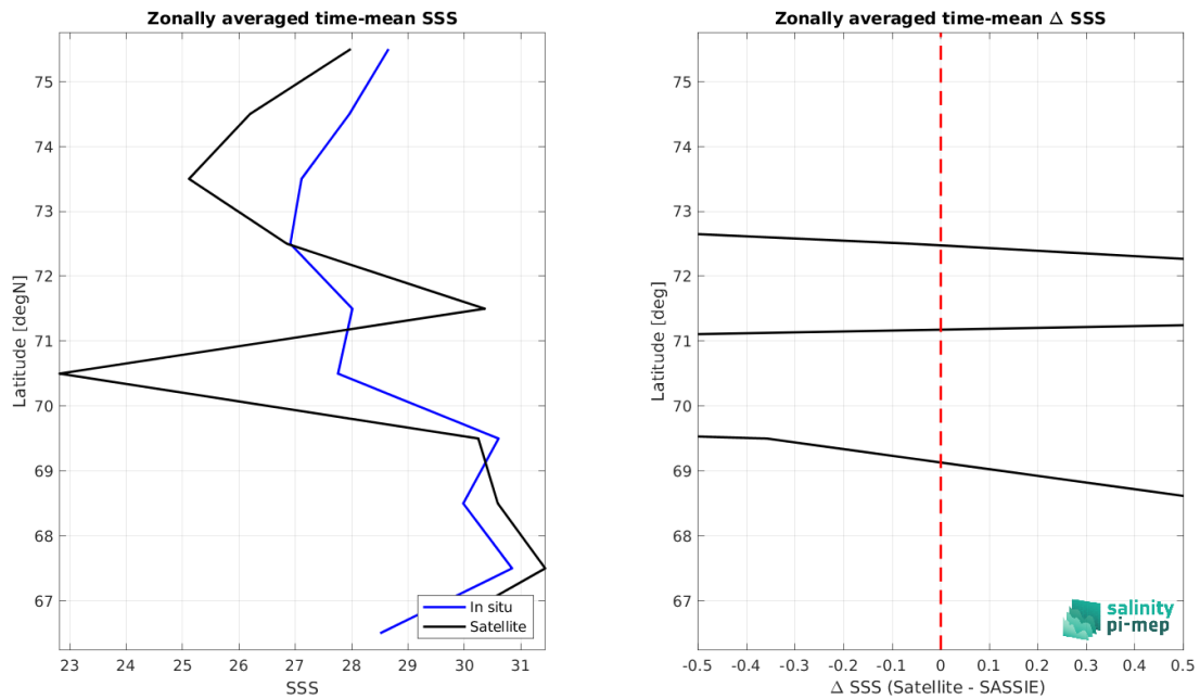
Figure 9: Left panel: Zonal mean SSS from SMAP SSS L3 v5.0 - Monthly (JPL) satellite product (black) and from SASSIE (blue). Right panel: Zonal mean of \Delta SSS (Satellite - SASSIE) for all the collected Pi-MEP match-up pairs estimated over the full satellite product period.
