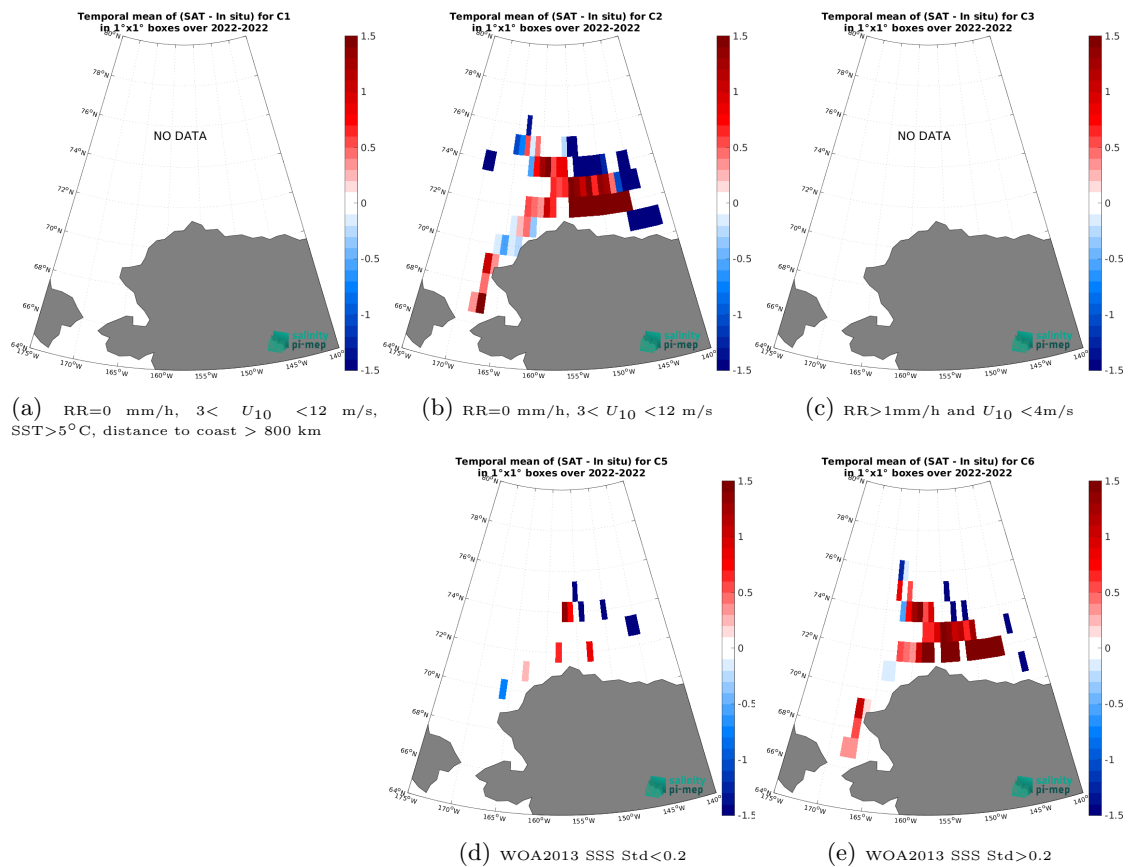
Figure 14: Temporal mean gridded over spatial boxes of size 1^\circ \times 1^\circ of \Delta\text{SSS} (SMAP SSS L3 v5.0 - Monthly (JPL) - SASSIE) for 5 different subdatasets corresponding to:RR=0 mm/h, 3 < U_{10} < 12 m/s, SST>5°C, distance to coast > 800 km (a), RR=0 mm/h, 3 < U_{10} < 12 m/s (b), RR>1mm/h and U_{10} < 4 m/s (c), WOA2013 SSS Std<0.2 (d), WOA2013 SSS Std>0.2 (e).
