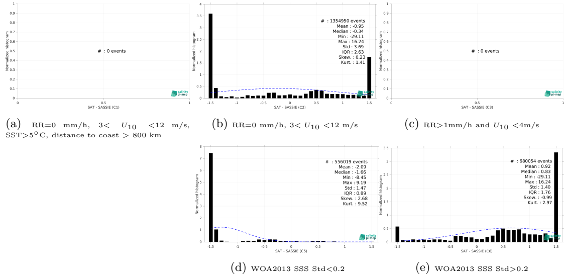
Figure 15: Normalized histogram of \Delta SSS (SMAP SSS L3 v5.0 - Monthly (JPL) - SASSIE) for 5 different subdatasets corresponding to: RR=0 mm/h, 3 < U_{10} < 12 m/s, SST > 5°C, distance to coast > 800 km (a), RR=0 mm/h, 3 < U_{10} < 12 m/s (b), RR > 1mm/h and U_{10} < 4 m/s (c), WOA2013 SSS Std < 0.2 (d), WOA2013 SSS Std > 0.2 (e).
