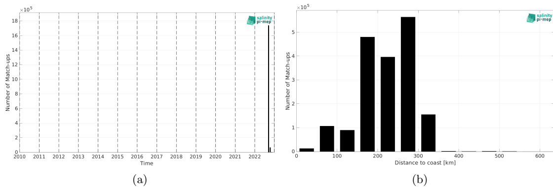
Figure 2: Number of match-ups between SASSIE and SMAP SSS L3 v5.0 - Monthly (JPL) SSS as a function of time (a) and as function of the distance to coast (b) over the Arctic Ocean Pi-MEP region and for the full satellite product period.
