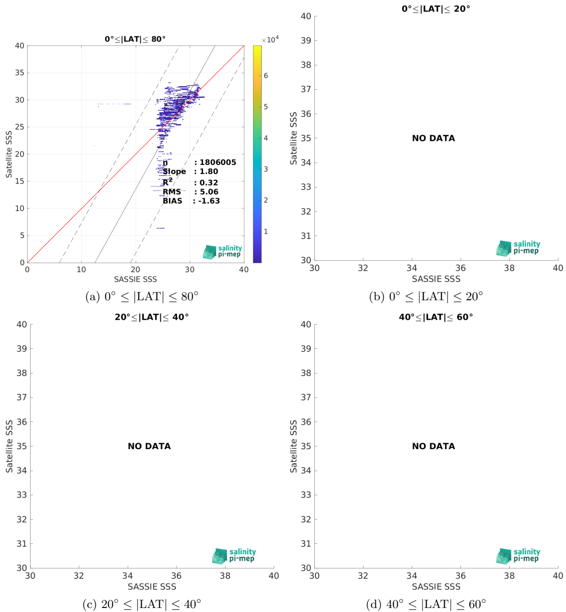
Figure 10: Contour maps of the concentration of SMAP SSS L3 v5.0 - Monthly (JPL) SSS (y-axis) versus SASSIE SSS (x-axis) at match-up pairs for different latitude bands. For each plot, the red line shows x=y . The black thin and dashed lines indicate a linear fit through the data cloud and the \pm 95\% confidence levels, respectively. The number match-up pairs n , the slope and R^2 coefficient of the linear fit, the root mean square (RMS) and the mean bias between satellite and in situ data are indicated for each latitude band in each plots.
