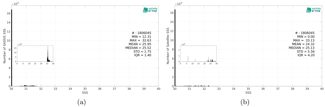
Figure 3: Histograms of SSS from SASSIE (a) and SMAP SSS L3 v5.0 - Monthly (JPL) (b) considering all match-up pairs per bins of 0.1 over the Arctic Ocean Pi-MEP region and for the full satellite product period.
