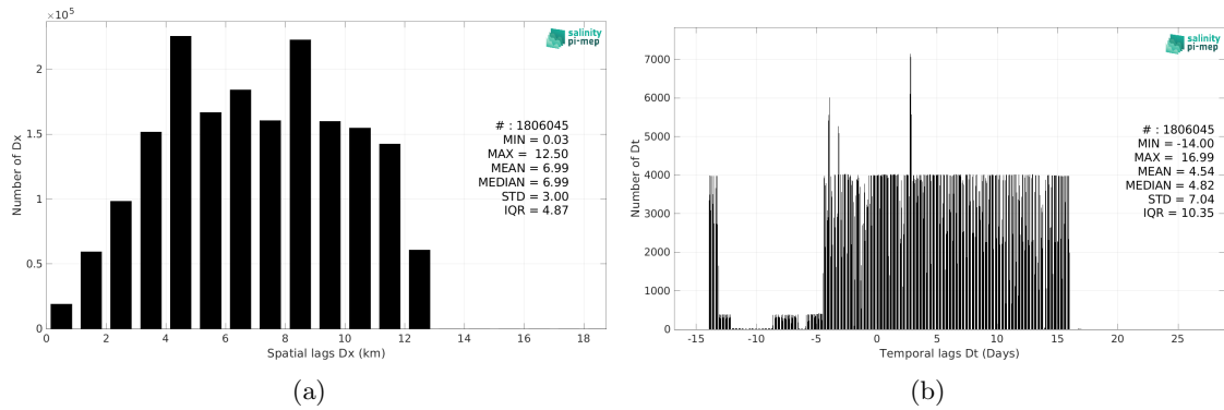
Figure 6: Histograms of the spatial (a) and temporal (b) lags between the location/time of the SASSIE measurement and the date of the corresponding SMAP SSS L3 v5.0 - Monthly (JPL) SSS pixel.
