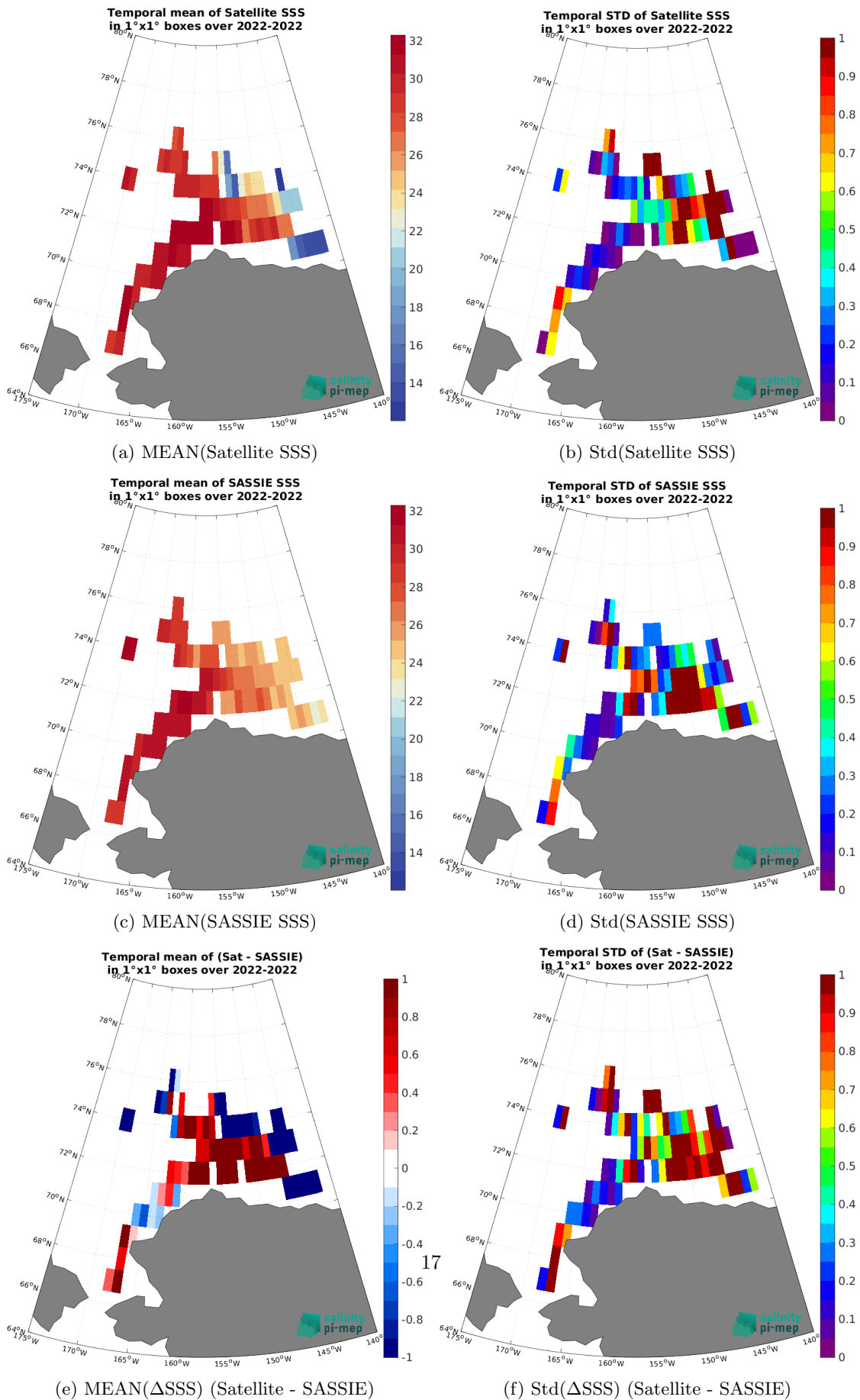
Figure 7: Temporal mean (left) and Std (right) of SSS from SMAP SSS L3 v5.0 - Monthly (JPL) (top), SASSIE (middle), and of \Delta SSS (Satellite - SASSIE). Only match-up pairs are used to generate these maps.
