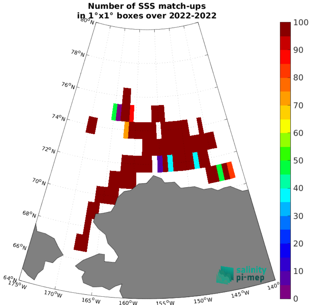
Figure 5: Number of SSS match-ups between SASSIE SSS and the SMAP SSS L3 v5.0 - Monthly (JPL) SSS product for the Arctic Ocean Pi-MEP region over 1^\circ \times 1^\circ boxes and for the full satellite product period.
