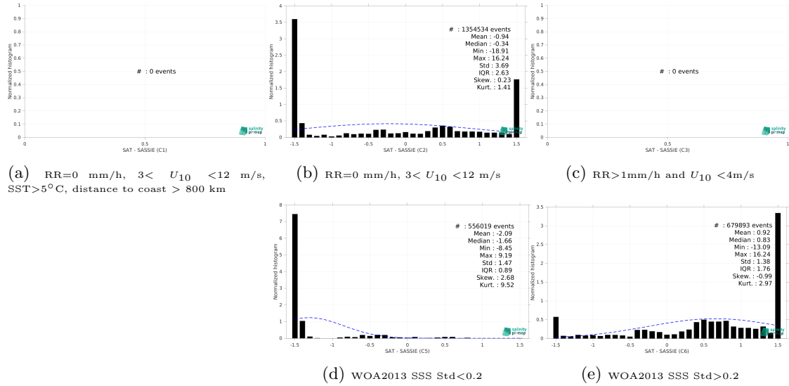
Figure 15: Normalized histogram of \Delta\text{SSS} (SMAP SSS L3 v5.0 - Monthly (JPL) - SASSIE) for 5 different subdatasets corresponding to: RR=0 mm/h, 3 < U_{10} < 12 m/s, SST>5°C, distance to coast > 800 km (a), RR=0 mm/h, 3 < U_{10} < 12 m/s (b), RR>1mm/h and U_{10} < 4 m/s (c), WOA2013 SSS Std<0.2 (d), WOA2013 SSS Std>0.2 (e).
