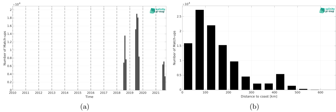
Figure 2: Number of match-ups between Sairdrone and SMAP SSS L3 v5.0 - Monthly (JPL) SSS as a function of time (a) and as function of the distance to coast (b) over the Arctic Ocean Pi-MEP region and for the full satellite product period.
