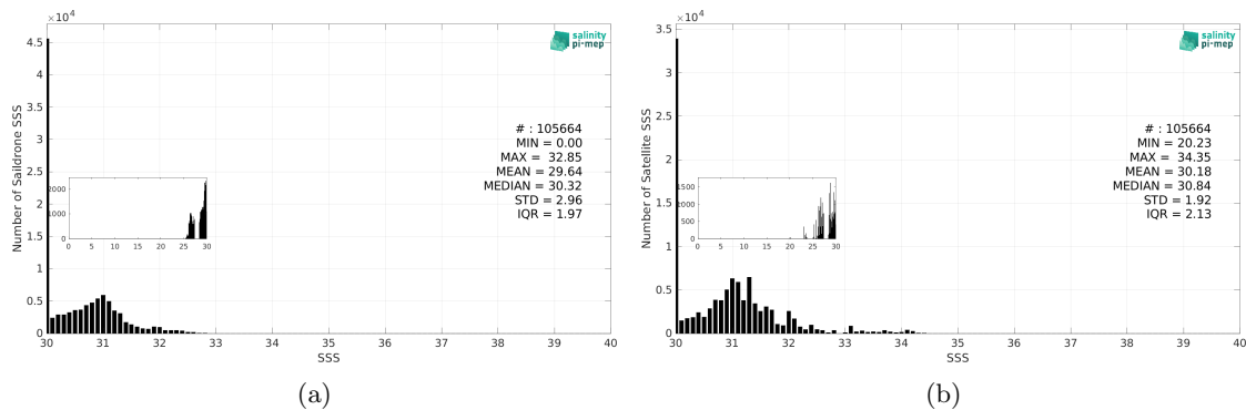
Figure 3: Histograms of SSS from Sairdrone (a) and SMAP SSS L3 v5.0 - Monthly (JPL) (b) considering all match-up pairs per bins of 0.1 over the Arctic Ocean Pi-MEP region and for the full satellite product period.
