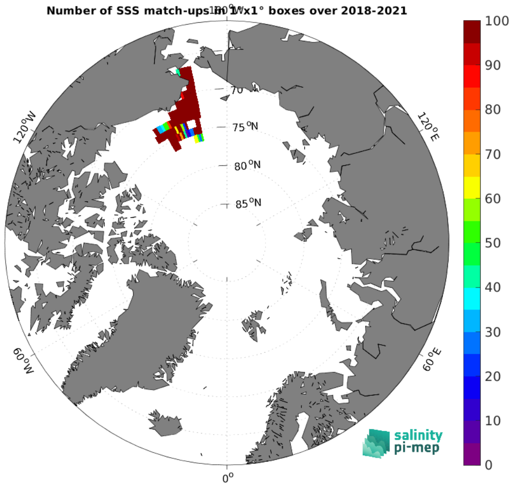
Figure 5: Number of SSS match-ups between Sailldrone SSS and the SMAP SSS L3 v5.0 - Monthly (JPL) SSS product for the Arctic Ocean Pi-MEP region over 1^\circ \times 1^\circ boxes and for the full satellite product period.
