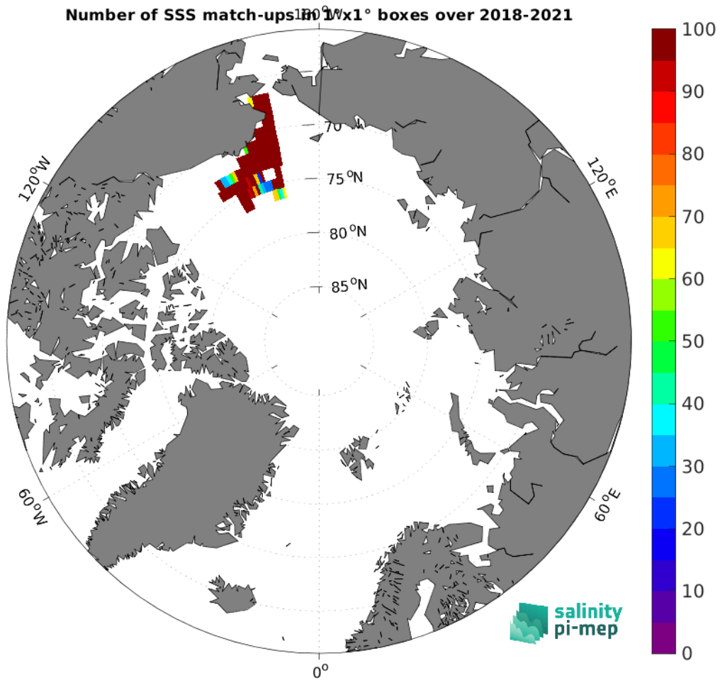
Figure 4: Number of SSS match-ups between Sailldrone SSS and the SMAP SSS L3 v5.0 - Monthly (JPL) SSS product for the Arctic Ocean Pi-MEP region over 1^\circ \times 1^\circ boxes and for the full satellite product period.
