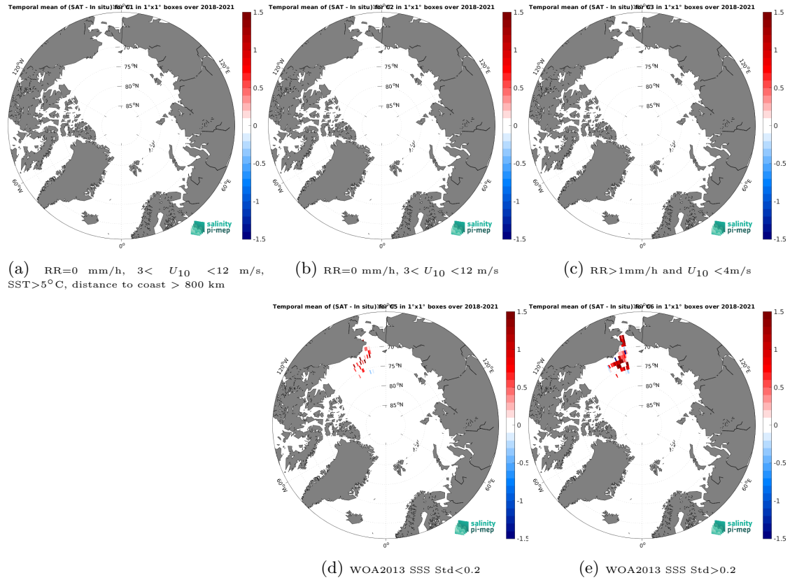
Figure 12: Temporal mean gridded over spatial boxes of size 1^{\circ}\times 1^{\circ} of \Delta\text{SSS} (SMAP SSS L3 v5.0 - Monthly (JPL) - Sairdrone) for 5 different subdatasets corresponding to:RR=0 mm/h, 3 < U_{10} < 12 m/s, SST >5^{\circ}\text{C} , distance to coast > 800 km (a), RR=0 mm/h, 3 < U_{10} < 12 m/s (b), RR >1 mm/h and U_{10} < 4 m/s (c), WOA2013 SSS Std <0.2 (d), WOA2013 SSS Std >0.2 (e).
