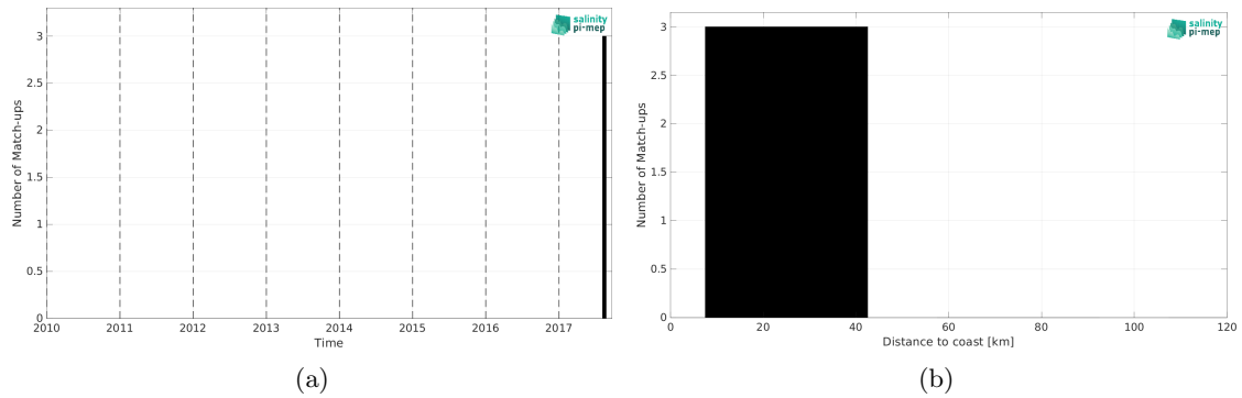
Figure 1: Number of match-ups between Marine mammals and SMAP SSS L3 v5.0 - Monthly (JPL) SSS as a function of time (a) and as function of the distance to coast (b) over the Arctic Ocean Pi-MEP region and for the full satellite product period.
