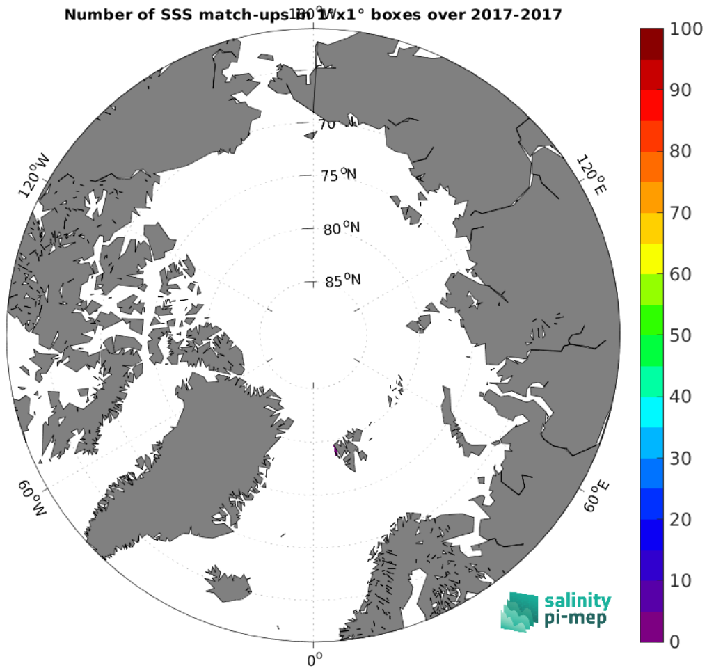
Figure 4: Number of SSS match-ups between Marine mammals SSS and the SMAP SSS L3 v5.0 - Monthly (JPL) SSS product for the Arctic Ocean Pi-MEP region over 1^\circ \times 1^\circ boxes and for the full satellite product period.
