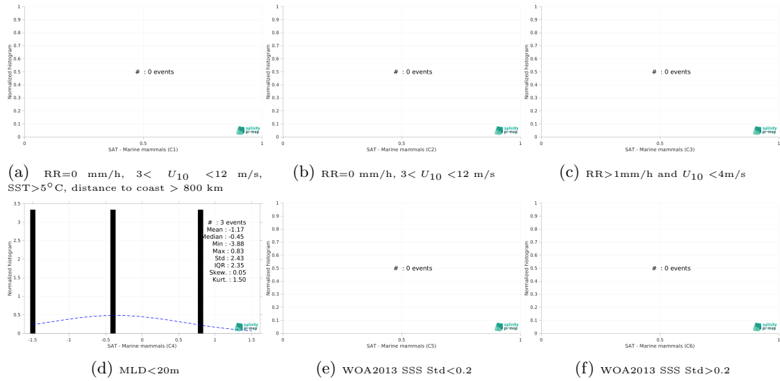
Figure 13: Normalized histogram of \Delta\text{SSS} (SMAP SSS L3 v5.0 - Monthly (JPL) - Marine mammals) for 6 different subdatasets corresponding to: RR=0 mm/h, 3 < U_{10} < 12 m/s, SST > 5^\circ\text{C} , distance to coast > 800 km (a), RR=0 mm/h, 3 < U_{10} < 12 m/s (b), RR > 1 mm/h and U_{10} < 4 m/s (c), MLD < 20 m (d), WOA2013 SSS Std < 0.2 (e), WOA2013 SSS Std > 0.2 (f).
