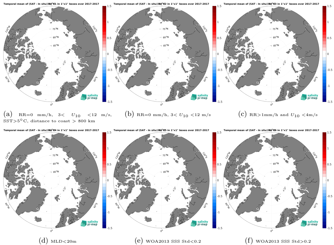
Figure 12: Temporal mean gridded over spatial boxes of size 1^{\circ}\times 1^{\circ} of \Delta\text{SSS} (SMAP SSS L3 v5.0 - Monthly (JPL) - Marine mammals) for 6 different subdatasets corresponding to:RR=0 mm/h, 3 < U_{10} < 12 m/s, SST >5^{\circ}\text{C} , distance to coast > 800 km (a), RR=0 mm/h, 3 < U_{10} < 12 m/s (b), RR >1 mm/h and U_{10} < 4 m/s (c),MLD <20 m (d),WOA2013 SSS Std <0.2 (e),WOA2013 SSS Std >0.2 (f).
