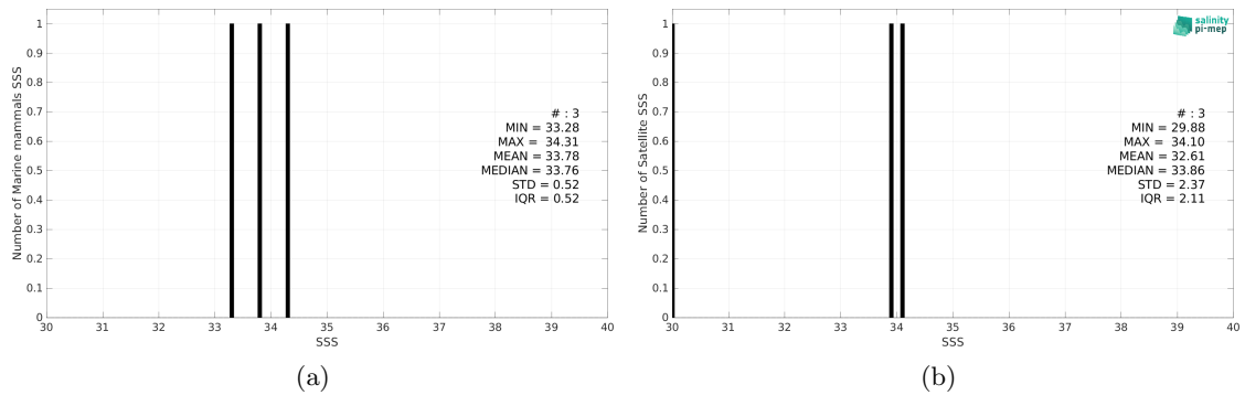
Figure 2: Histograms of SSS from Marine mammals (a) and SMAP SSS L3 v5.0 - Monthly (JPL) (b) considering all match-up pairs per bins of 0.1 over the Arctic Ocean Pi-MEP region and for the full satellite product period.
