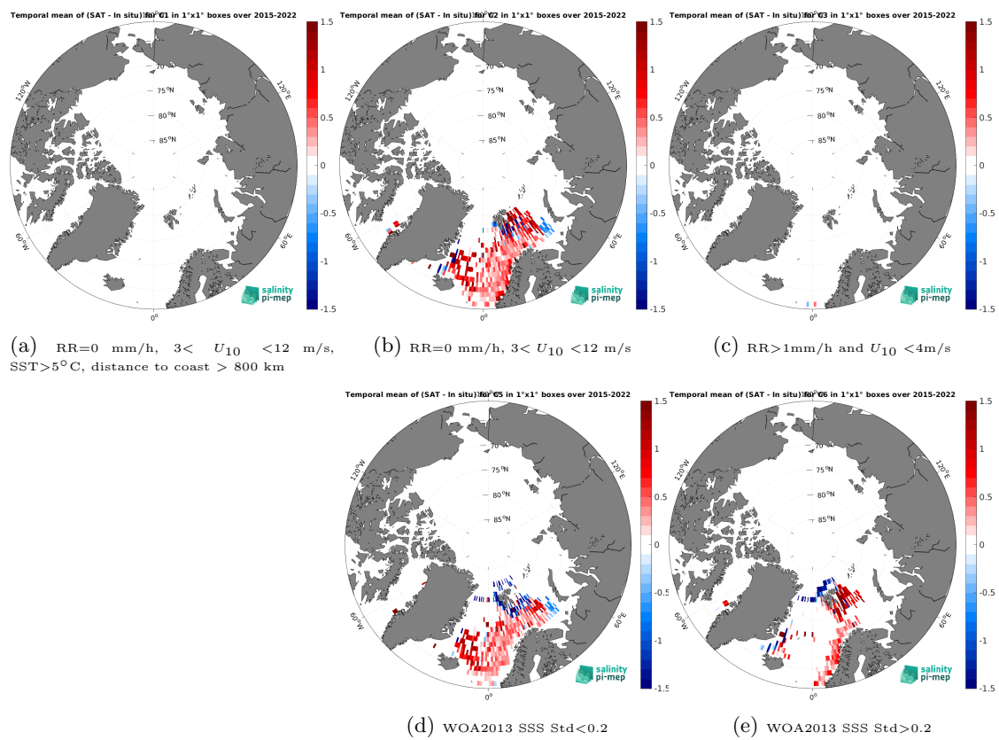
Figure 14: Temporal mean gridded over spatial boxes of size 1^\circ \times 1^\circ of \Delta\text{SSS} (SMAP SSS L3 v5.0 - Monthly (JPL) - ICES) for 5 different subdatasets corresponding to:RR=0 mm/h, 3 < U_{10} < 12 m/s, SST>5°C, distance to coast > 800 km (a), RR=0 mm/h, 3 < U_{10} < 12 m/s (b), RR>1mm/h and U_{10} < 4 m/s (c), WOA2013 SSS Std<0.2 (d), WOA2013 SSS Std>0.2 (e).
