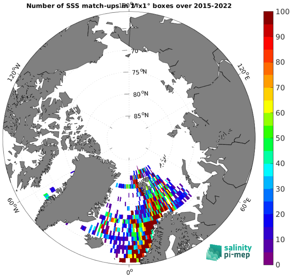
Figure 5: Number of SSS match-ups between ICES SSS and the SMAP SSS L3 v5.0 - Monthly (JPL) SSS product for the Arctic Ocean Pi-MEP region over 1^\circ \times 1^\circ boxes and for the full satellite product period.
