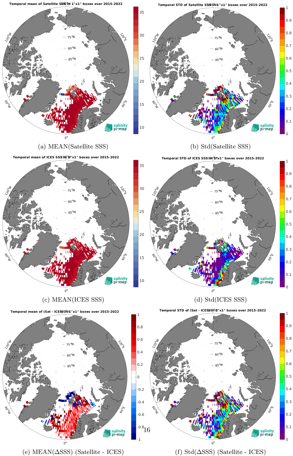
Figure 7: Temporal mean (left) and Std (right) of SSS from SMAP SSS L3 v5.0 - Monthly (JPL) (top), ICES (middle), and of \Delta SSS (Satellite - ICES). Only match-up pairs are used to generate these maps.
