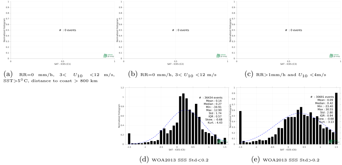
Figure 13: Normalized histogram of \Delta SSS (SMAP SSS L3 v5.0 - Monthly (JPL) - ICES) for 5 different subdatasets corresponding to: RR=0 mm/h, 3 < U_{10} < 12 m/s, SST > 5°C, distance to coast > 800 km (a), RR=0 mm/h, 3 < U_{10} < 12 m/s (b), RR > 1mm/h and U_{10} < 4 m/s (c), WOA2013 SSS Std < 0.2 (d), WOA2013 SSS Std > 0.2 (e).
