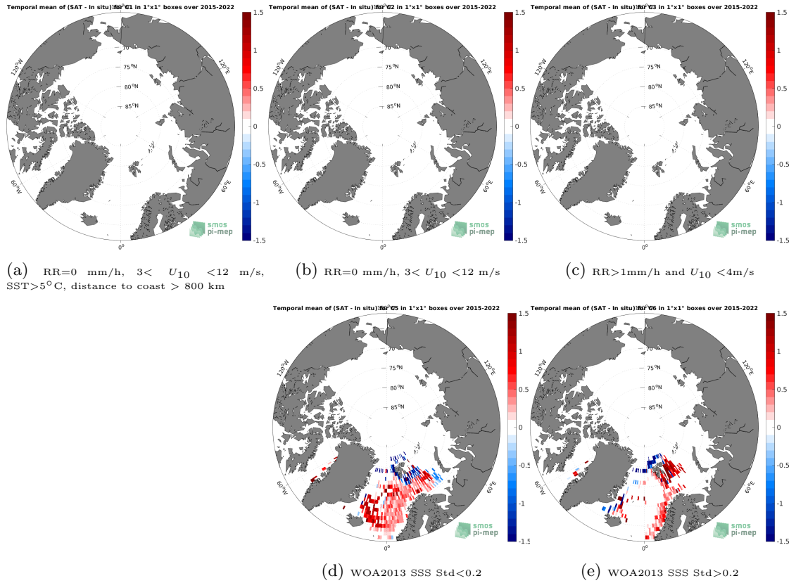
Figure 12: Temporal mean gridded over spatial boxes of size 1^{\circ}\times 1^{\circ} of \Delta\text{SSS} (SMAP SSS L3 v5.0 - Monthly (JPL) - ICES) for 5 different subdatasets corresponding to:RR=0 mm/h, 3 < U_{10} < 12 m/s, SST > 5^{\circ}\text{C} , distance to coast > 800 km (a), RR=0 mm/h, 3 < U_{10} < 12 m/s (b), RR > 1 mm/h and U_{10} < 4 m/s (c), WOA2013 SSS Std < 0.2 (d), WOA2013 SSS Std > 0.2 (e).
