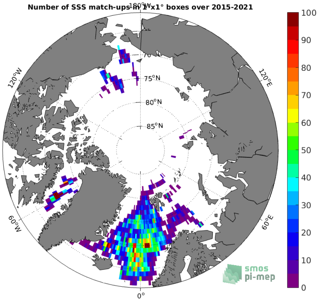
Figure 4: Number of SSS match-ups between Argo SSS and the SMAP SSS L3 v5.0 - Monthly (JPL) SSS product for the Arctic Ocean Pi-MEP region over 1^\circ \times 1^\circ boxes and for the full satellite product period.
