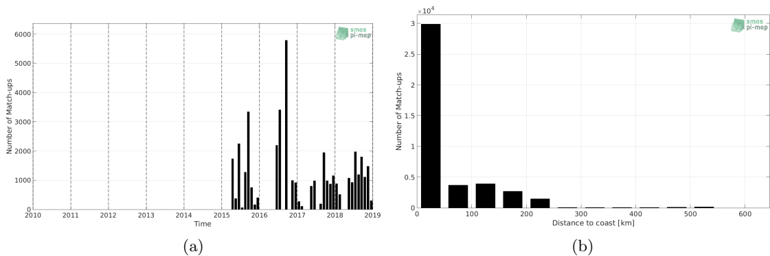
Figure 1: Number of match-ups between TSG-LEGOS-DM and SMAP-L3-JPL-V4.3-MONTHLY-60KM SSS as a function of time (a) and as function of the distance to coast (b) over the Arctic Ocean Pi-MEP region and for the full satellite product period.
