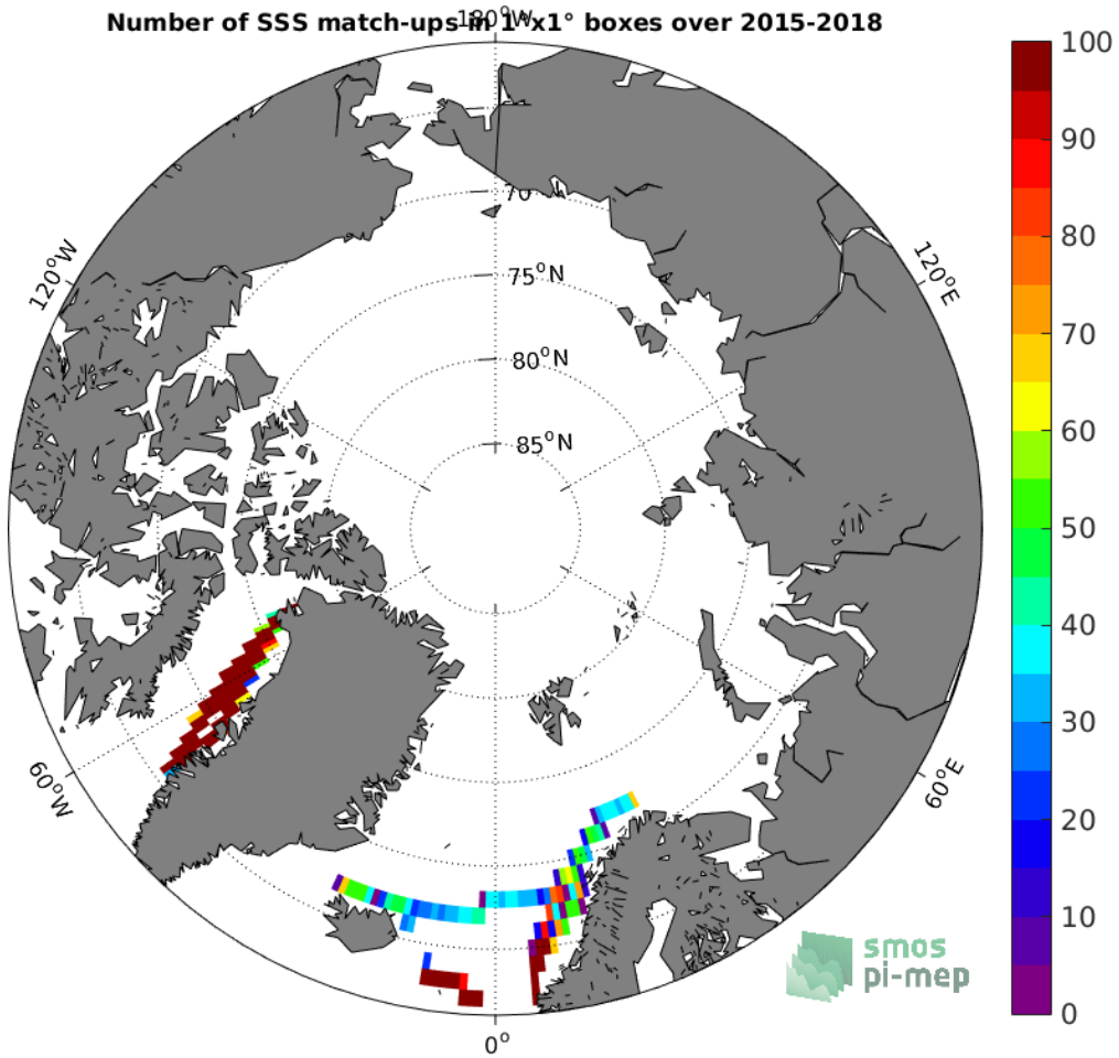
Figure 4: Number of SSS match-ups between TSG-LEGOS-DM SSS and the SMAP-L3-JPL-V4.3-MONTHLY-60KM SSS product for the Arctic Ocean Pi-MEP region over 1^{\circ} \times 1^{\circ} boxes and for the full satellite product period.
