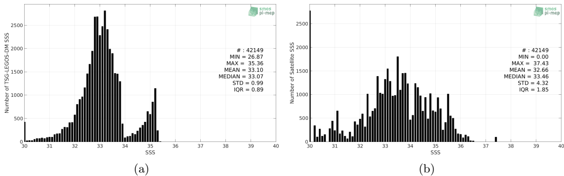
Figure 2: Histograms of SSS from TSG-LEGOS-DM (a) and SMAP-L3-JPL-V4.3-MONTHLY-60KM (b) considering all match-up pairs per bins of 0.1 over the Arctic Ocean Pi-MEP region and for the full satellite product period.
